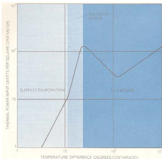
THREE STAGES OF VAPORIZATION are apparent on this graph, which shows the temperature difference between the outside surface of a container and the surface of a pool of liquid boiling inside the container as a function of the input power density. In the first stage (surface evaporation) the input heat is just enough to cause evaporation of the liquid at its surface. In the second stage (nucleate boiling) vapor bubbles form within the body of the fluid and rise to the surface. (There is strong evidence that nucleate boiling does not take place in a heat pipe.) In the third stage (film boiling) the individual bubbles tend to form a film that covers all or large portions of the surface. (The initial downward part of the curve corresponds to partial film boiling.) The onset of the film-boiling stage represents a critical input power density that cannot be exceeded without damaging the container.
