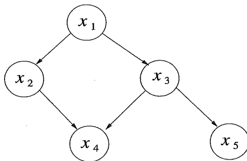
Figure 2.8 An example of a Bayesian network.
