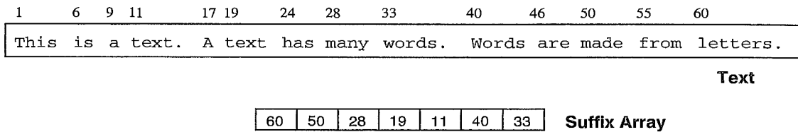
Figure 8.7 The suffix array for the sample text.
