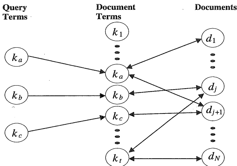
Figure 2.7 A neural network model for information retrieval.
