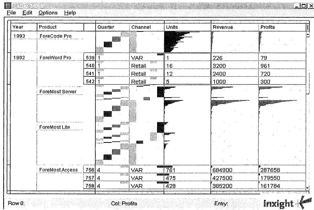
Figure 10.24 The TableLens visualization [666].
