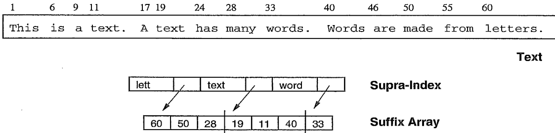
Figure 8.8 A supra-index over our suffix array. One out of three entries are sampled, keeping their first four characters. The pointers (arrows) are in fact unnecessary.
