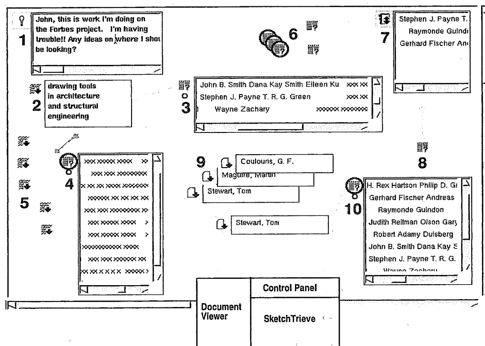
Figure 10.30 The SketchTrieve interface [365].
