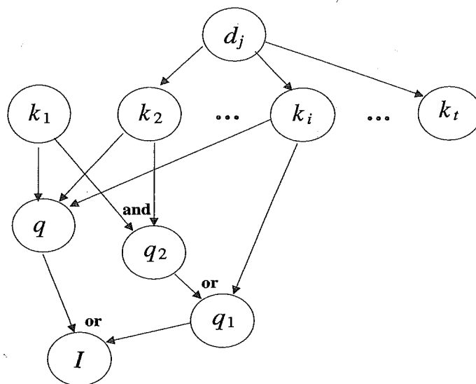
Figure 2.9 Basic inference network model.
