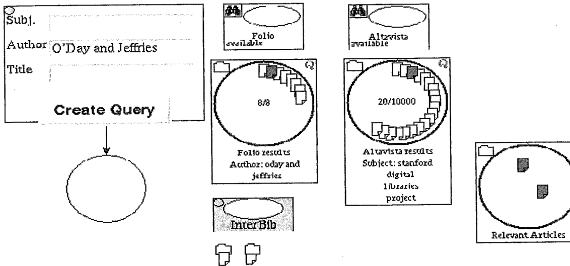
Figure 10.29 The DLITE interface [193].
