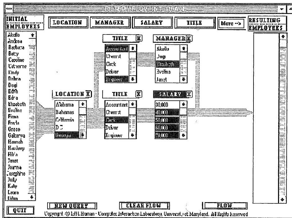
Figure 10.11 The filter-flow visualization for Boolean query specification [841].
