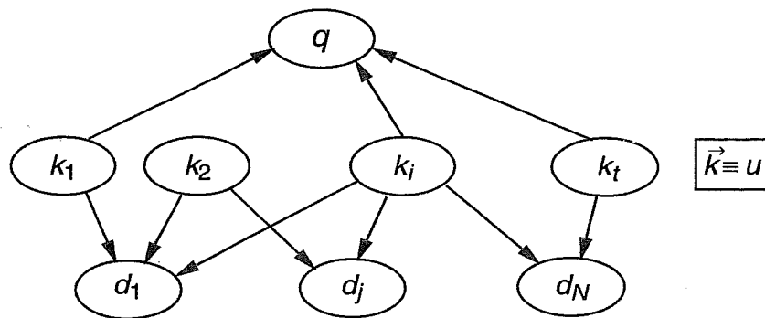
Figure 2.10 Basic belief network model.
