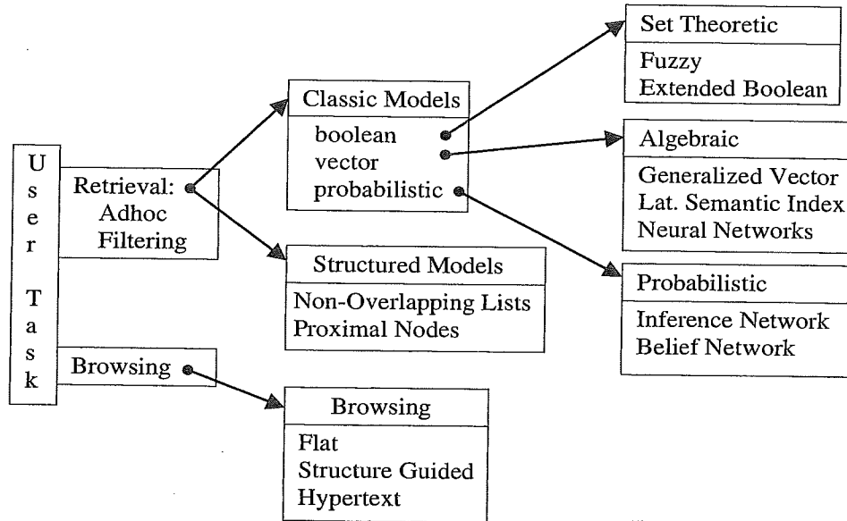
Figure 2.1 A taxonomy of information retrieval models.
