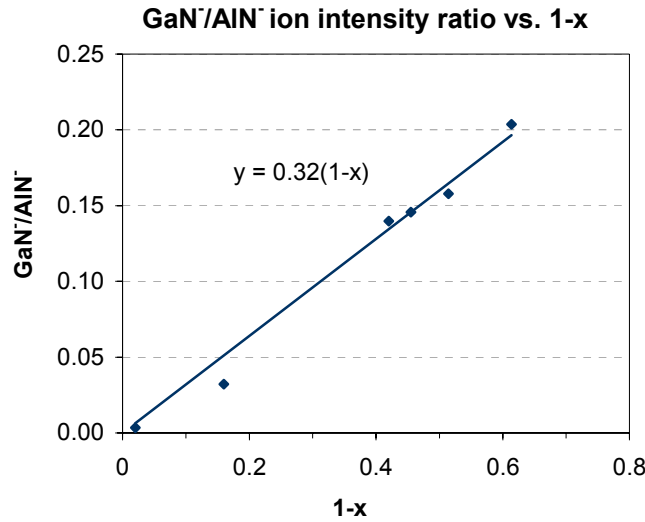
Figure 5-3. Inverse plot of figure 5-3: Matrix ion intensity ratio \text{GaN}^-/\text{AlN}^- ratio as a function of GaN mole fraction (1-x) in \text{Al}_x\text{Ga}_{1-x}\text{N} at 14.5 keV impact energy
