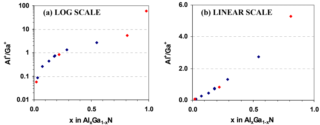
Figure 4-5. Matrix ion intensity ratio \text{Al}^+/\text{Ga}^+ ratio as a function of AlN mole fraction ( x ) with wide range of x ( 0 \leq x < 1 ) with \text{O}_2^+ ion impact energy 5.5 keV; the left figure is in log scale, the right one is in linear scale. The red data points are data from ion implantation fabricated samples.
