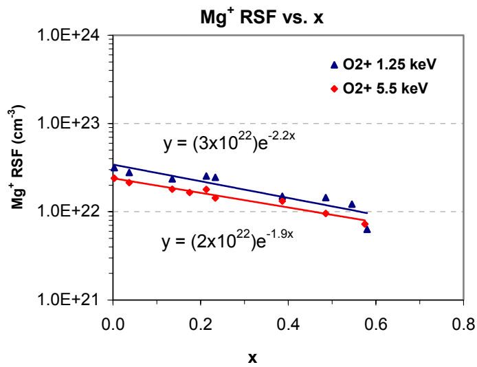
Figure 4-9. \text{Mg}^+ RSF (normalized to \text{Ga}^+ ) as a function of AlN mole fraction ( x ) at high and low impact energies
