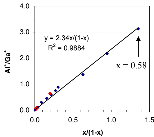
Figure 4-6. Matrix ion intensity ratio \text{Al}^+/\text{Ga}^+ ratio as a function of AlN and GaN mole fraction ratio x/(1-x) ; The red points are data from ion implantation fabricated samples.
