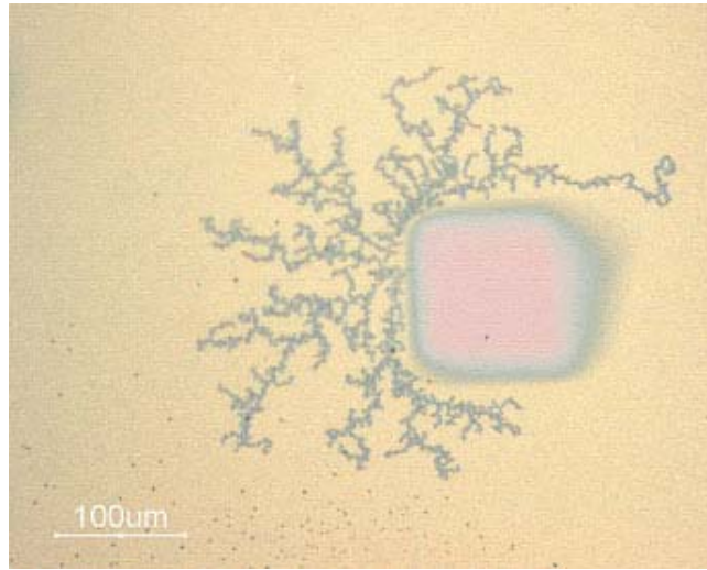
Figure 2-10. Optical image shows severe sample damages from charging. Sample is 1.36μm SiO 2 under 14.5 keV impact energy of Cs + bombardment.
