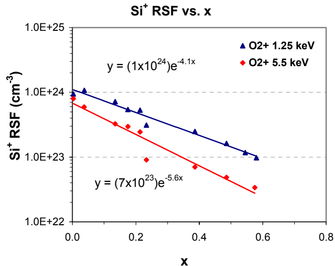
Figure 4-10. \text{Si}^+ RSF (normalized to \text{Ga}^+ ) as a function of AlN mole fraction ( x ) at high and low impact energies
