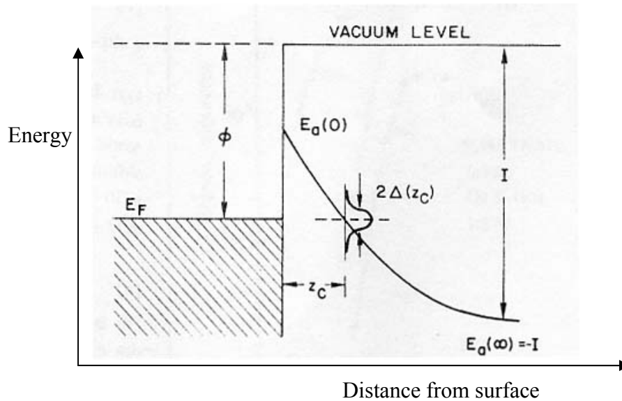
Figure 2-4. Schematic drawing of energy diagram of an atom leaving a metal surface. Z_c is the crossing distance when E_a = E_F which is in the order of several bond lengths away from surface. (Adapted from reference 20)
