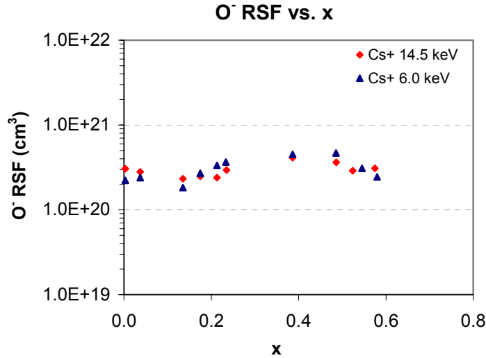
Figure 5-6. \text{O}^- RSF (normalized to \text{GaN}^- ) as a function of AlN mole fraction ( x ) in \text{Al}_x\text{Ga}_{1-x}\text{N} at 14.5 keV and 6.0 keV impact energies
