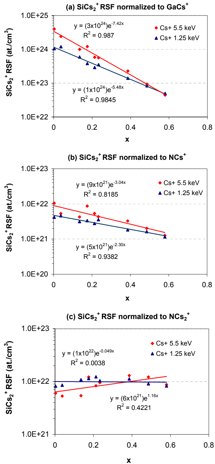
Figure 6-10. \text{SiCs}_2^+ RSF as a function of AlN mole fraction ( x ) at high and low impact energies. Figure (a) is \text{SiCs}_2^+ RSF normalized to \text{GaCs}^+ , (b) to \text{NCs}^+ and (c) to \text{NCs}_2^+ .
