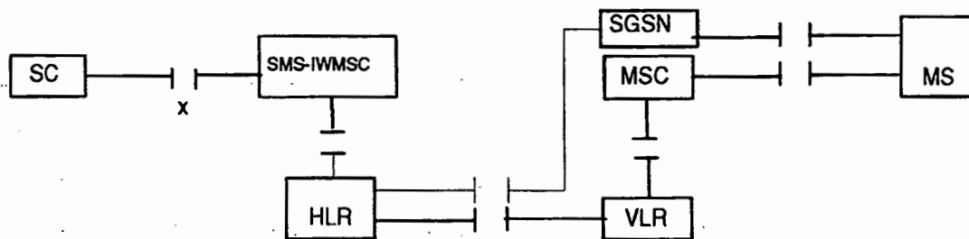
Figure 19: Interfaces involved in the Alert procedure. X is the interface between an SC and an MSC as defined in clause 5
