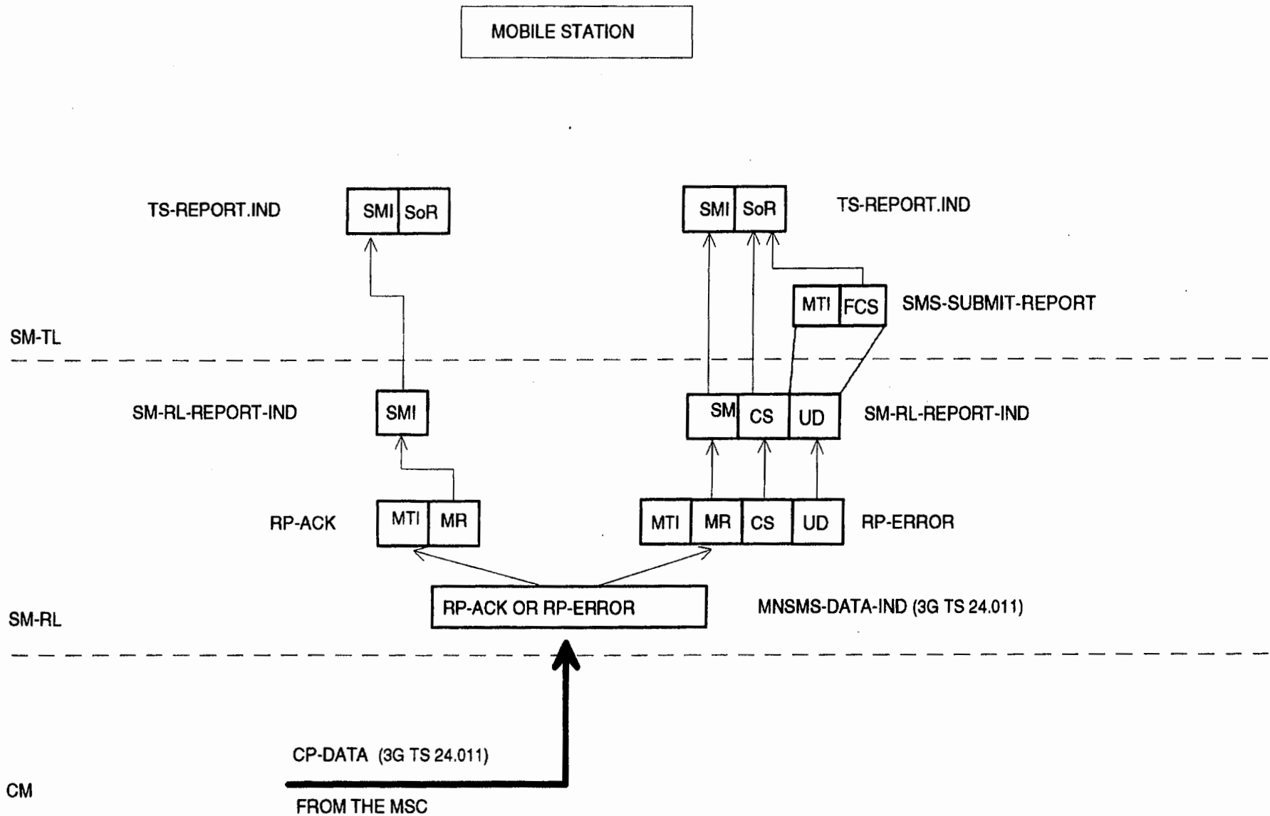
Figure C.16: Acknowledgement in the MO case
