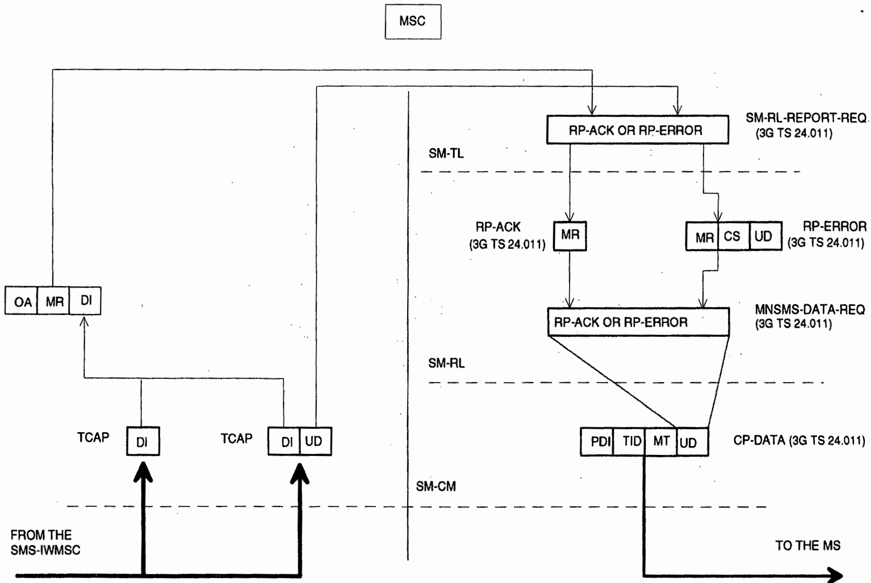
Figure C.15: Acknowledgement in the MO case
