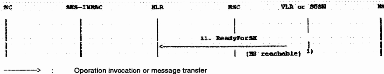
Figure 20a: The alert procedure when the MS becomes reachable, MNRF, MNRG or both are set and MCEF is not set
