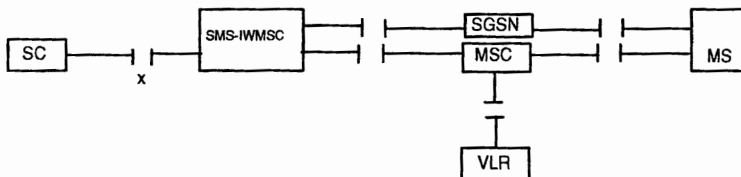
Figure 17: Interfaces involved in the Short message mobile originated procedure
