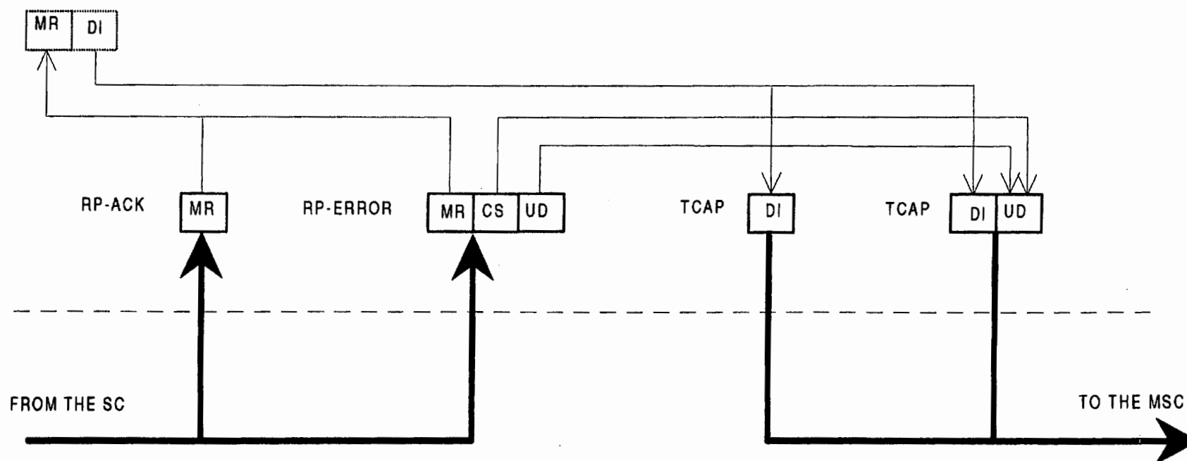
Figure C.14: Acknowledgement in the MO case
