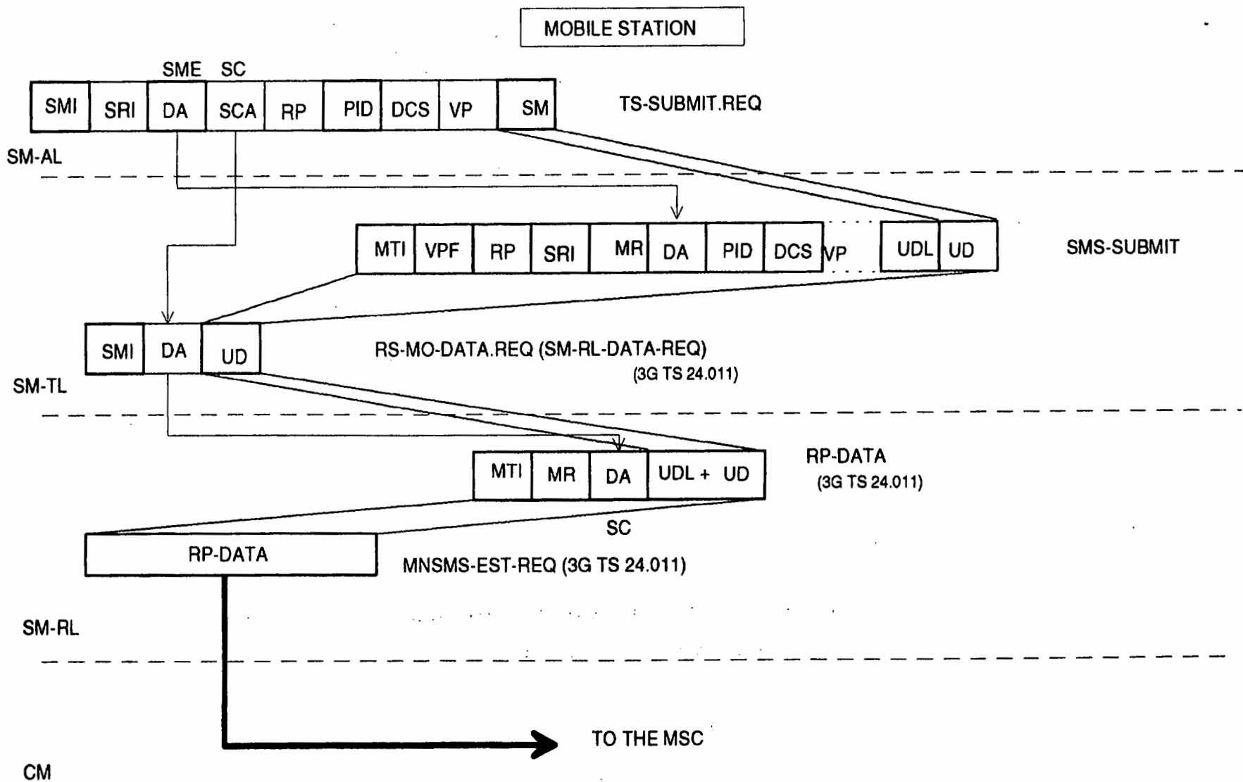
Figure C.9: Mobile originated short message
