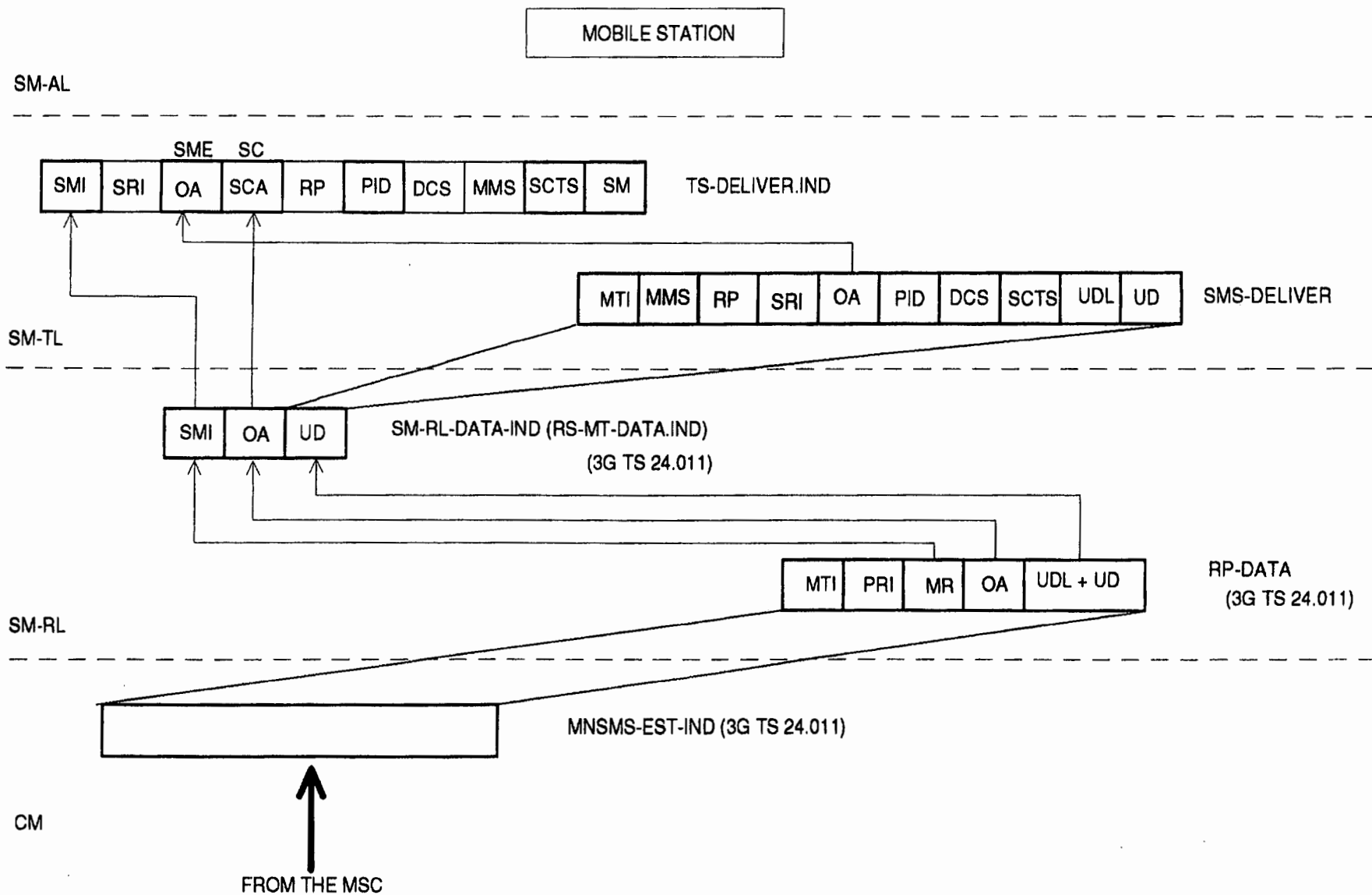
Figure C.4: Mobile terminated short message
