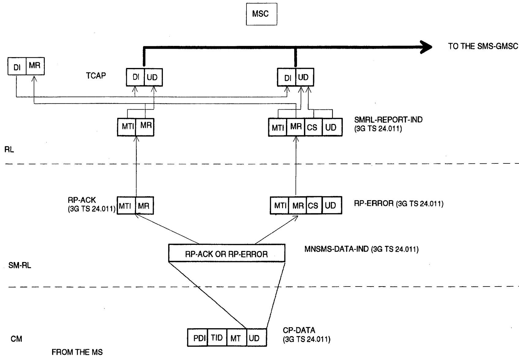
Figure C.6: Acknowledgement in the MT case
