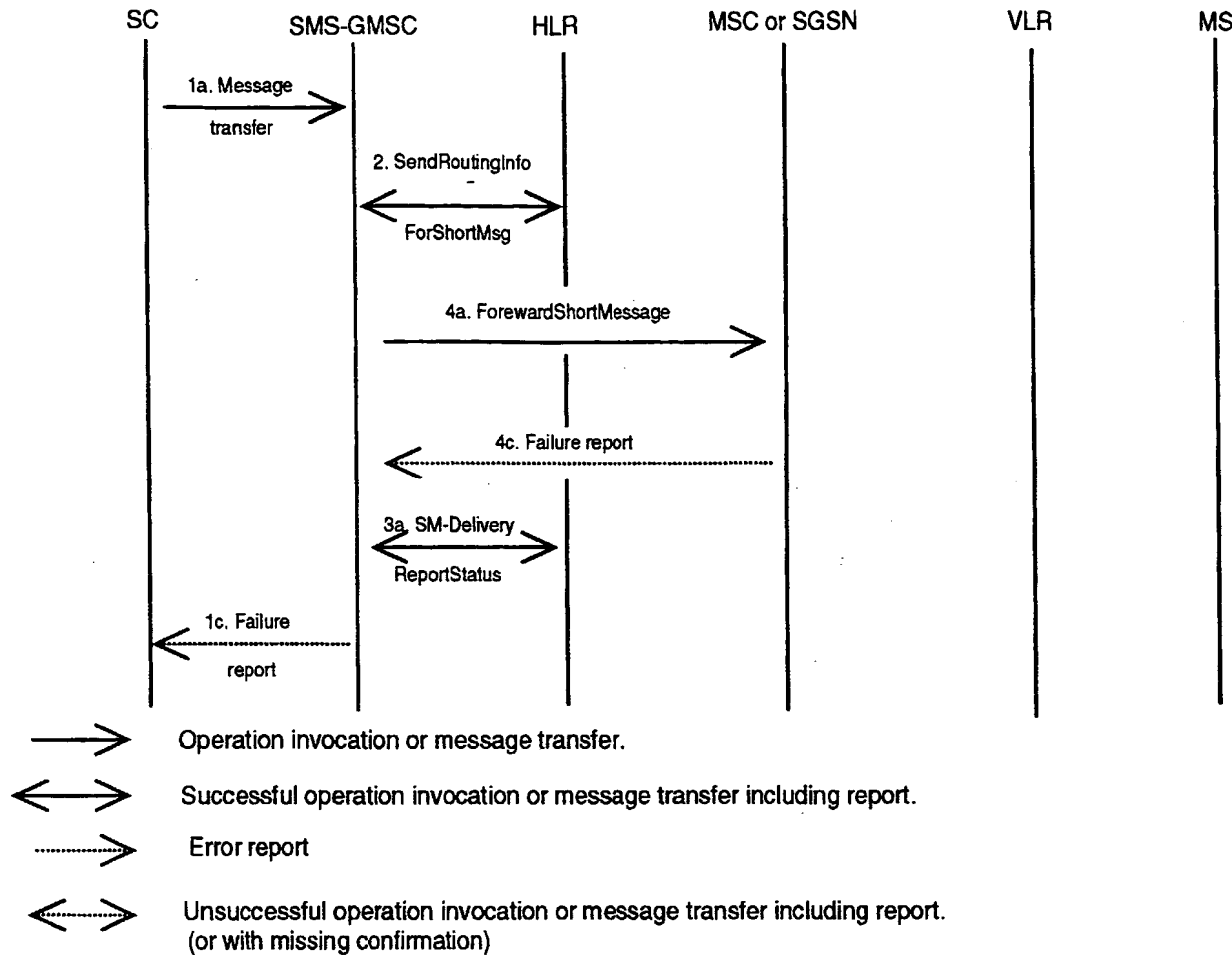
Figure 15d): Short message transfer attempt failing due to error at the MSC or SGSN
