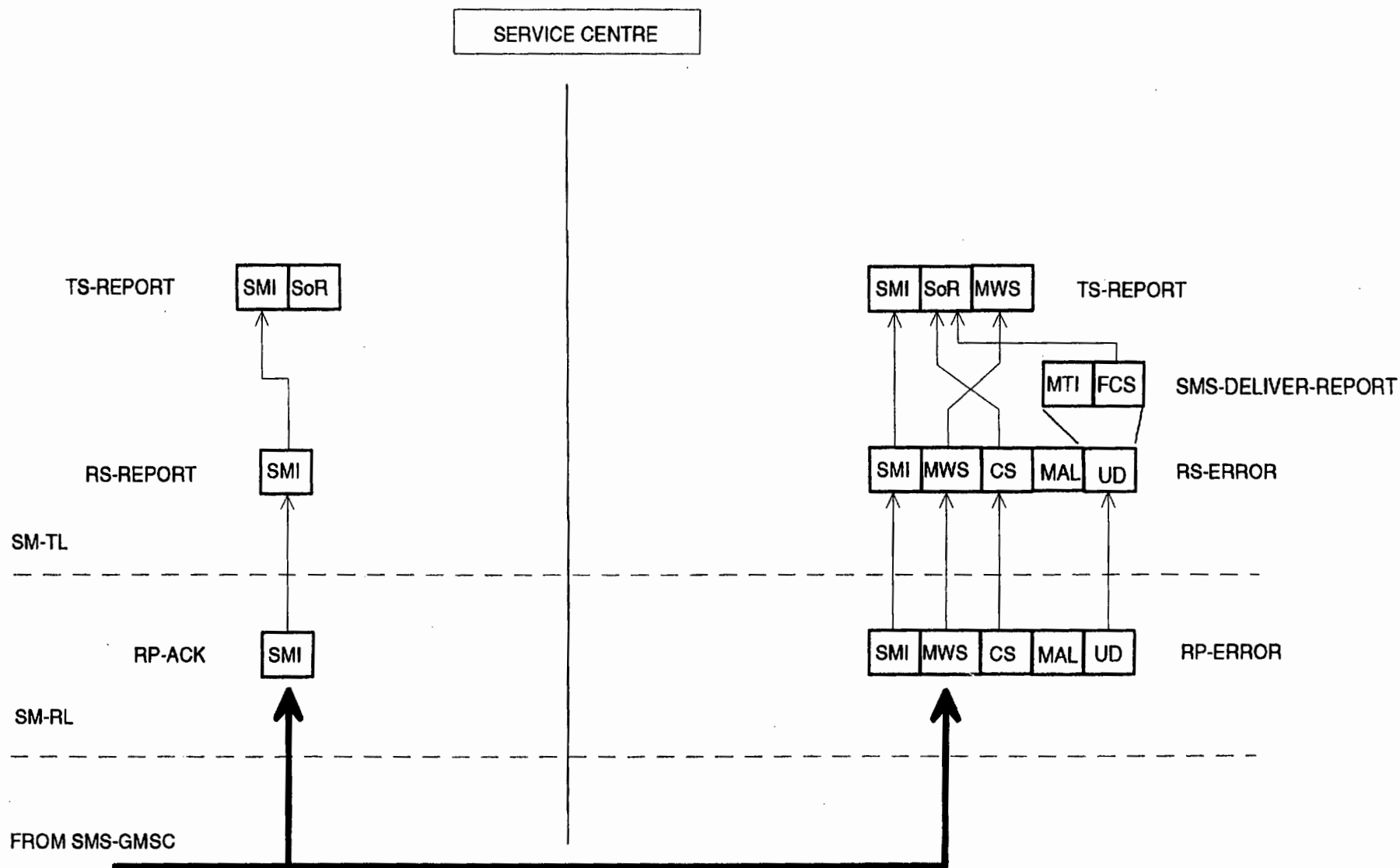
Figure C.8: Acknowledgement in the MT case
