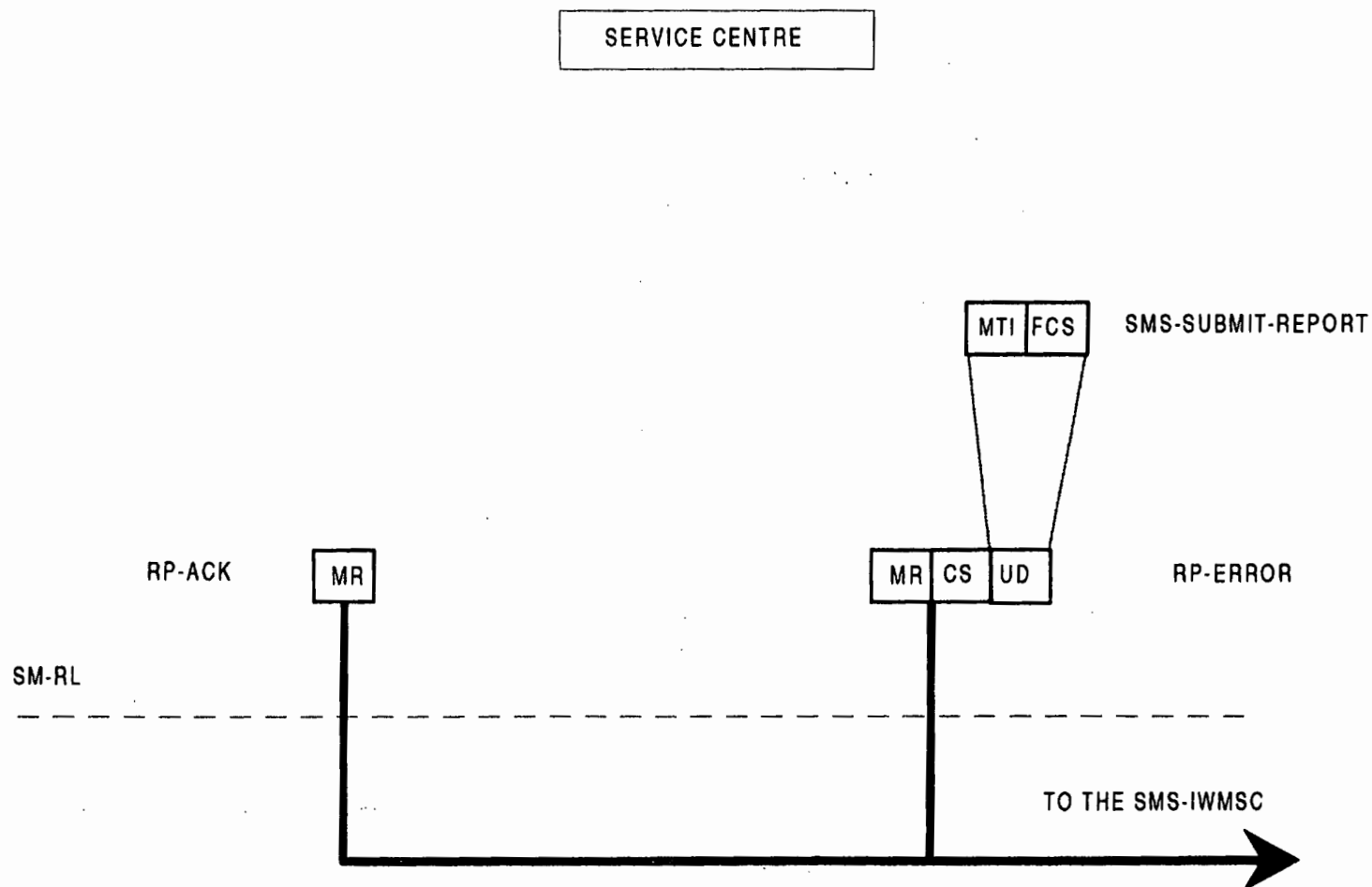
Figure C.13: Acknowledgement in the MO case
