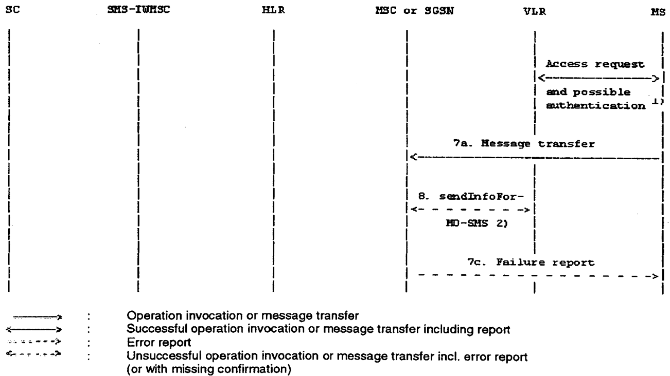
Figure 18b): Short message transfer attempt failing due to error at the MSC or SGSN
