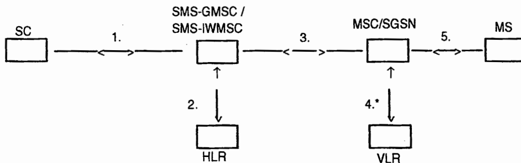
Figure 5: The main network structure serving as a basis for the short message transfer
