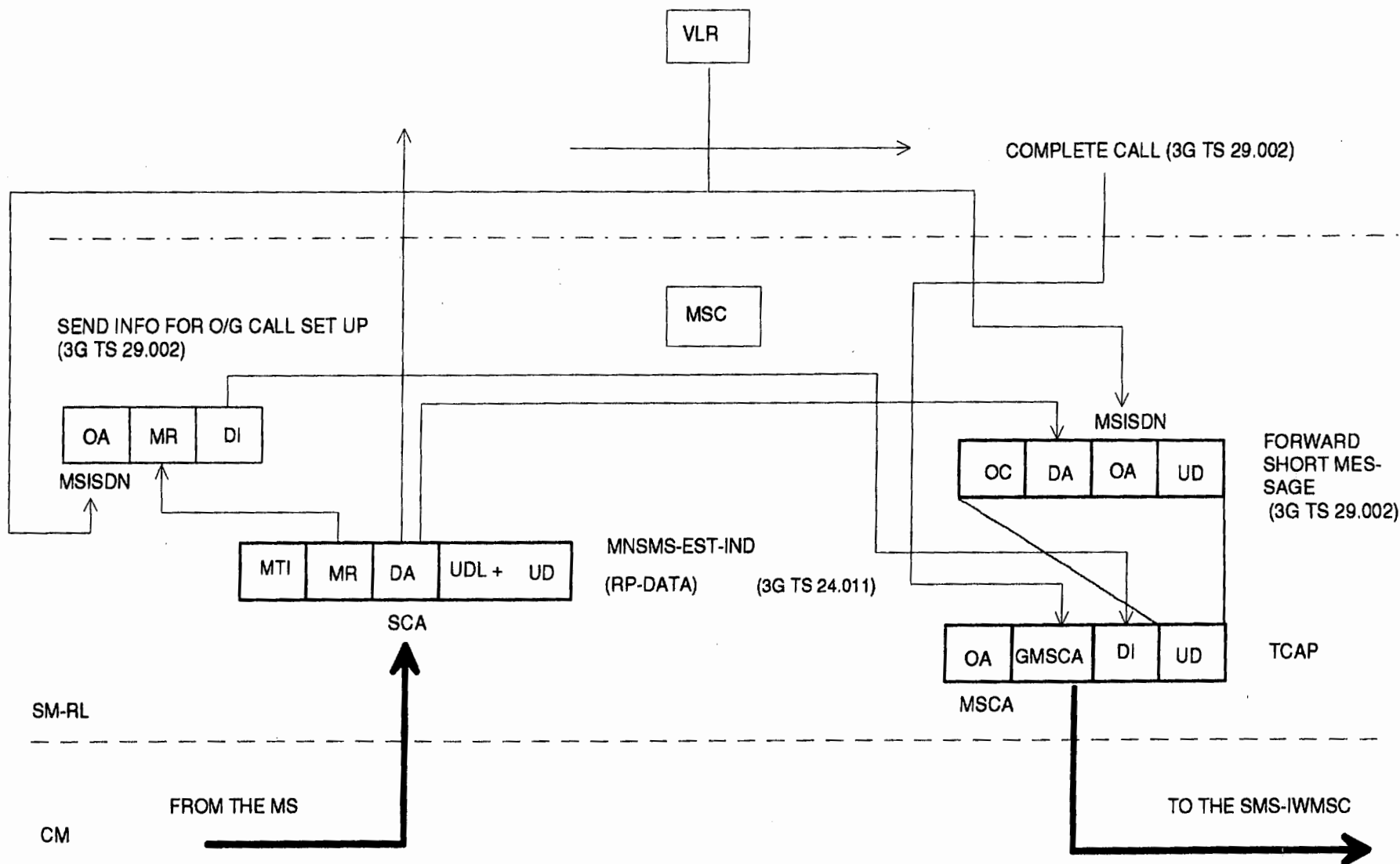
Figure C.10: Mobile originated short message
