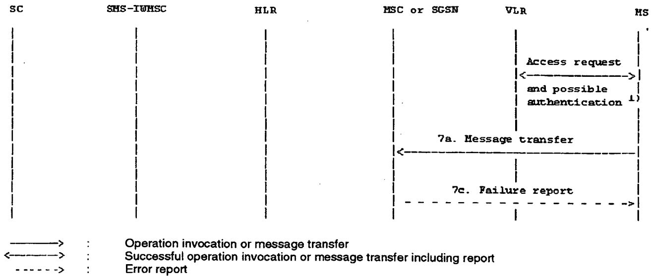
Figure 18b): Short message transfer attempt failing due to error at the MSC or SGSN
