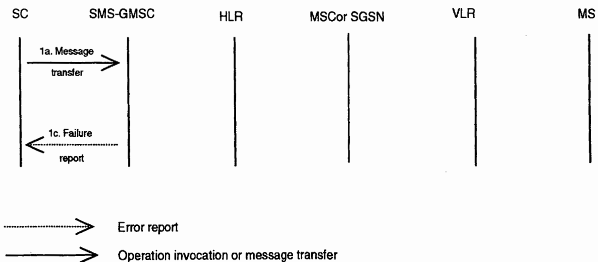
Figure 15b): Short message transfer attempt failing due to error at the SMS-GMSC
