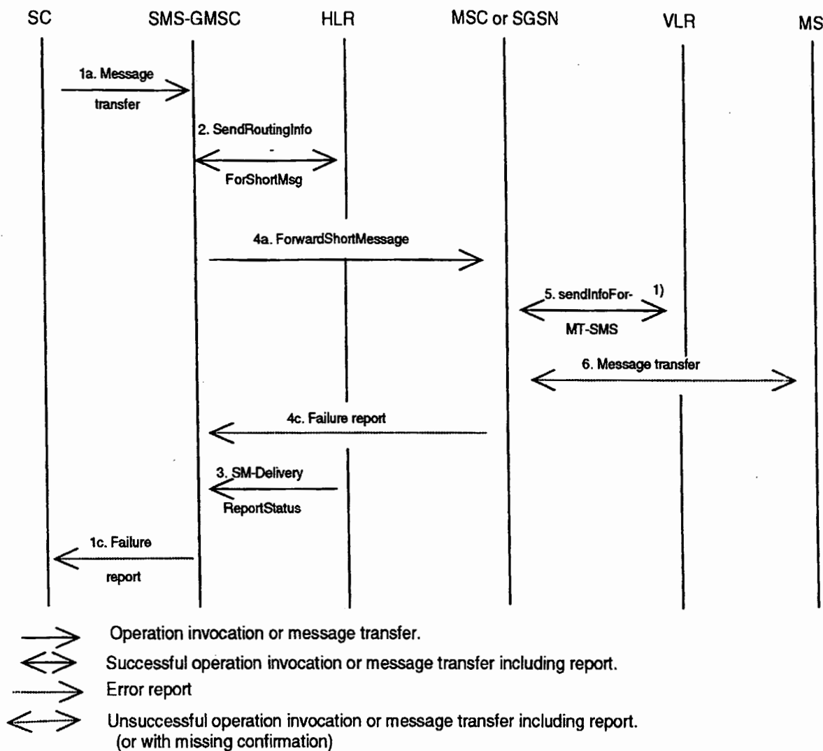
Figure 15f): Short message transfer attempt failing due to erroneous message transfer on the radio path
