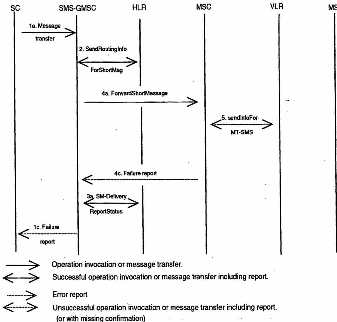
Figure 15e): Short message transfer attempt failing due to negative outcome of VLR information retrieval
