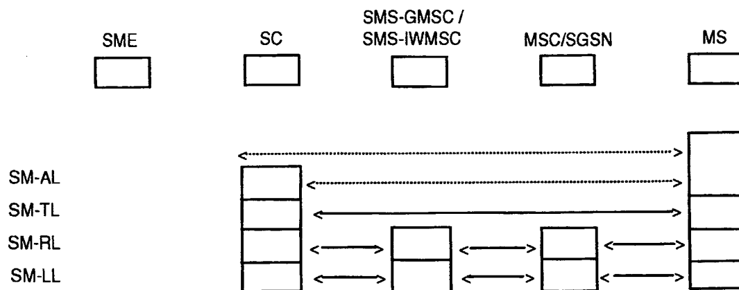
Figure 7: Protocol layer overview for the Short Message Service
