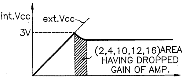
FIG. 3 (CONVENTIONAL ART)
