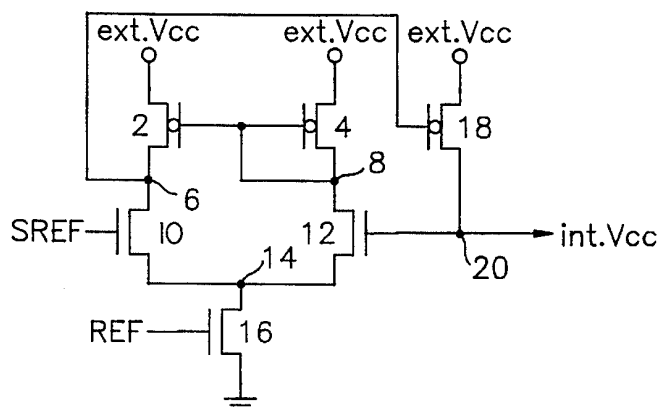
FIG. 1 (CONVENTIONAL ART)
