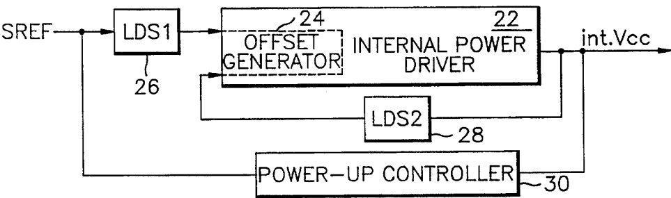
FIG. 3 (CONVENTIONAL ART)
