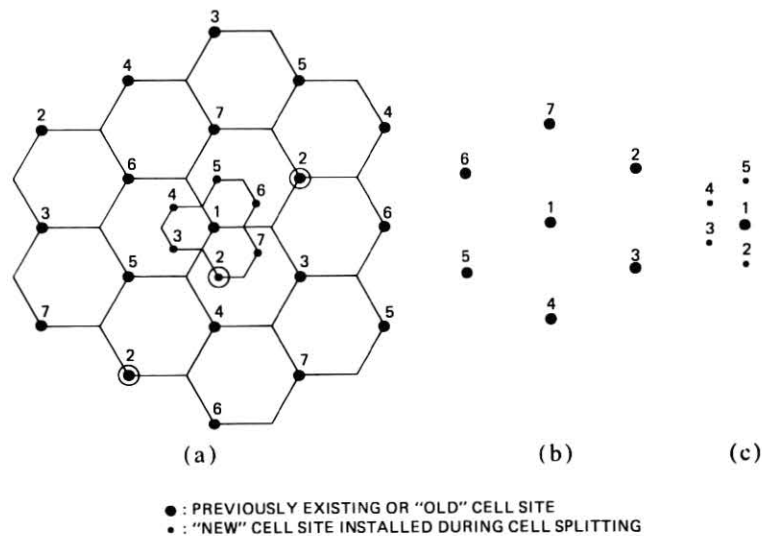
Fig. 9—Channel-set deployment pattern for seven cells per cluster, with multiple cell sizes. (a) Overall cell-site pattern. (b) Orientation of cluster of cell sites in larger-cell pattern. (c) Orientation of cluster of cell sites in smaller-cell pattern.
