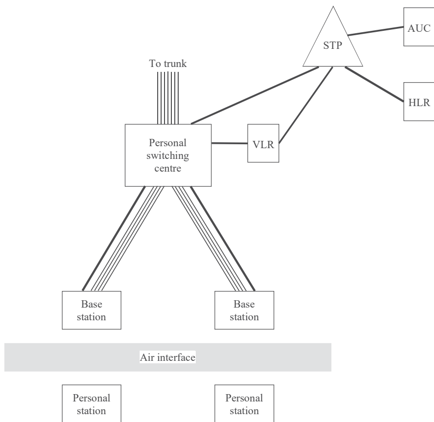
FIGURE 12 System configuration example
