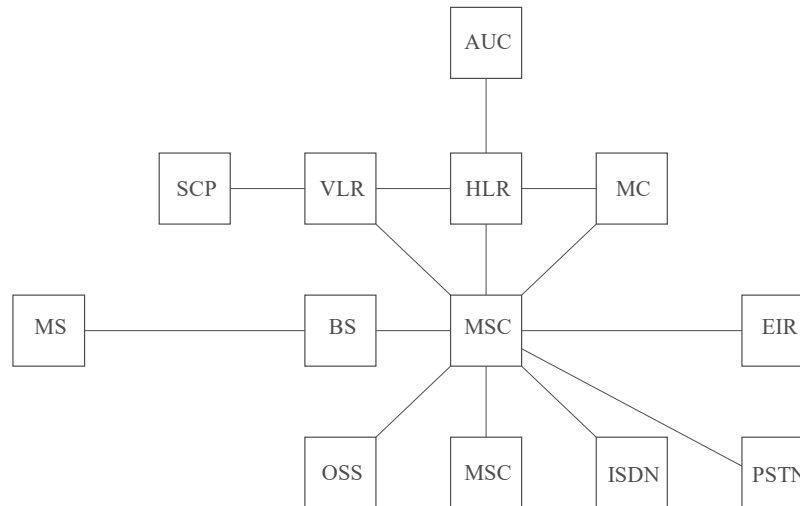
FIGURE 6 ANSI J-STD-011 based PCS network
