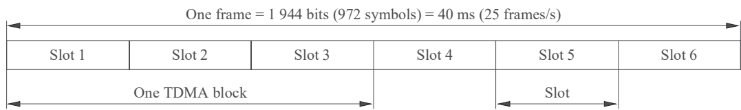
FIGURE 3 Frame structure
