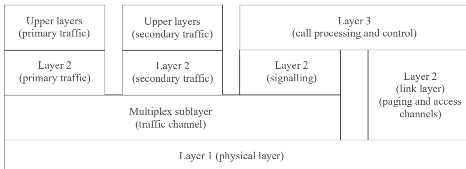
FIGURE 8 Mobile station layers
