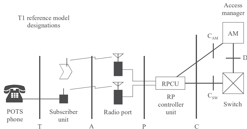
FIGURE 14 Functional reference architecture
