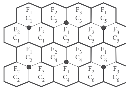
FIGURE 9 N = 3 cellular reuse
