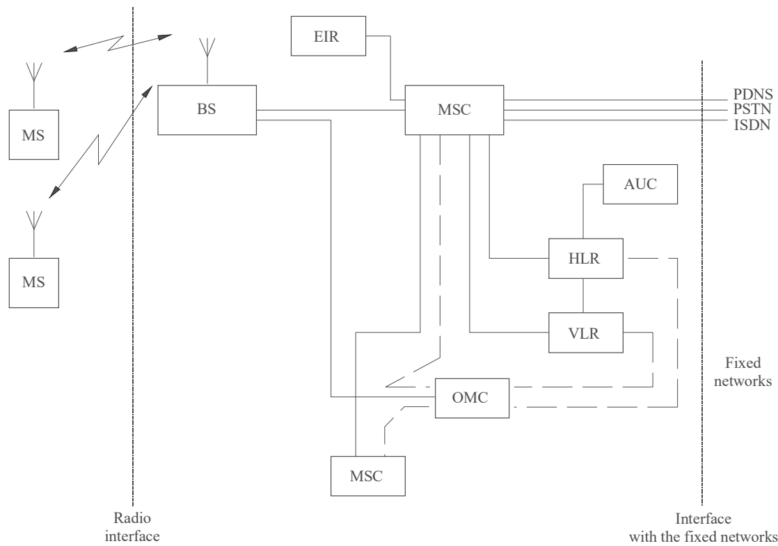
FIGURE 1 Network architecture
