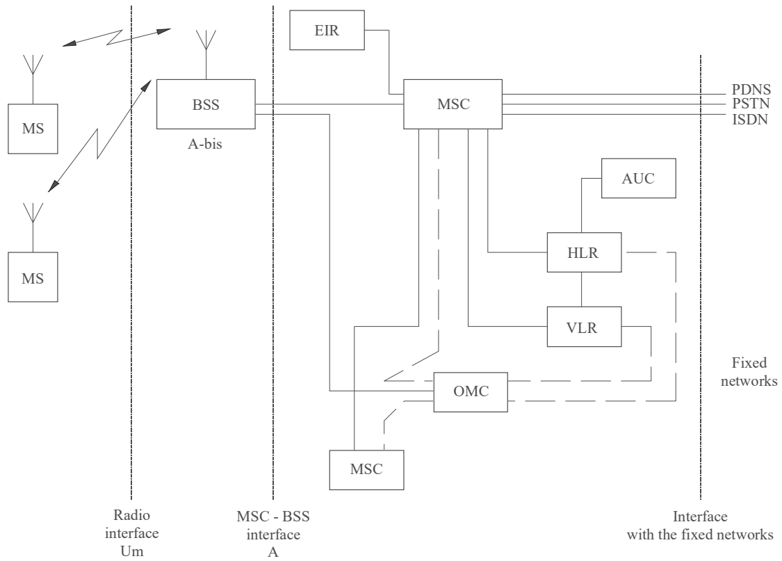
FIGURE 2 GSM 01.02 system architecture
