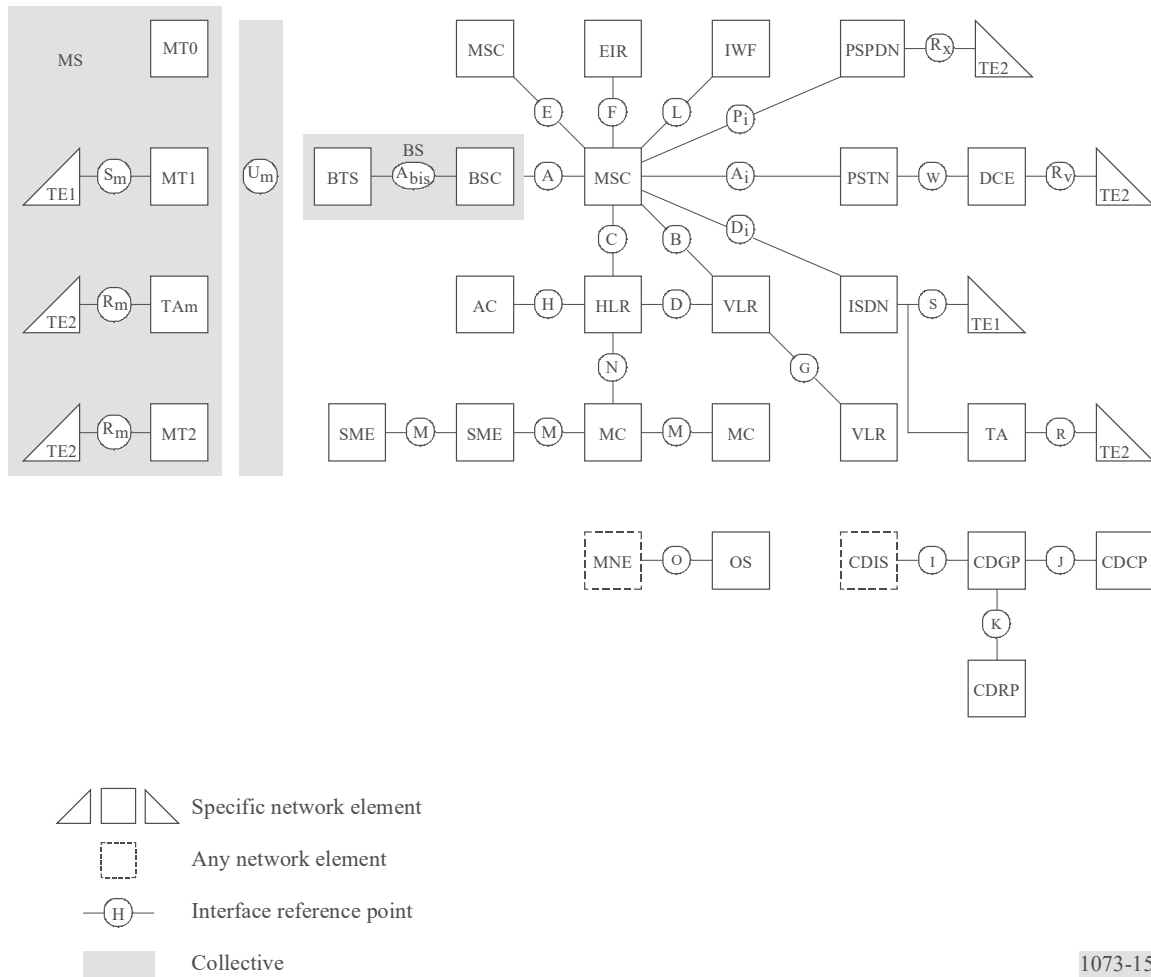
FIGURE 15 Cellular network
