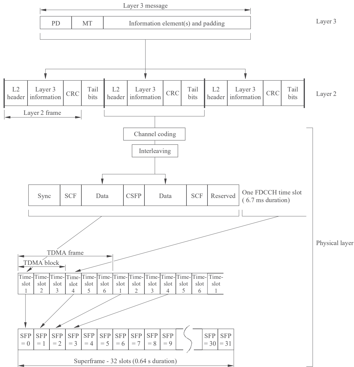
FIGURE 4 Message layering
