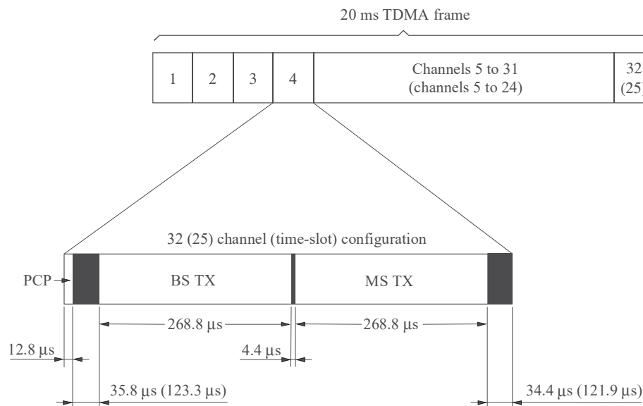
FIGURE 10 TDMA frame and TDMA channel time-slot structure
