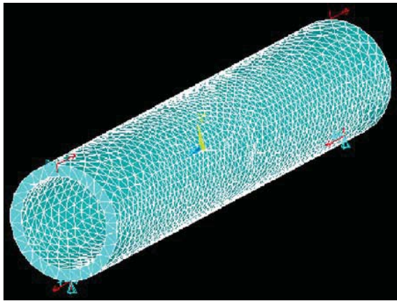
Fig. 5. Finite element model of the tube with 20 mm wall thickness
