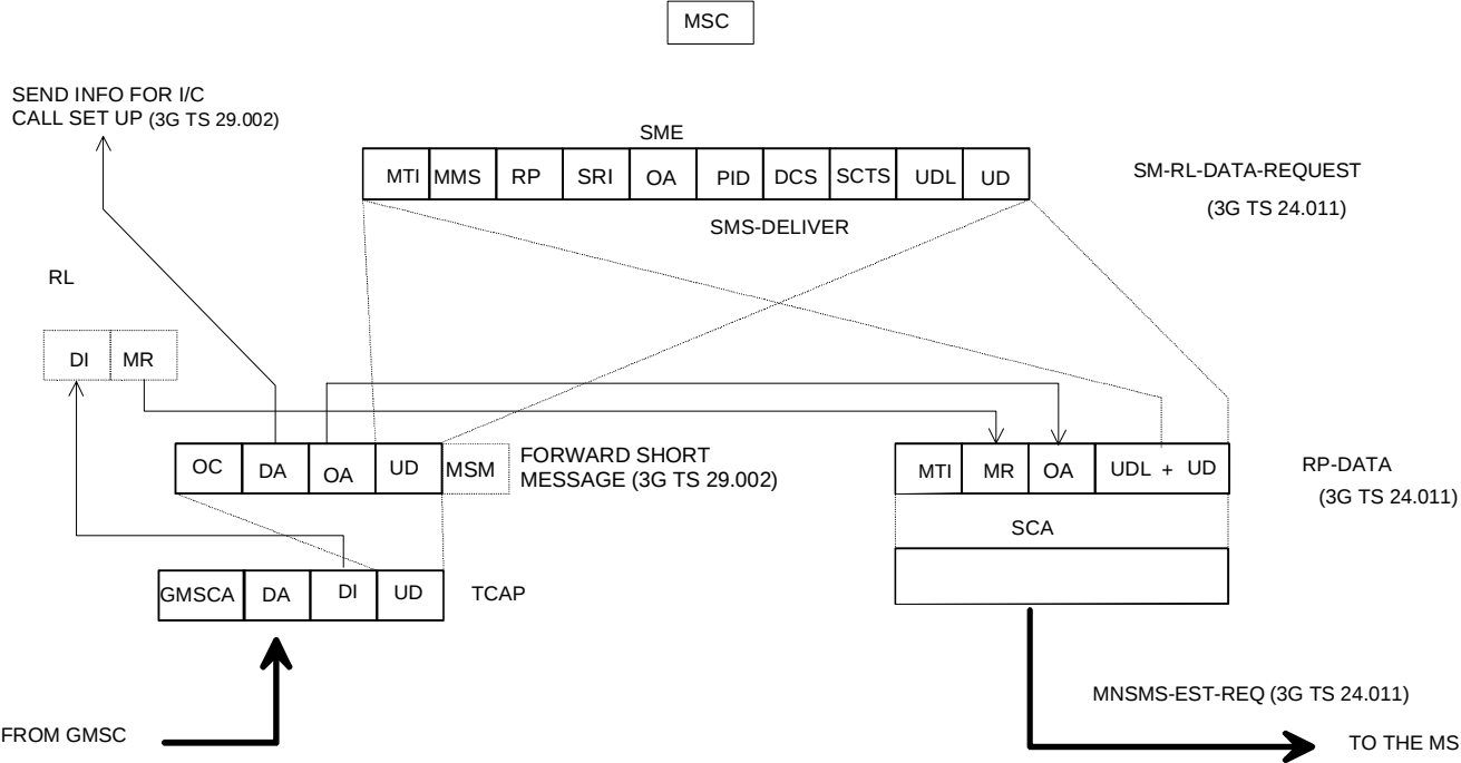
Figure C.3: Mobile terminated short message
