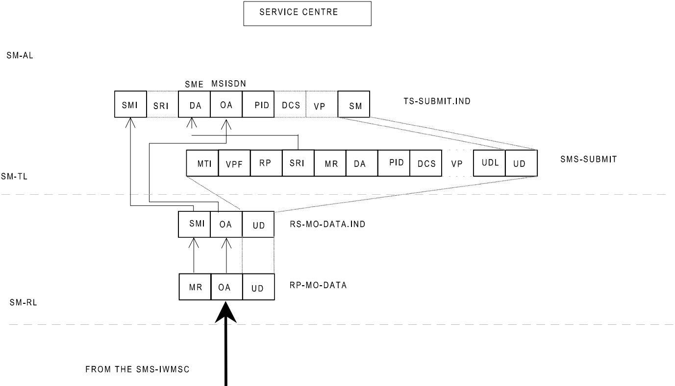
Figure C.12: Mobile originated short message
