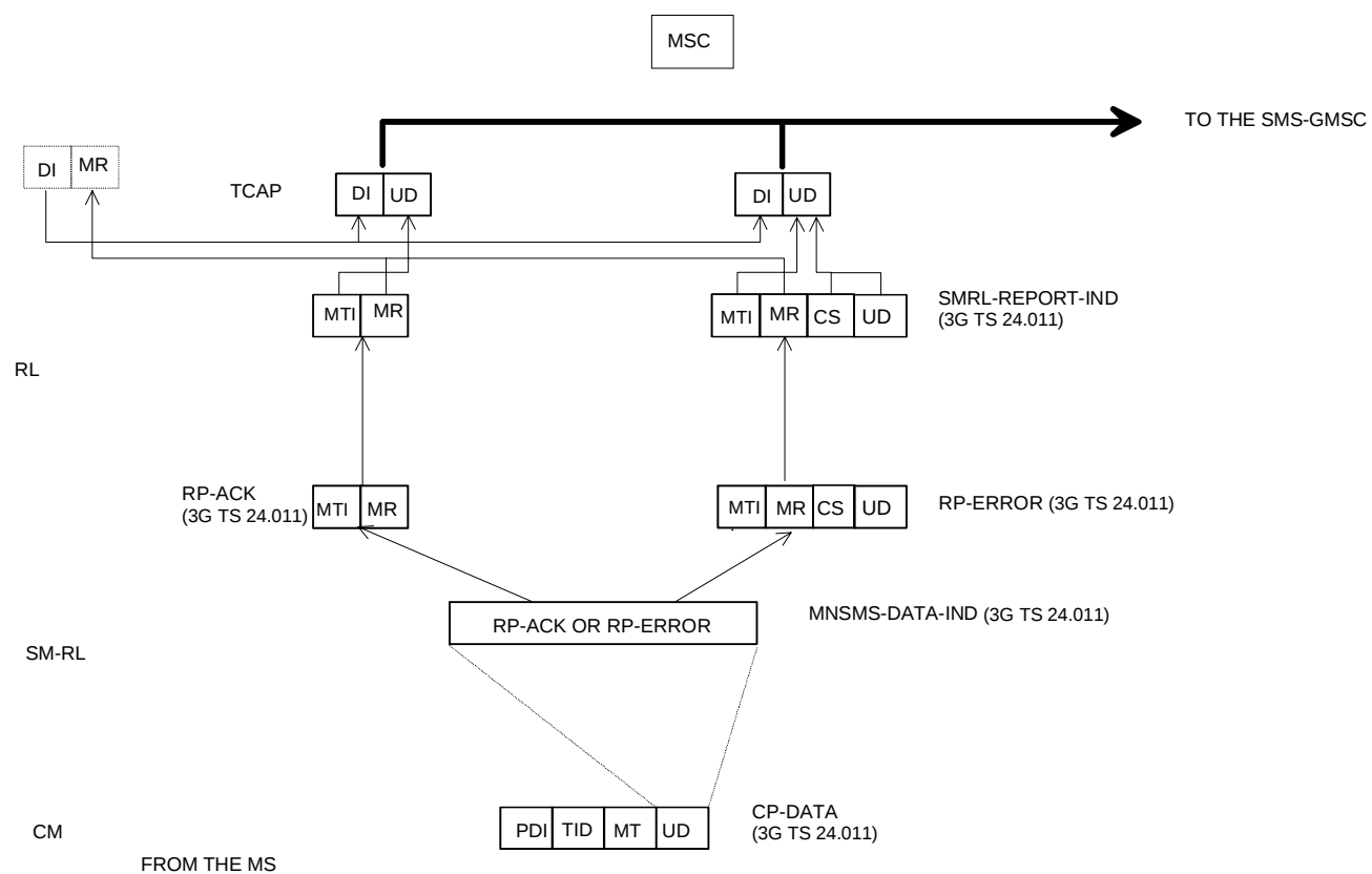
Figure C.6: Acknowledgement in the MT case
