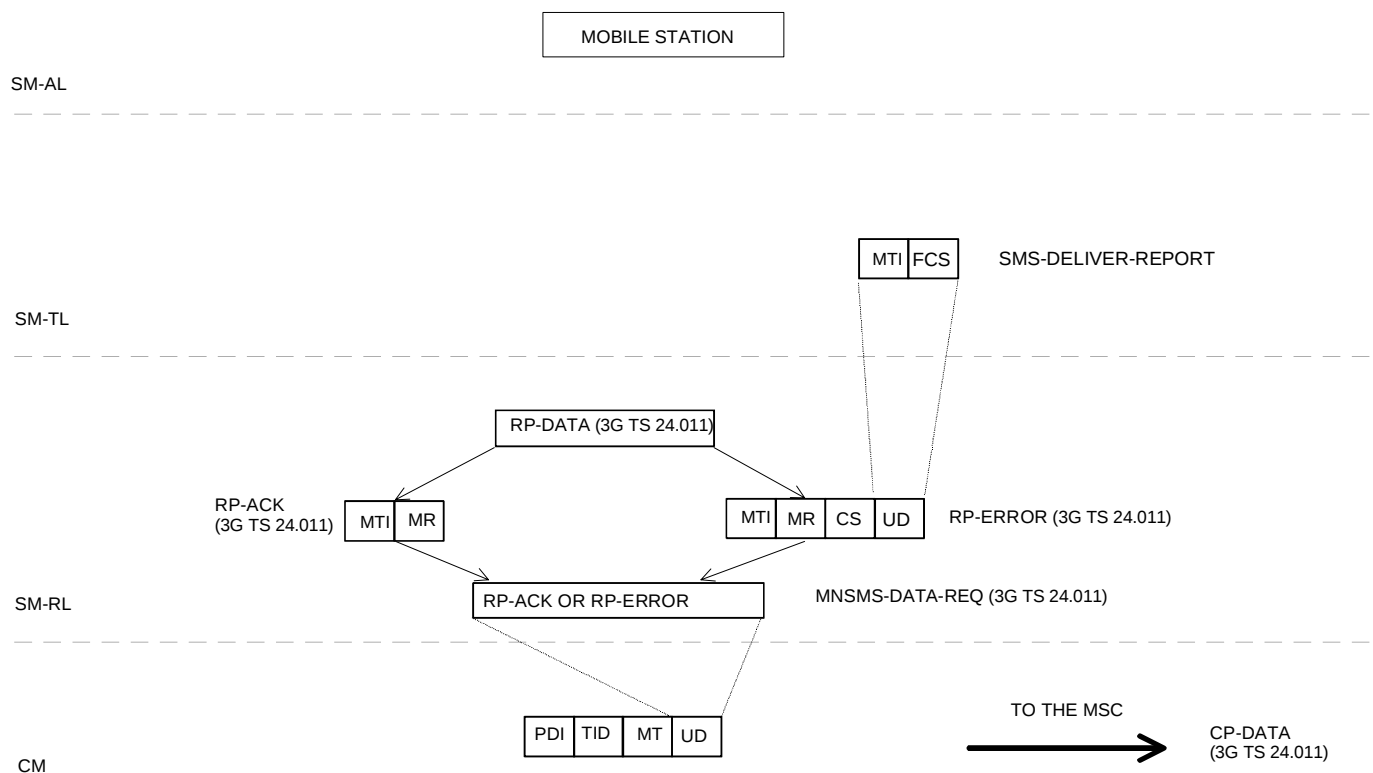
Figure C.5: Acknowledgement in the MT case
