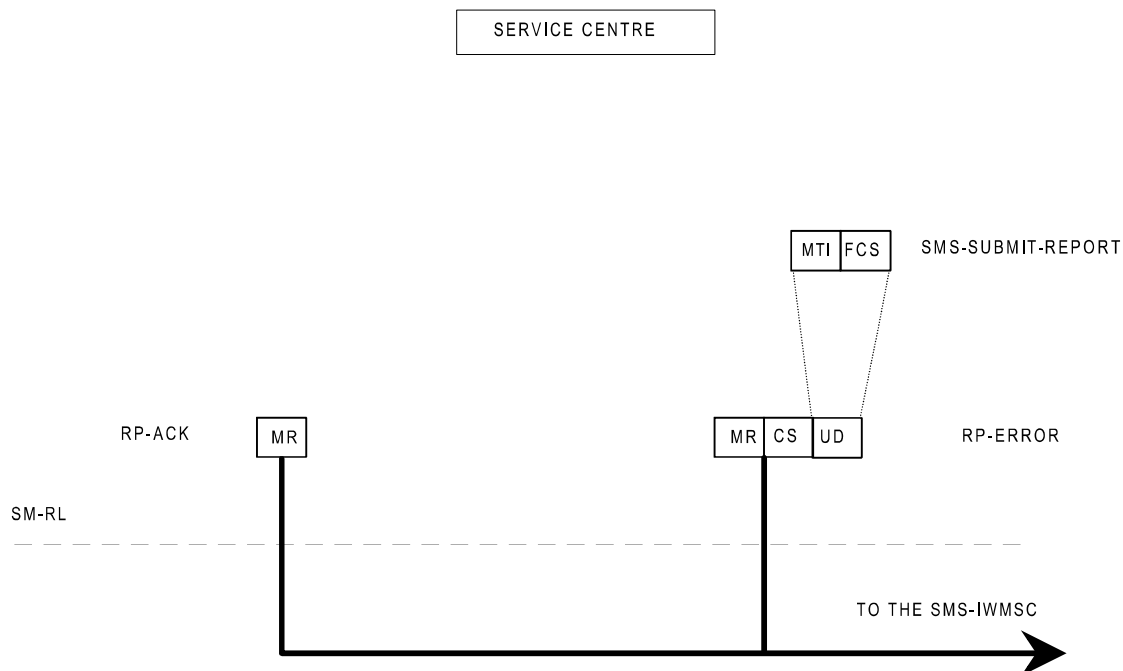
Figure C.13: Acknowledgement in the MO case
