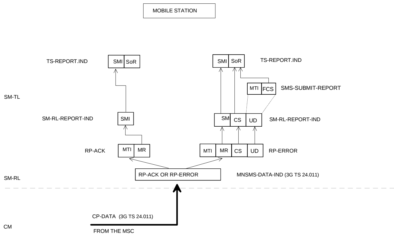
Figure C.16: Acknowledgement in the MO case
