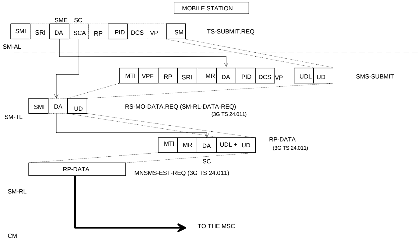
Figure C.9: Mobile originated short message
