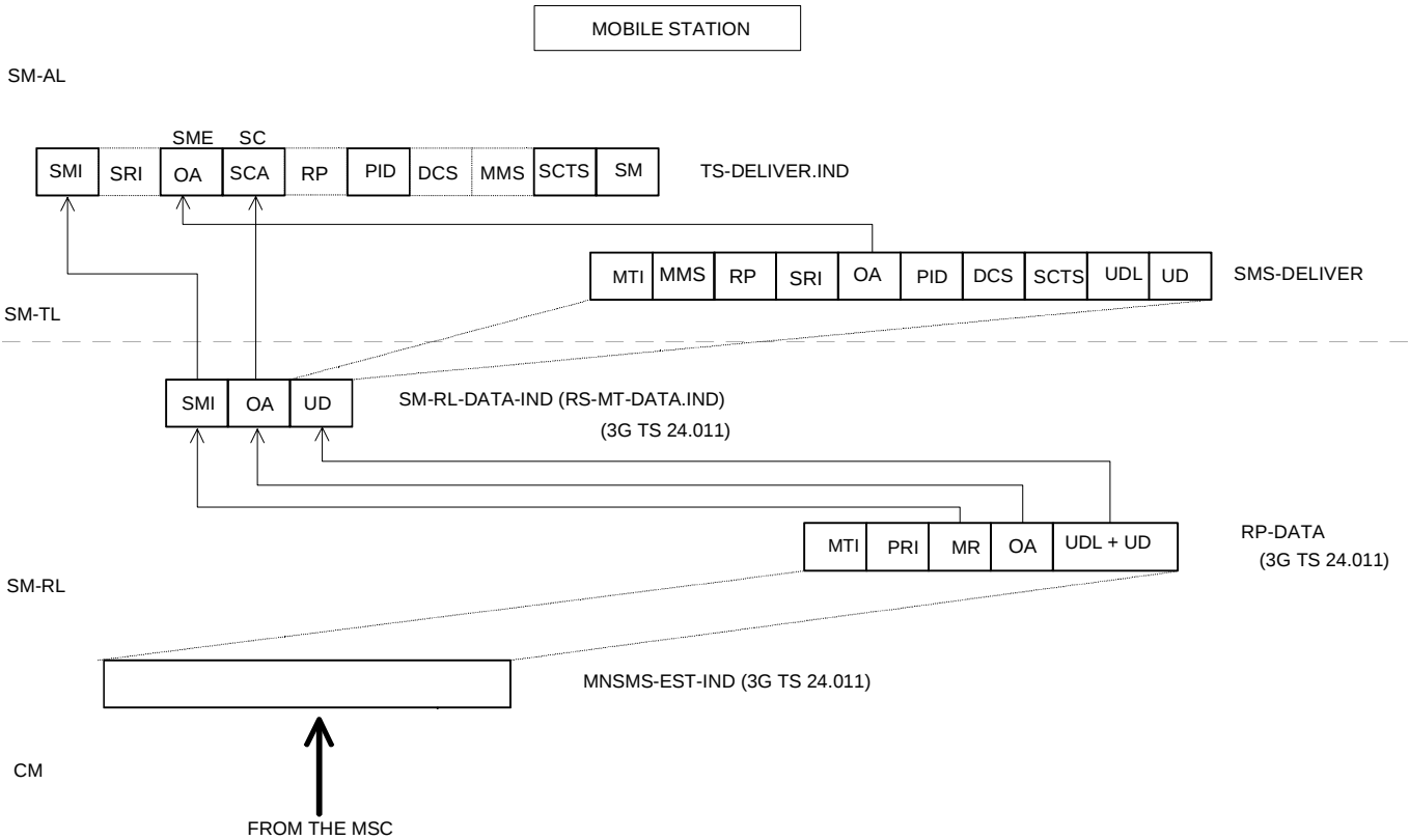
Figure C.4: Mobile terminated short message
