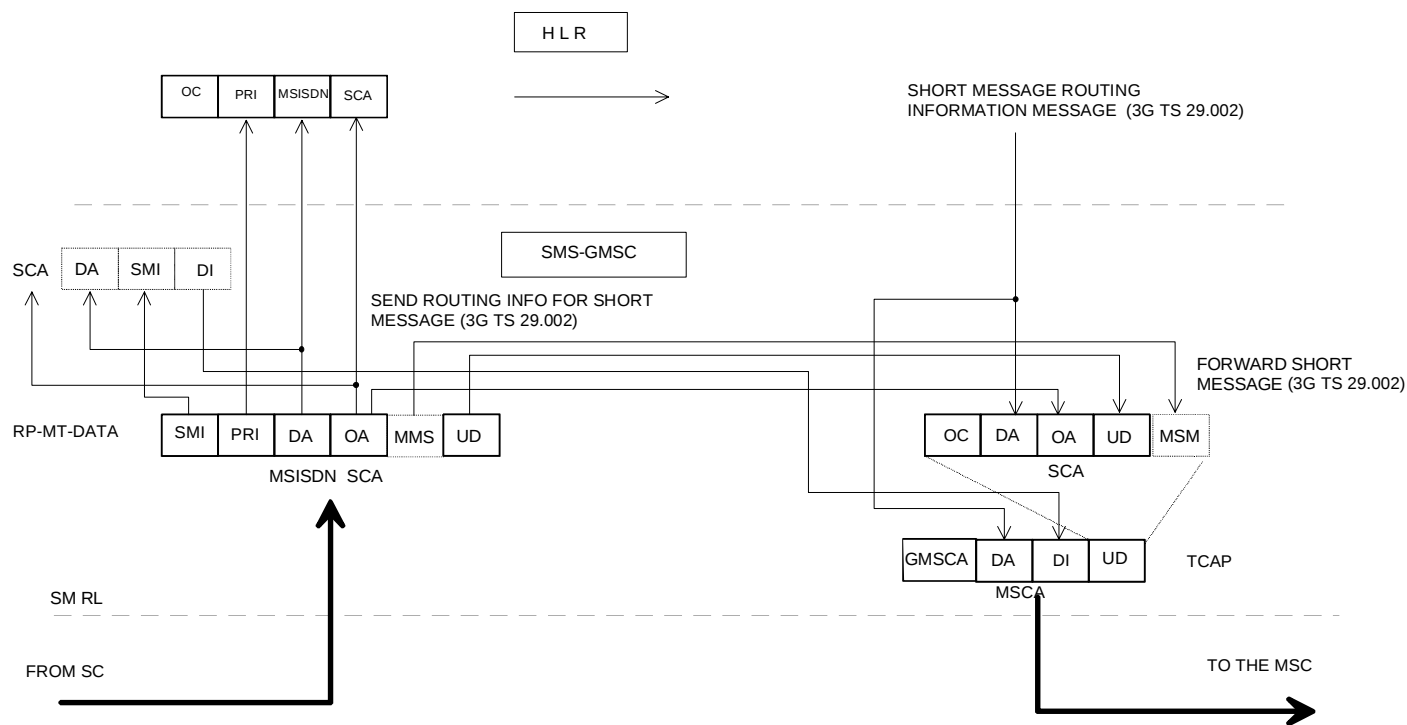
NOTE: A sequence of short messages shall have MMS set to 1 in each RP-MT-DATA except the last (last shall have MMS set to 0). Each RP-MT-DATA shall be carried via FORWARD SHORT MESSAGE via TCAP and shall be assigned the same Dialogue Identifier as previous RP-MT-DATAS in the sequence. Figure C.2: Mobile terminated short message
