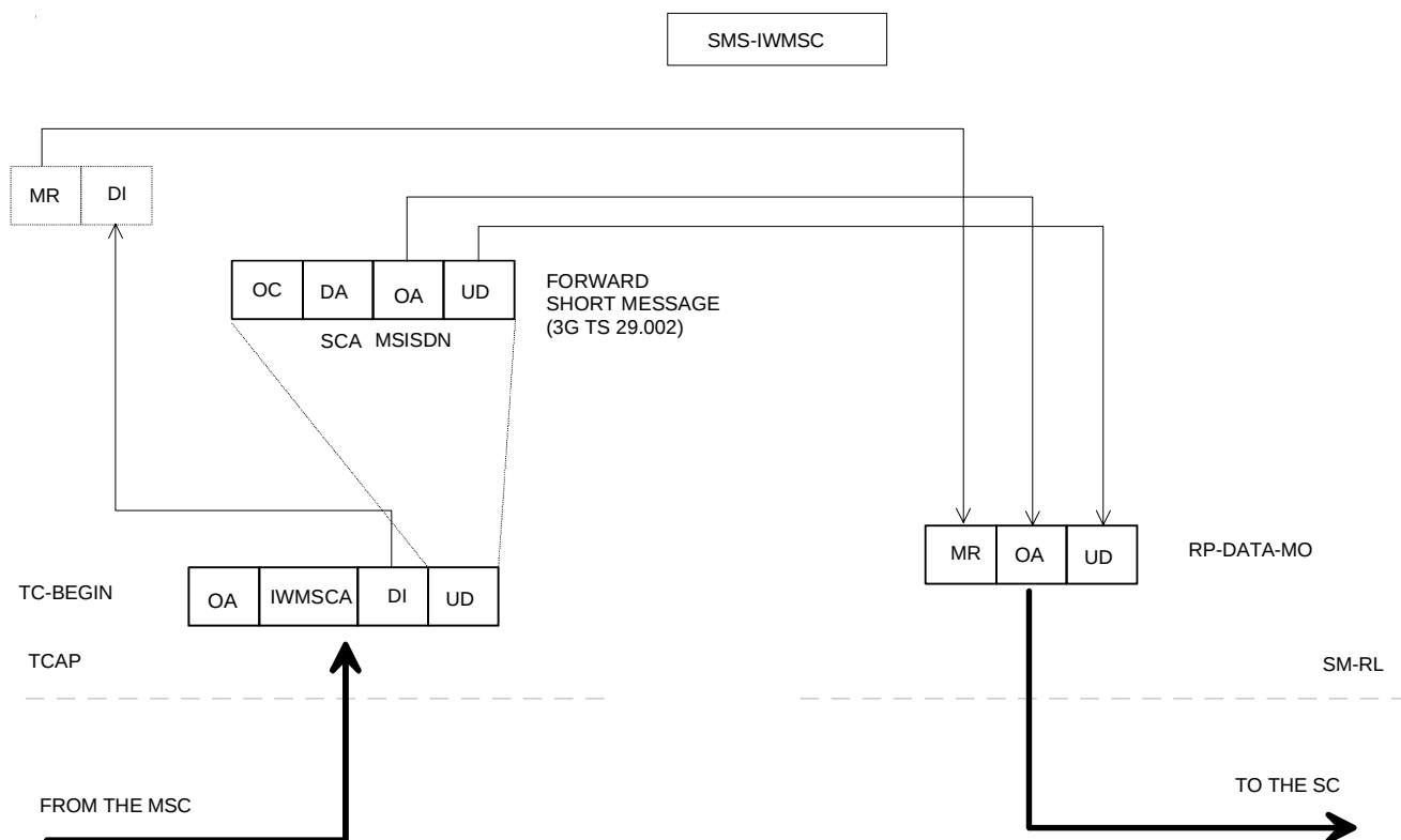
Figure C.11: Mobile originated short message
