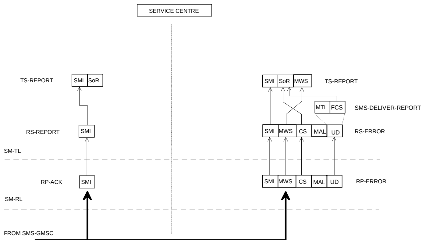
Figure C.8: Acknowledgement in the MT case
