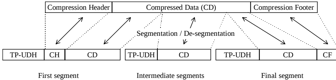
Figure 9.2.3.24.1 (a): Concatenation of a Compressed short message
