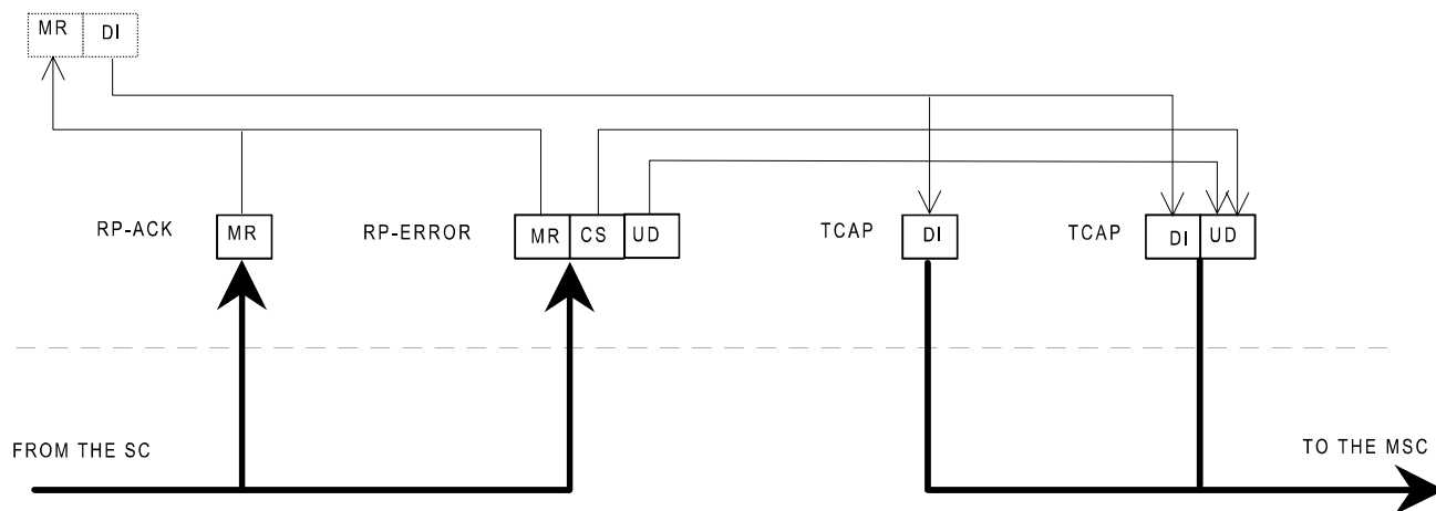
Figure C.14: Acknowledgement in the MO case
