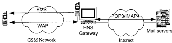
Fig. 12. Architecture of e-mail services.
