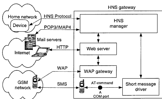
Fig. 6. Architecture of the HNS gateway.
