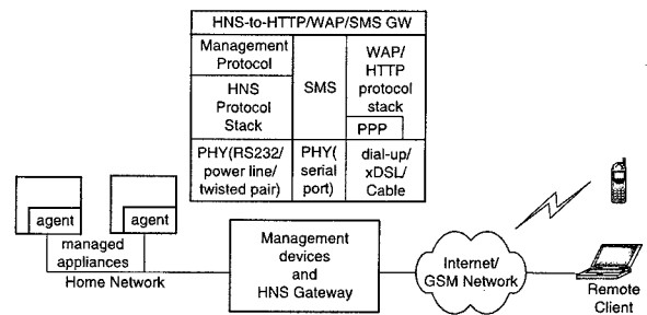
Fig. 7. Protocol stack of the HNS gateway.
