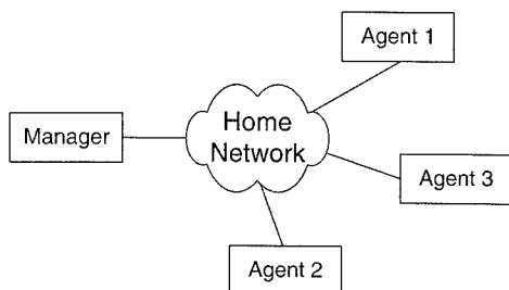
Fig. 4. Manager-agent model.
