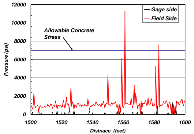
Figure 4. Field and gage side pressures around the derailment site.
