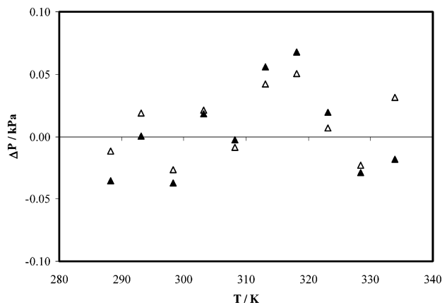
Figure 4. Comparison between correlated experimental and literature vapor pressure data of perfluorotoluene: ▲, this work; △, Ambrose et al. 17 \Delta P = P_{\text{exptl}} - P_{\text{calcd}} .
