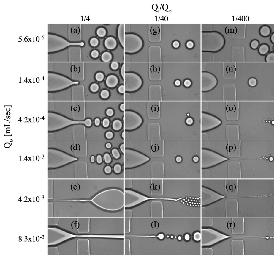
FIG. 3. Phase diagram for drop formation in flow focusing. Each image represents the drop sizes and drop patterns that form at the specified value of Q_o (rows) and Q_i/Q_o (columns). We note that for these flows the Reynolds numbers \mathcal{R} = Q/(\nu h) , where \nu is the kinematic viscosity of the fluid and h is the height of the channel, of the oil ( o ) and water ( i ) are in the ranges 0.07 < \mathcal{R}_o < 12 and 0.001 < \mathcal{R}_i < 18 , which are typically smaller than the values for the original flow-focusing studies (see Refs. 11 and 12).
