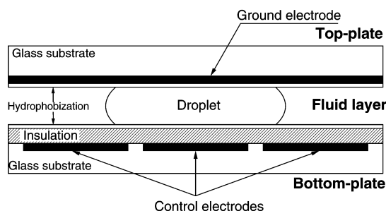
Fig. 2 Schematic cross-section of the electrowetting chip.
