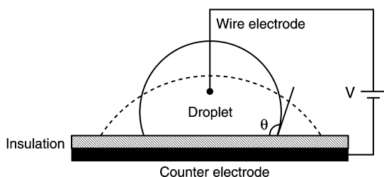
Fig. 1 The electrowetting effect. A droplet of conducting liquid initially forms a contact angle \theta with a solid hydrophobic insulator (solid contour). Application of a voltage V between the droplet and a counter-electrode underneath the insulator reduces the solid-liquid interfacial energy, leading to a reduction in \theta and improved wetting of the solid by the droplet (dashed contour).
