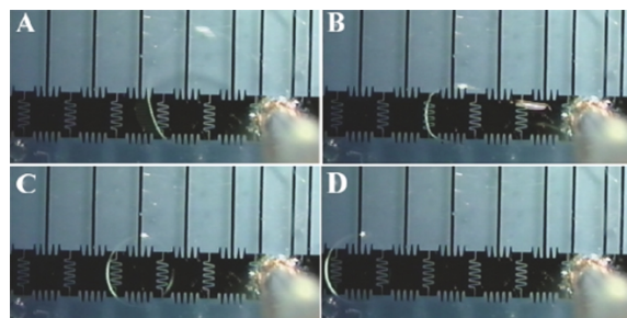
Fig. 10 Time-lapse series, droplet dispensing from an external source. Electrolyte is introduced under pressure through a pipette-tip fitted to a hole in the top-plate (A). The fluid is allowed to retract (B) and a new microdroplet is left on an energized electrode (C). The droplet is then transported away (D) and the process repeated. The total elapsed time is about 2 s and the droplet volume is about 700 nl.
