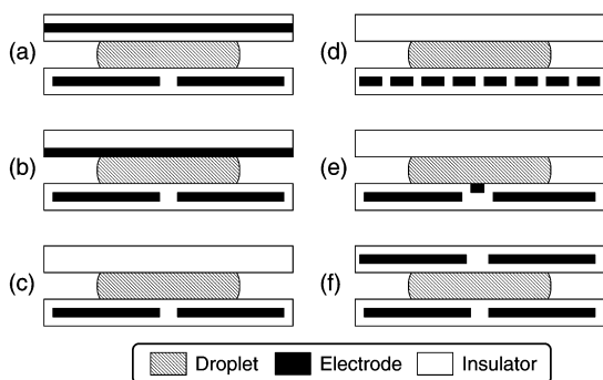
Fig. 3 Alternative microactuator electrode arrangements.
