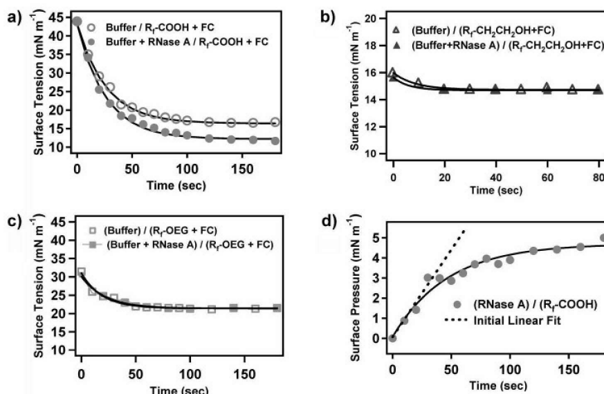
Figure 5. Graphs of surface tension versus time for RNase A at an interface that presented one of the following three surfactants: R f -COOH (●), R f -CH 2 CH 2 OH (▲) or R f -OEG (■). Open symbols indicate (buffer)/(surfactant + FC) control droplets; closed symbols indicate (buffer + RNase A)/(surfactant + FC) test droplets. (a) RNase A adsorbed to the interface that presented R f -COOH. The surface tension of the test droplet was lower than the surface tension of the control. RNase A did not adsorb to interfaces that presented either the R f -CH 2 CH 2 OH (b) or the R f -OEG surfactant (c). In (b, c), the surface tension of the test droplet matched the surface tension of the control droplet. (d) The difference in surface tension between (buffer)/(surfactant + FC) controls and (buffer + RNase A)/(surfactant + FC) tests for R f -COOH (●) surfactant was plotted as surface pressure versus time, and a fit was applied to obtain the rate constant for adsorption.
