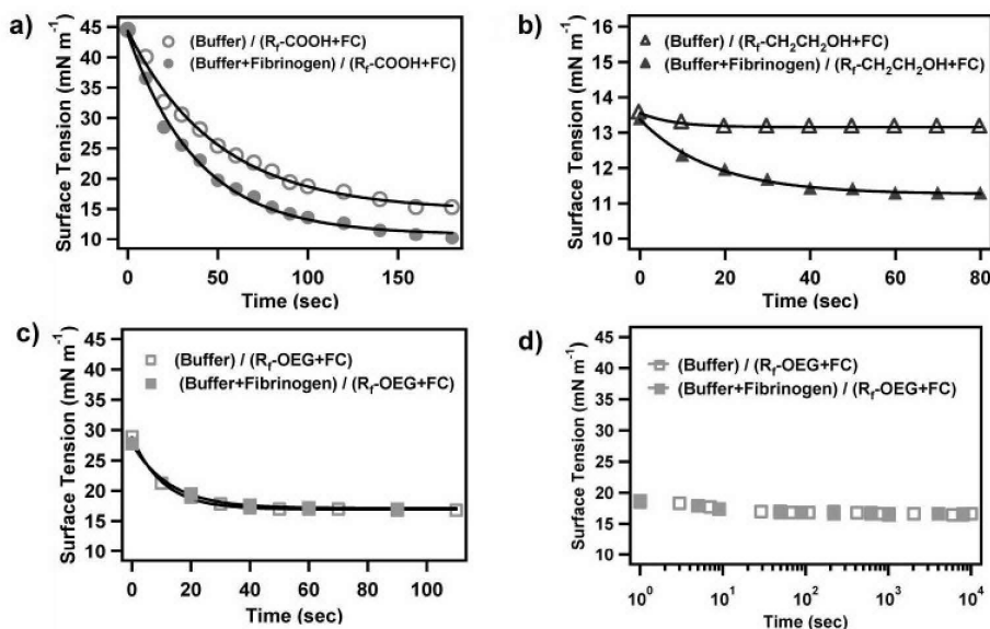
Figure 4. Graphs of surface tension versus time for fibrinogen at an interface that presented one of the following three surfactants: R f -COOH (●), R f -CH 2 CH 2 OH (▲) or R f -OEG (■). Open symbols indicate (buffer)/(surfactant + FC) control droplets; closed symbols indicate (buffer + fibrinogen)/(surfactant + FC) test droplets. Fibrinogen adsorbed to interfaces that presented either the R f -COOH surfactant (a) or the R f -CH 2 -CH 2 OH surfactant (b). In (a, b), the surface tension of the test droplet was lower than the surface tension of the control droplet. (c) Fibrinogen did not adsorb to the interface that presented R f -OEG. The surface tension of the test droplet matched the surface tension of the control droplet. (d) Concentrated fibrinogen does not adsorb to an interface presenting the R f -OEG surfactant for times up to 10 4 s.
