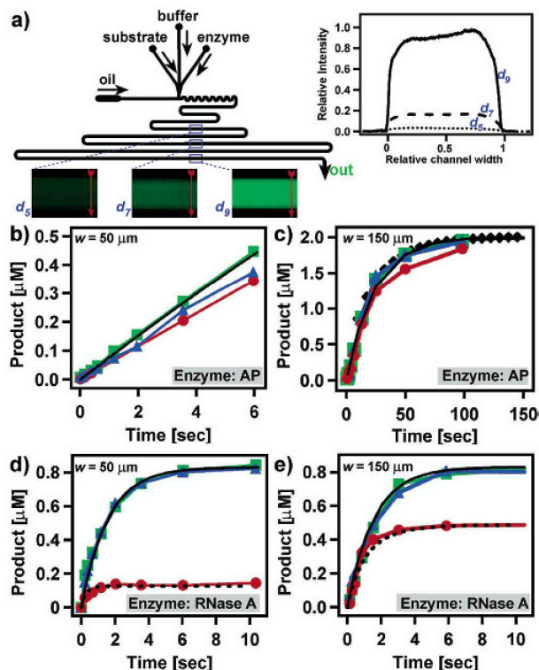
Figure 7. Quantitative test for adsorption in plugs. (a) Left: A schematic of the microchannel network for measuring exponential enzyme kinetics. The blue rectangles outline the field of view for the false-color fluorescence microphotographs obtained at three microchannel distances: d_5 , d_7 , and d_9 . Right: Intensity profiles were obtained across the region indicated by the red arrow for each microphotograph. (b-e) Enzyme kinetics was measured within microfluidic devices for w = 50 \mu\text{m} (in b, d) and w = 150 \mu\text{m} (in c, e) for three different surfactants: R_f\text{-COOH} (●), R_f\text{-CH}_2\text{CH}_2\text{OH} (▲), and R_f\text{-OEG} (■). (b, c) Kinetic measurements for alkaline phosphatase (AP). Solid black curves represent expected kinetic curves for fully active AP, obtained from fluorimeter data (◆). (d, e) Kinetic measurements for RNase A. Solid black lines represent expected curves for fully active RNase A. Dashed black lines represent numerical fits according to eq 7 and Michaelis-Menten kinetics, where fits were obtained using k_a = 1.4 \times 10^{-2} \text{ mL } \mu\text{g}^{-1} \text{ s}^{-1} (d) and k_a = 0.9 \times 10^{-2} \text{ mL } \mu\text{g}^{-1} \text{ s}^{-1} (e).
