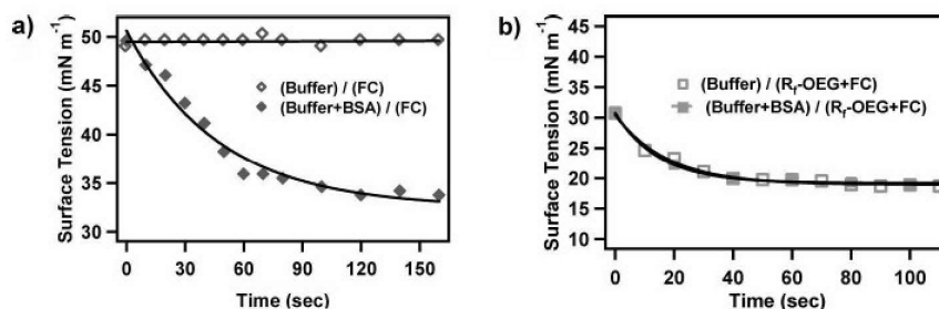
Figure 3. Graphs of surface tension versus time for BSA at an aqueous–fluorous interface without surfactant (◆) and at an interface that presented the R f -OEG surfactant (■). (a) BSA adsorbed to the aqueous–FC interface. The surface tension of the (buffer + BSA)/(FC) test droplet (◆) was lower than the surface tension of the (buffer)/(FC) control droplet (◇). (b) BSA did not adsorb to an interface that presented the R f -OEG surfactant. The surface tension of the (buffer + BSA)/(R f -OEG + FC) test droplet (■) matched the surface tension of the (buffer)/(R f -OEG + FC) control droplet (□).
