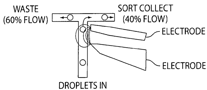
TEE JUNCTION
