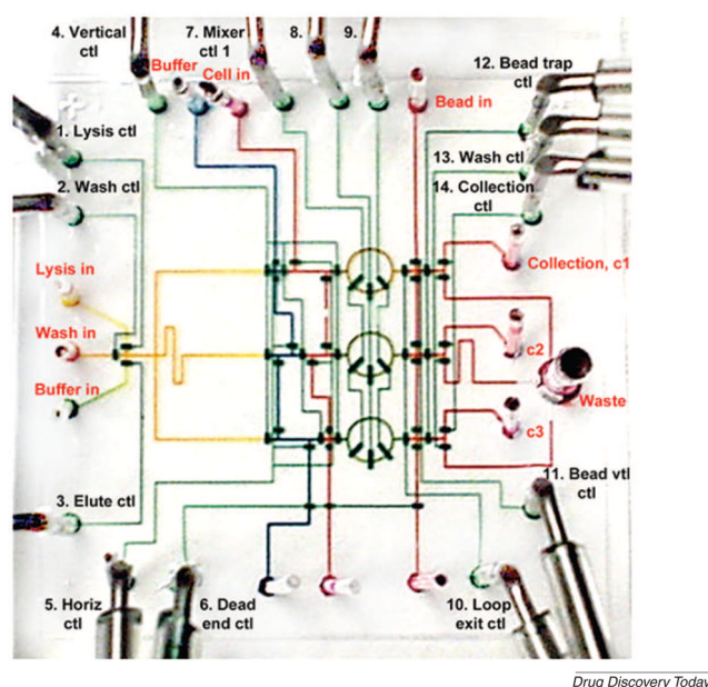
Figure 5. Microfluidic large-scale integration
