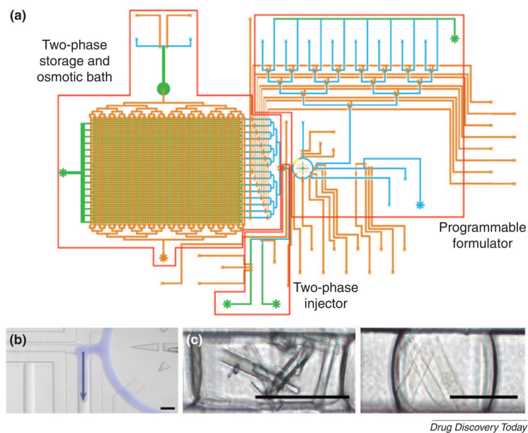
Figure 3. Protein crystallization in a microfluidic screening platform
