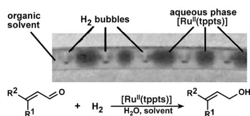
Figure 27. Catalytic multiphase reaction for the hydrogenation of unsaturated aldehydes performed by using alternating droplets. [191] Photograph of a capillary (diameter 750 \mu\text{m} ) containing alternating \text{H}_2 bubbles and aqueous droplets. The continuous phase is an organic solvent (either toluene or hexane) that contains the unsaturated aldehyde. Figure reprinted from reference [191].
