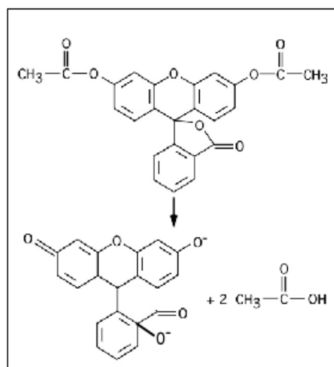
Figure 4.3: The conversion of fluorescein diacetate to fluorescein ( \lambda_{\text{ex}} = 490 nm, \lambda_{\text{em (max)}} = 518 nm). The reaction occurs via the cleavage of the ester bonds by pNB esterase.
