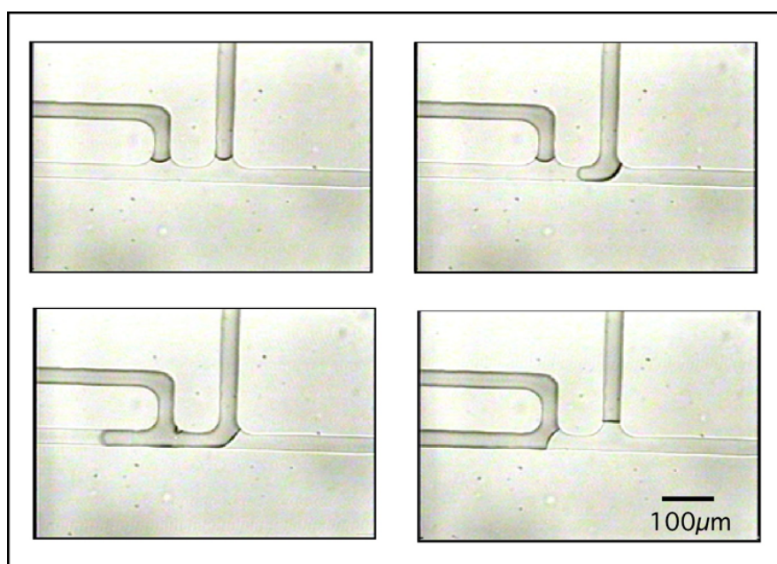
Figure 3.14: Dual-T microfluidic mixer. Water from the input channels enters the oil stream sequentially, mixing upon contact with each other, prior to being sheared into droplets.
