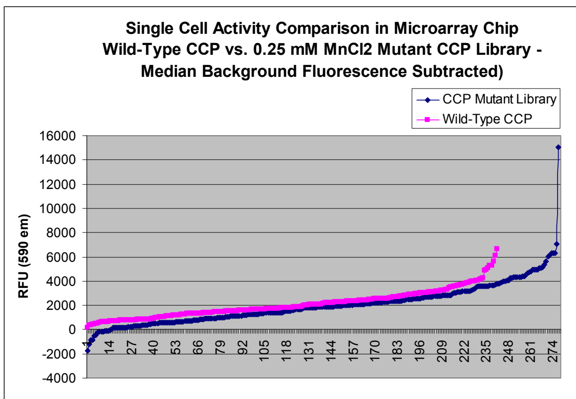
Figure 6.8: Single cell activity comparison for the wild-type CCP and the 0.25 mM MnCl 2 randomly mutagenized CCP library. Median background fluorescence levels were subtracted for each respective population.
