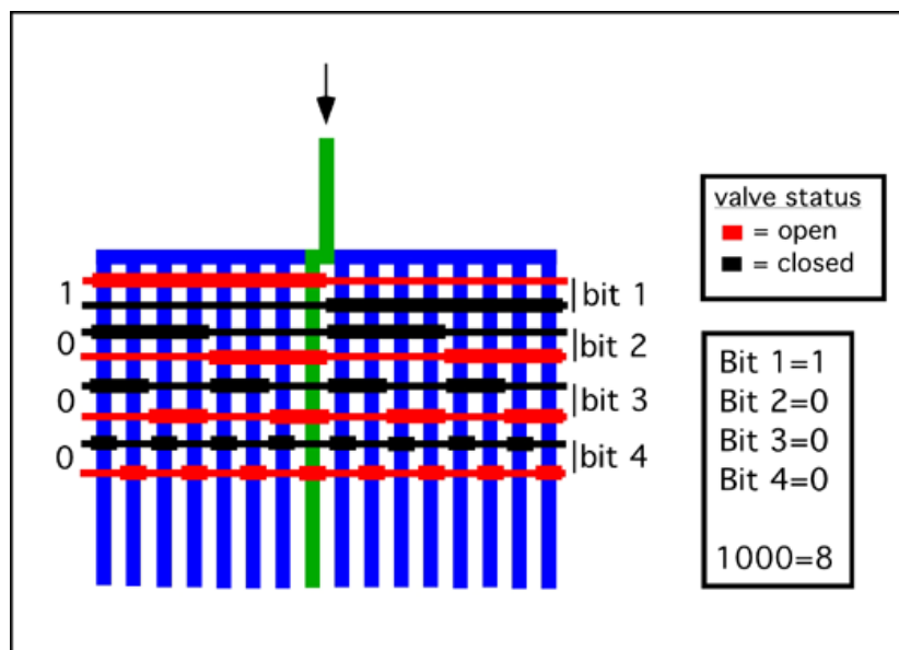
Figure 5.1: Multiplexor control in a multilayer elastomeric microfluidic device. Each open/closed valve configuration within the control layer opens a single flow channel. Valve closing pressure scales with the width of the control channel, allowing non-contiguous flow channels to be closed by the wide valves while flow channels under the narrow valves remain open.
