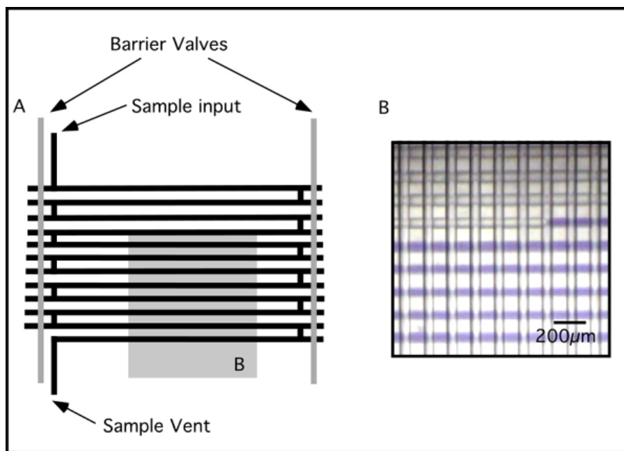
Figure 5.3: A) Detailed diagram of flow channel layout in high-density array region of serpentine chip illustrating flow path for sample loading when control layer barrier valves are closed. B) Illustration of sample loading mechanics in high-density array region using bromophenol blue. Vertical valves in photo are part of the non-actuated array sandwich valve (not visible in part A for simplification purposes).
