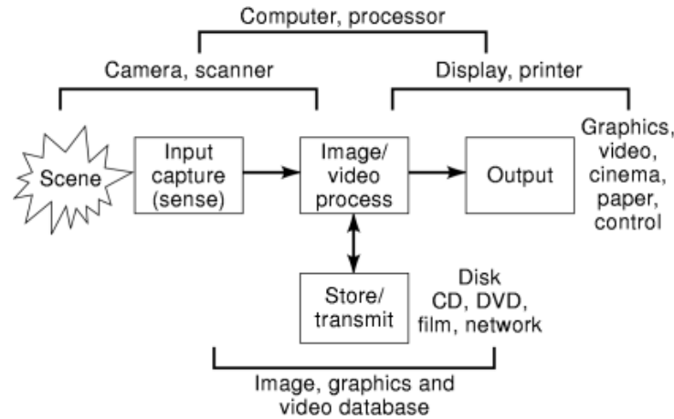
Fig. 1. Elements of image processing equipment (IPE) include the input block (for image/video capture/sensing), the processing block (for image/video computing), the storage/transmission block (for image/video database and compression), and the output block (for display or print of the images).
