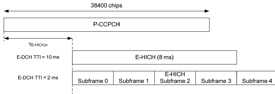
Figure 37: E-HICH timing
