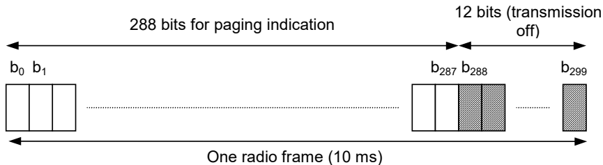
Figure 24: Structure of Paging Indicator Channel (PICH)
