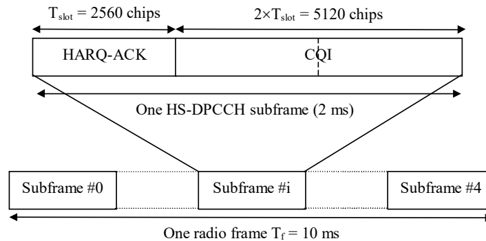
Figure 2A: Frame structure for uplink HS-DPCCH
