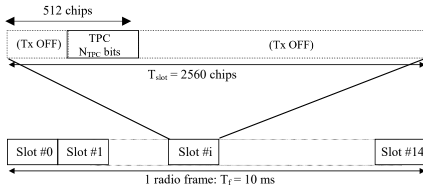
Figure 12B: Frame structure for F-DPCH
