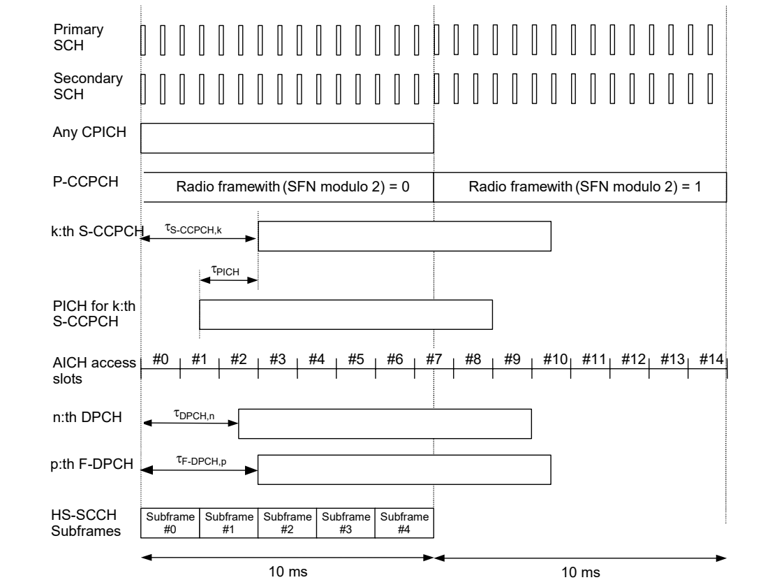
Figure 29: Radio frame timing and access slot timing of downlink physical channels
