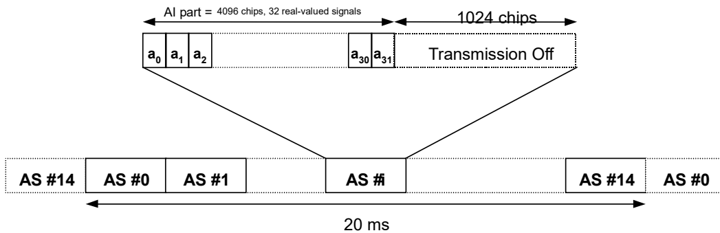
Figure 21: Structure of Acquisition Indicator Channel (AICH)
