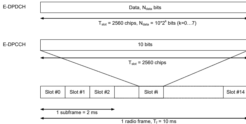
Figure 2B: E-DPDCH frame structure
