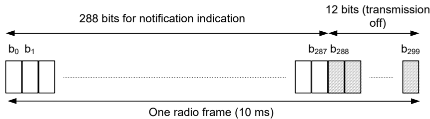
Figure 26D: Structure of MBMS Indicator Channel (MICH)
