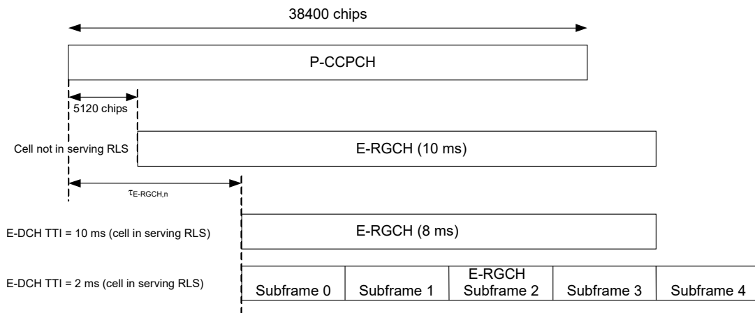
Figure 38: E-RGCH timing
