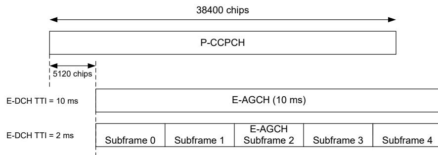
Figure 39: E-AGCH timing
