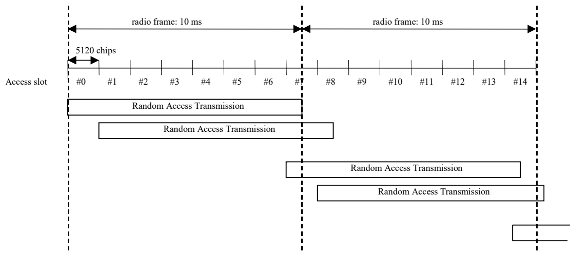
Figure 3: RACH access slot numbers and their spacing
