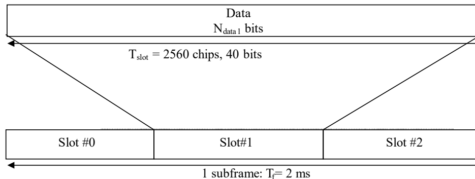
Figure 26A: Subframe structure for the HS-SCCH
