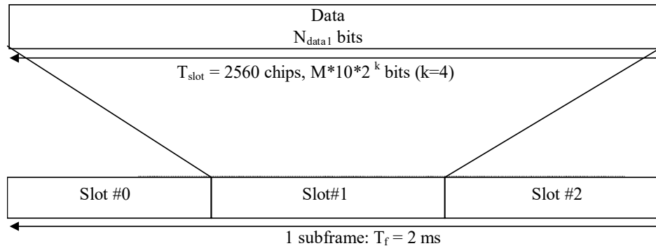
Figure 26B: Subframe structure for the HS-PDSCH
