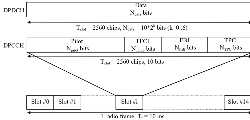
Figure 1: Frame structure for uplink DPDCH/DPCCH
