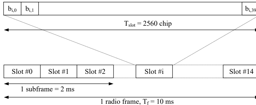
Figure 12A: E-RGCH and E-HICH structure
