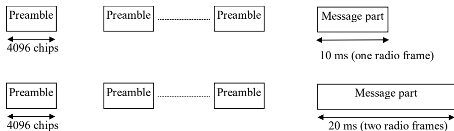
Figure 4: Structure of the random-access transmission
