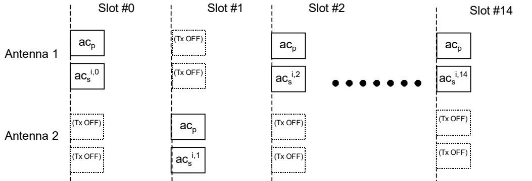
Figure 19: Structure of SCH transmitted by TSTD scheme
