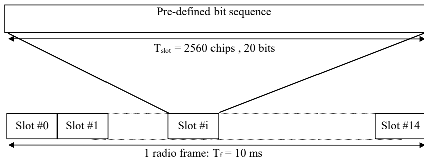
Figure 13: Frame structure for Common Pilot Channel
