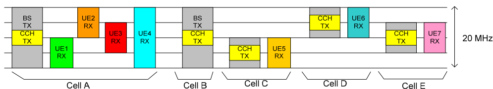
Figure 9.1.1: Variable bandwidth scenarios
