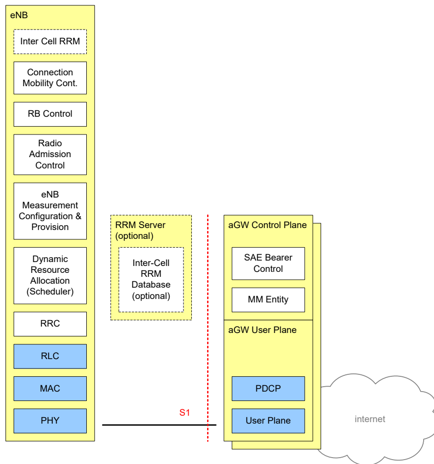
Figure 5.1: E-UTRAN Architecture
