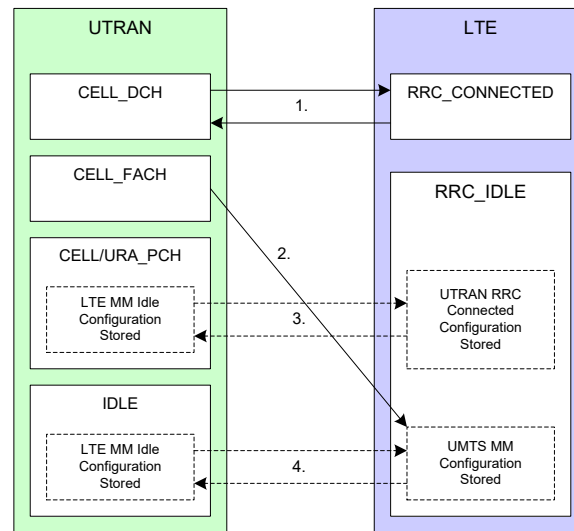
Figure 9: Handovers between E-UTRAN and UTRAN
