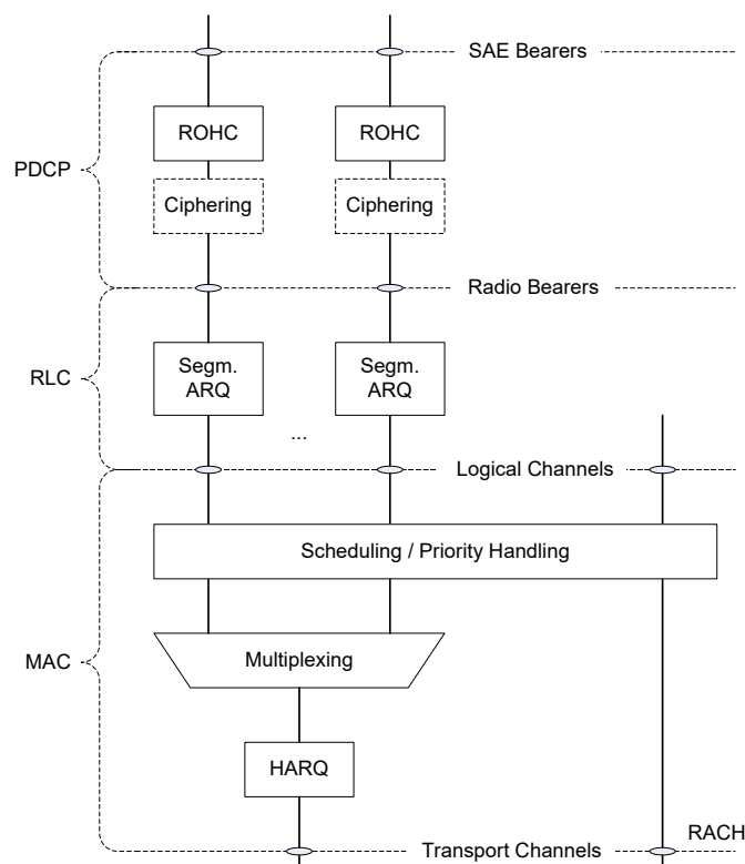
Figure 5.3.b: Layer 2 Structure for UL in UE
