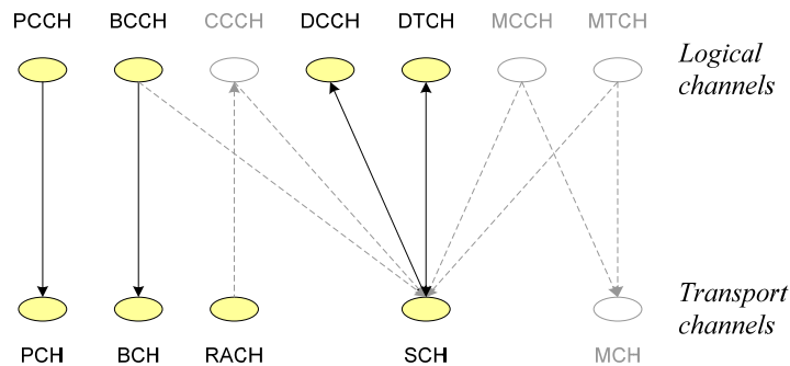
Figure 5.3.1.2: Mapping between logical channels and transport channels
