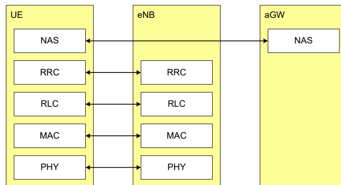
Figure 5.1.2: Control-plane protocol stack
