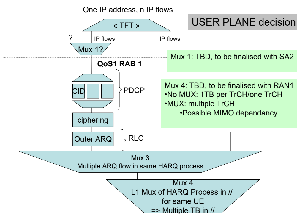
Figure C1: User Plane
