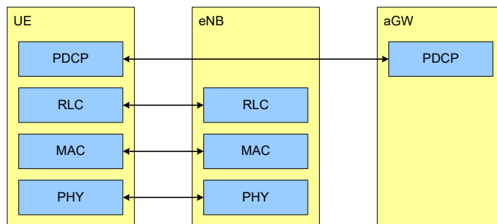
Figure 5.1.1: User-plane protocol stack
