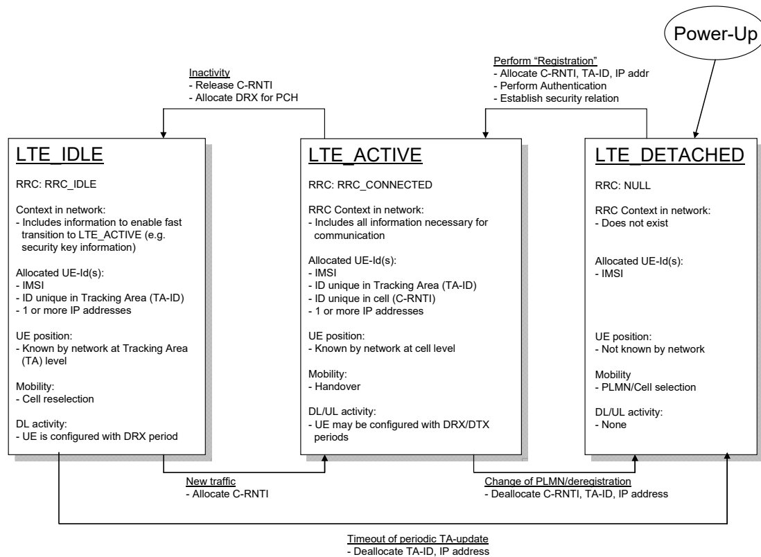
Figure 5.5.2: E-UTRAN RRC protocol states
