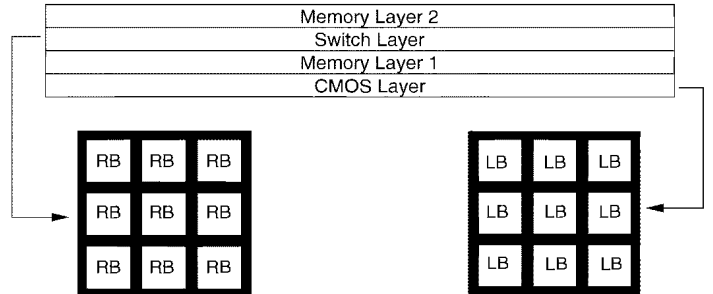
Fig. 20. Active layers of a 3-D-FPGA using proposed routing fabric. (RB: Routing block, LB: Logic block).
