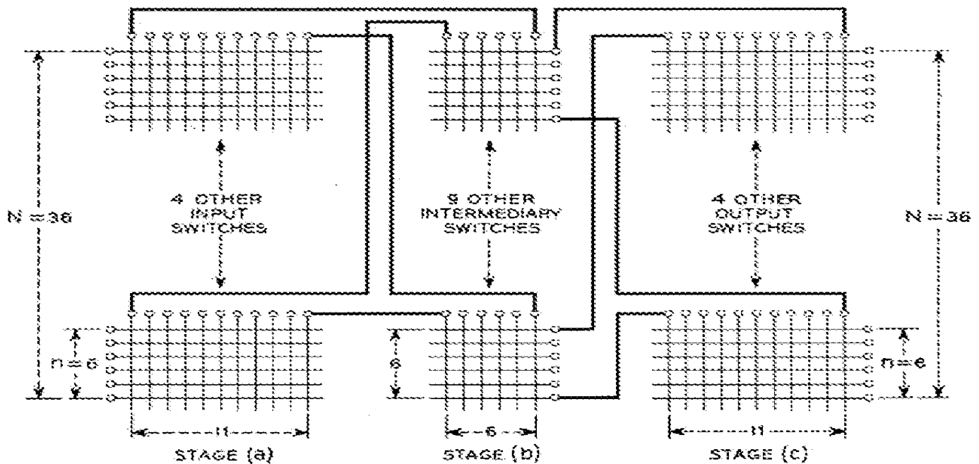
Fig. 3 — Three-stage switching array.
