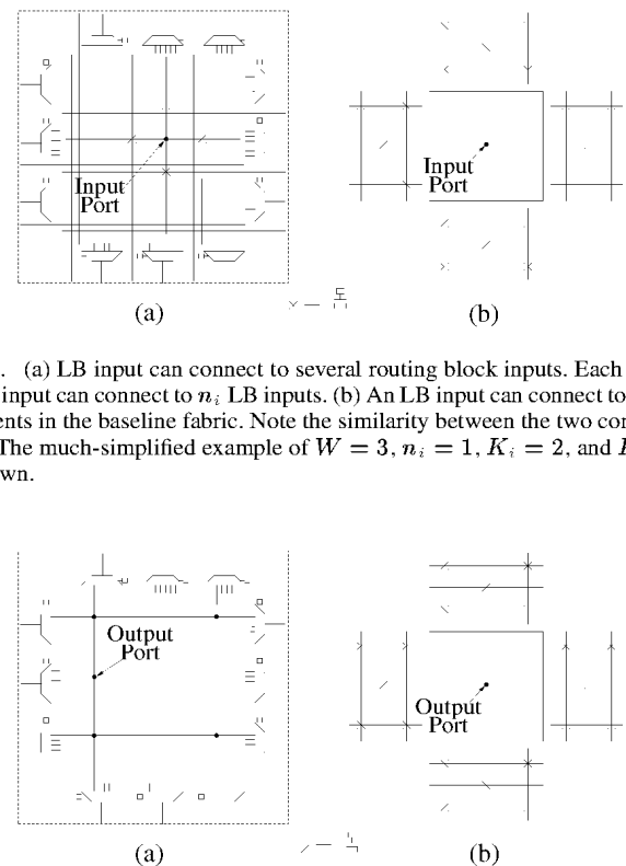
Fig. 10. (a) LB output can connect to n_o routing block MUX inputs on each side. (b) An LB output can connect to segments in the baseline fabric. Note the large difference between the two connectivities. The much-simplified example of W = 3 , n_o = 2 , K_i = 2 , and K_o = 1 is shown.
