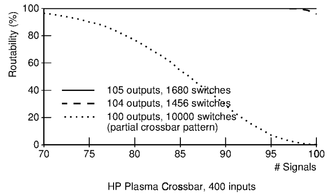
Figure 8: Routability Improvements made to the FLEX8000 and HP Plasma architectures.
