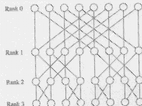
FIGURE 3-6 Butterfly network with 32 nodes. (Ullman [1984].)
