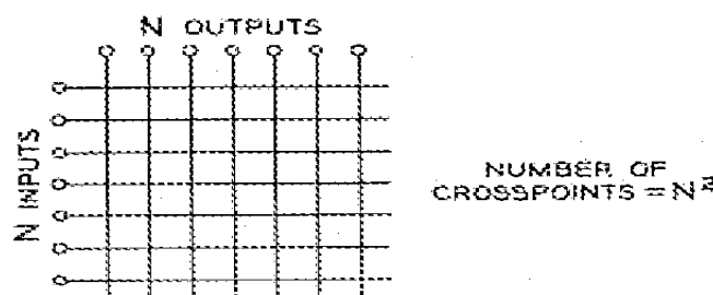
Fig. 1 — Square Array.
