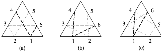
Fig. 13. (a) A 3-sided symmetric switch block. (b), (c) Two 3-sided isomorphic switch blocks of (a).
