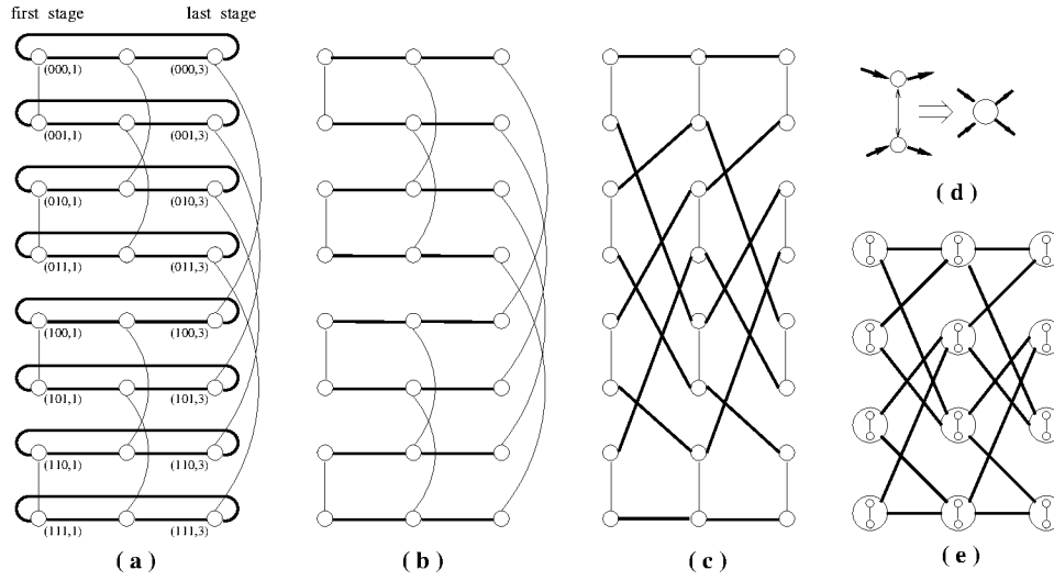
Figure 6: An embedding of \mathcal{K}_{8,8} into \mathcal{CCC}(n) .
