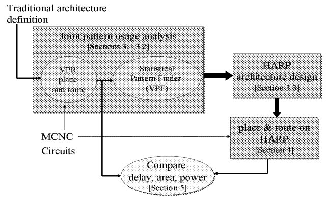
Figure 2: HARP-based Routing Architecture Design Flow.
