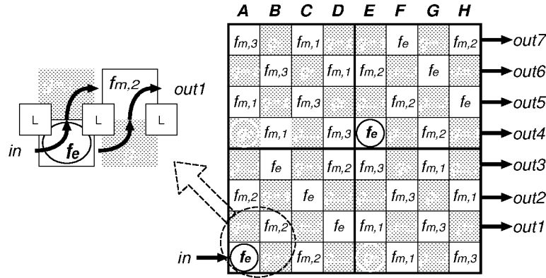
Fig. 5. An 8 \times 8 grid or supertile used for enumerating all two-turn paths.
