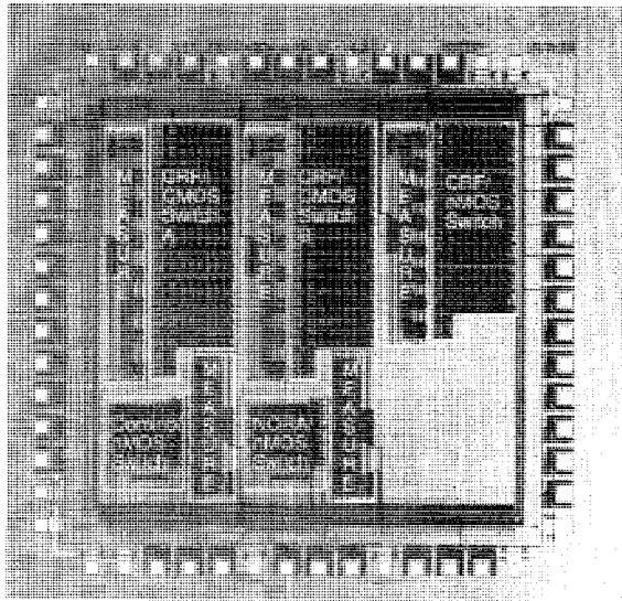
Fig. 21. Chip micrograph.
