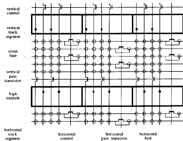
Fig. 1. Interconnect architecture.
