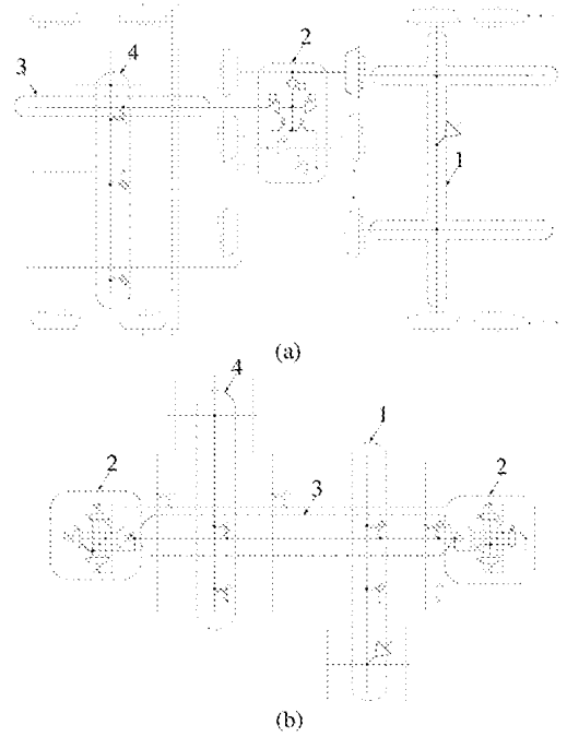
Fig. 15. Local connection in new fabric (a) and in baseline fabric (b). The numbers correspond to (1) output segment, (2) routing point/ switching point, (3) interconnect segment, and (4) input segment.
