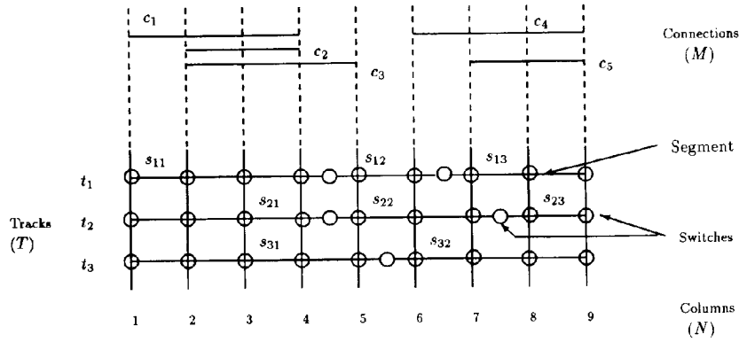
Fig. 3. An example of a segmented channel and a set of connections. M = 5 , T = 3 , N = 9 . Connections: c_1 , c_2 , c_3 , c_4 , c_5 . Segments: s_{11} , s_{12} , s_{13} , s_{21} , s_{22} , s_{23} , s_{31} , s_{32} .
