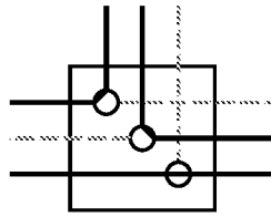
Figure 7: Single Crossover in p = 0 Case: the routed (highlighted) connections show an example where the physical network needs to have 1.5\times more wires in each channel than the design in order to be fully routable.
