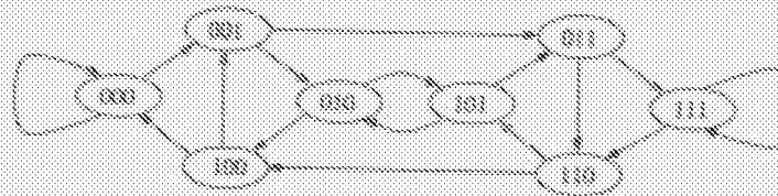
FIGURE 3-10 An 8-processor de Bruijn network.
