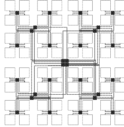
Figure 1: Floorplan of a 64-IP-BFT network.
