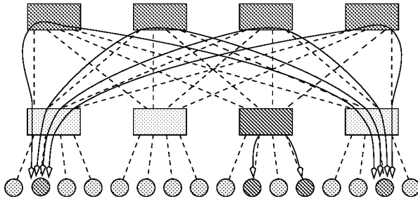
Figure 2. Routing on a 4-ary 2-tree.
