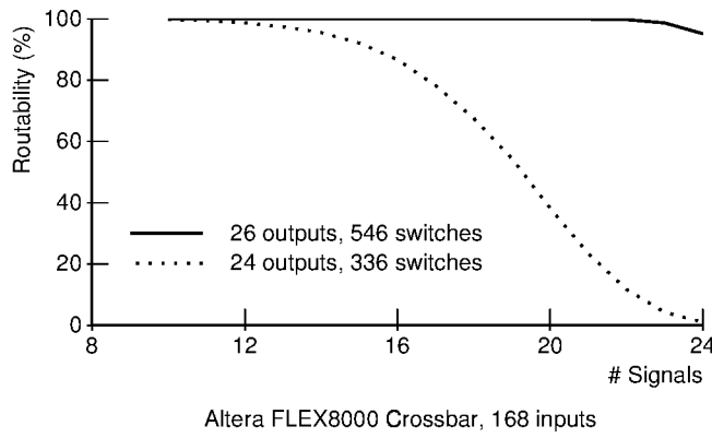
Figure 8: Routability Improvements made to the FLEX8000 and HP Plasma architectures.
