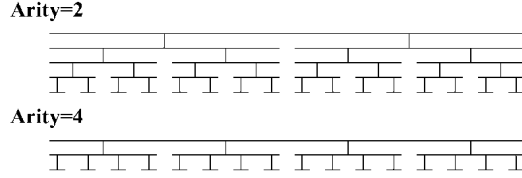
Fig. 15. Arity parameter on single row (column) channel in p = 0.5 MoT.
