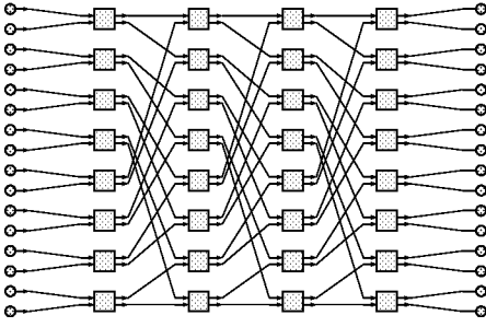
Figure 3: 16×16 Omega Network
