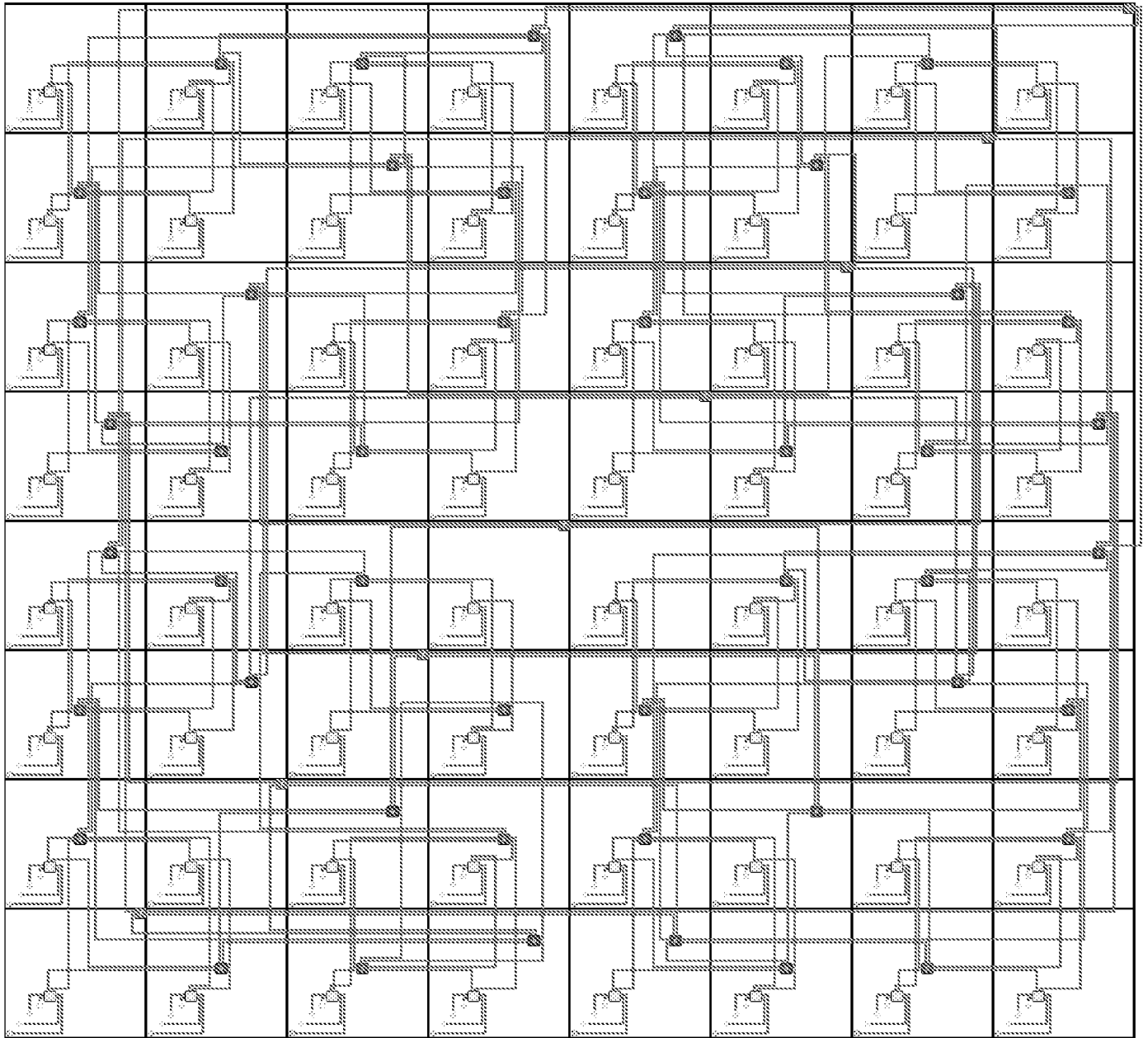
Figure 8: Fold-and-Squash Layout for 256-Node Rearranged Butterfly Fat-Tree
