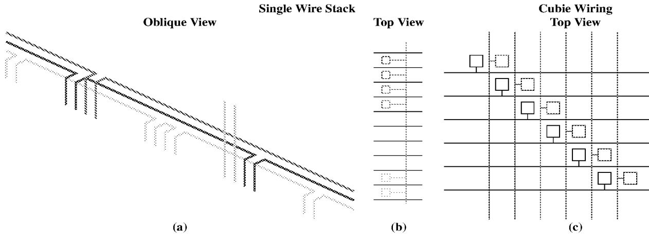
Figure 4: Wiring Pattern
