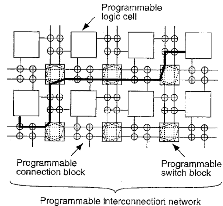
Fig. 1. FPGA architecture. An interconnection obtained after programming is indicated.
