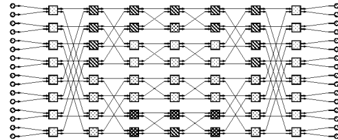
Figure 2: 16×16 Beneš Network
