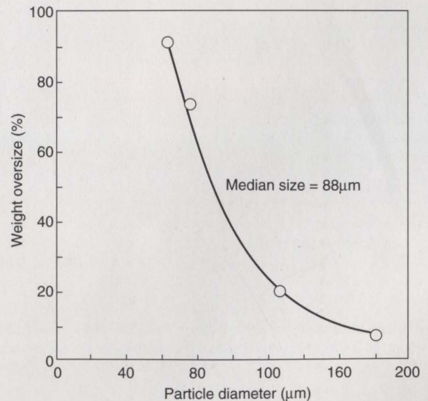
Fig. 4: Particle size distribution of mannitol powder.
