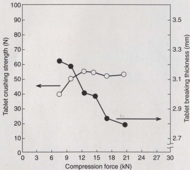
Fig. 2: Compression characteristics of granular mannitol.
