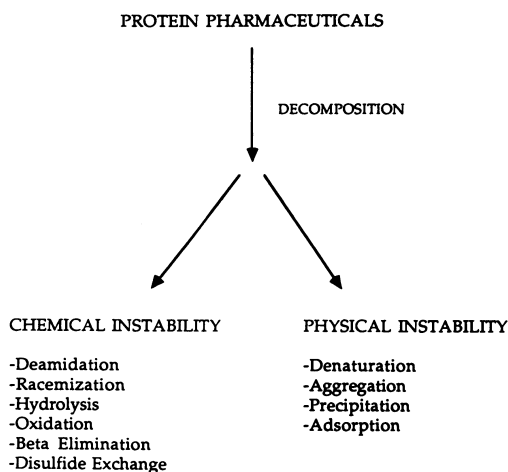
Fig. 1. Summary of the chemical and physical instability processes observed in protein pharmaceuticals.
