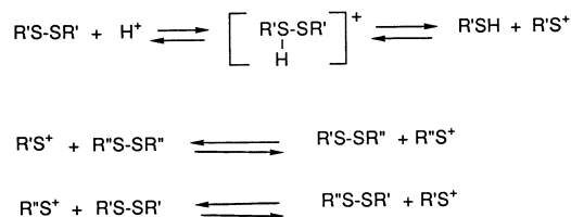
Fig. 6. Mechanism of disulfide exchange in acidic media.
