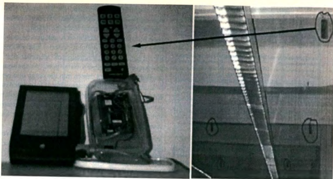
Figure 3. IR positioning prototype (left) and the array of positioning beacons in the GUV Lab (right).
