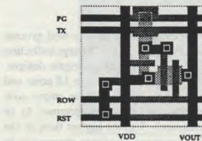
Fig. 10(a): Layout of single poly pixel
