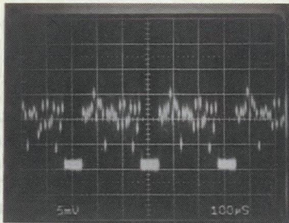
Fig. 13(a): FPN with crowbar off
