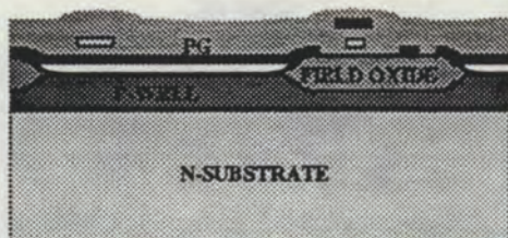
Fig. 5(a): Cross section of p-well pixel
