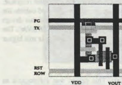
Fig. 9(a): Layout of tiny photogate pixel
