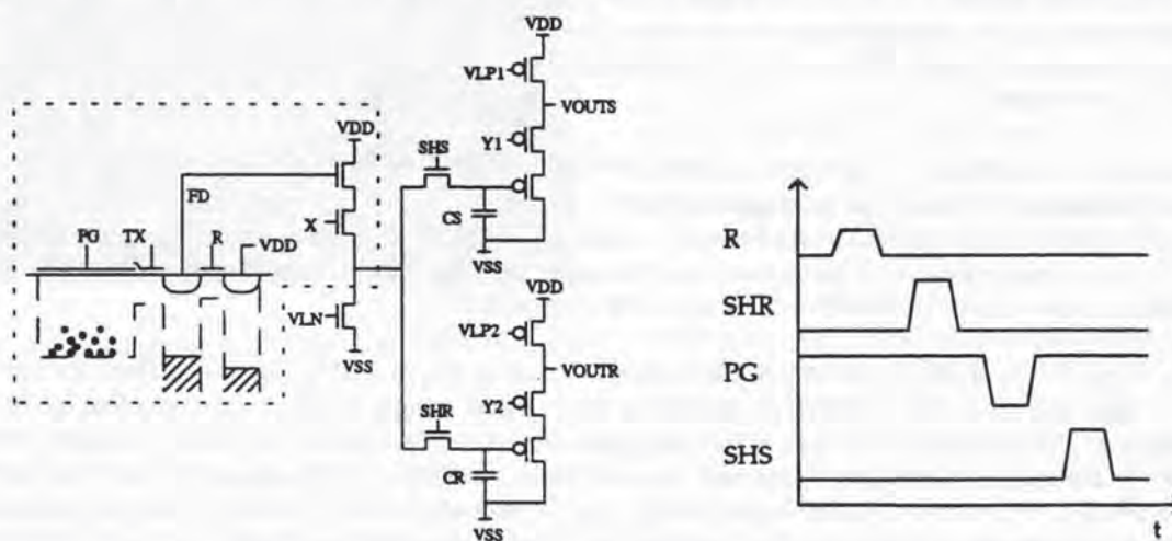
Figure 2(a): Schematic of readout circuit (b) timing for CMOS APS read out
