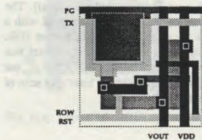
Fig. 8(a): Layout of square pixel
