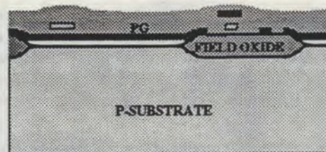
Fig. 5(b): Cross section of n-well pixel
