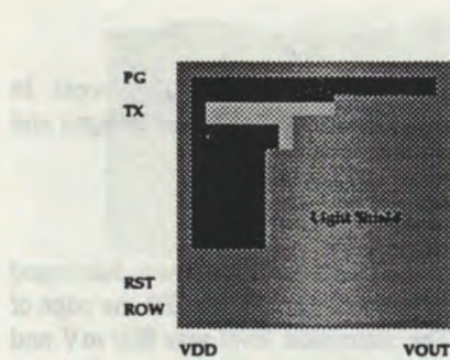
Fig. 7(a): Layout of light-shielded pixel
