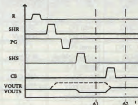
Fig. 12(b): Timing for crowbar readout
