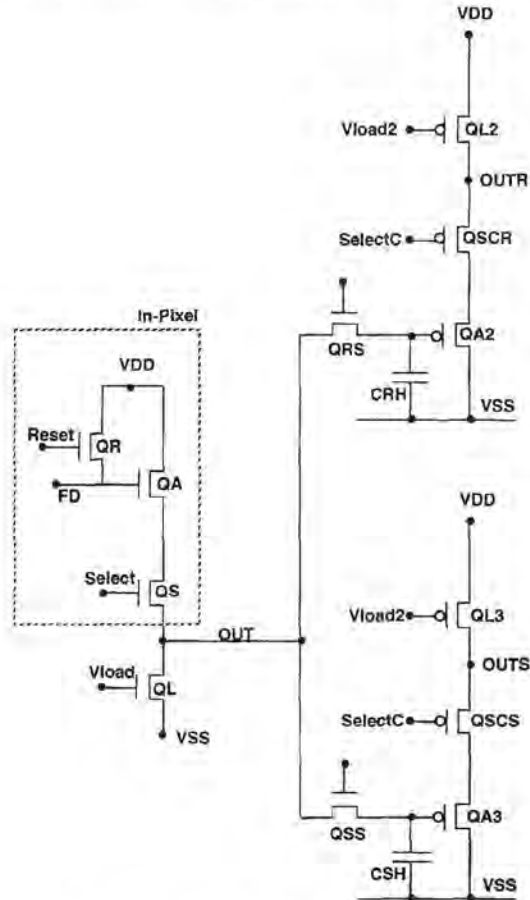
Figure 4: On-Chip Analog Signal Processor.
