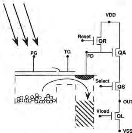
Figure 2: Double-Polysilicon Active Pixel.
