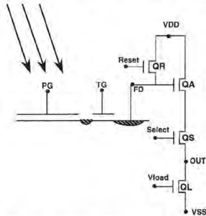
Figure 3: Single-Polysilicon Active Pixel.
