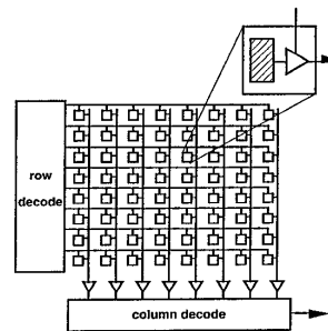
Figure 4: Active pixel sensor array.
