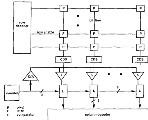
Figure 8: Per-column, single-slope A/D converter.
