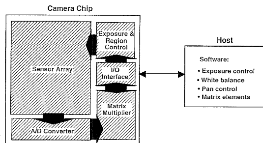
Figure 7: Camera on a chip hardware/software partitioning.
