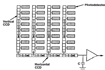
Figure 3: Interline transfer CCD.
