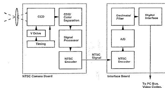
Figure 1: Conventional multimedia camera.
