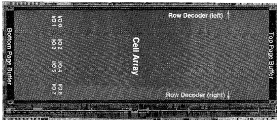
Figure 6: 128Mb NAND flash memory chip micrograph.
