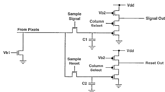
Figure 6: CDS fixed pattern noise reduction circuit.
