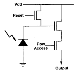
Figure 5: Active pixel circuit.
