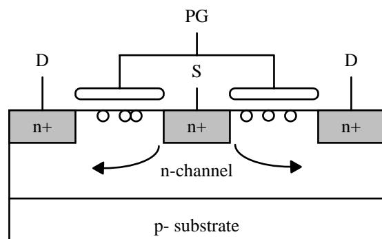
Fig. 6. Schematic illustration of Olympus CMD pixel
