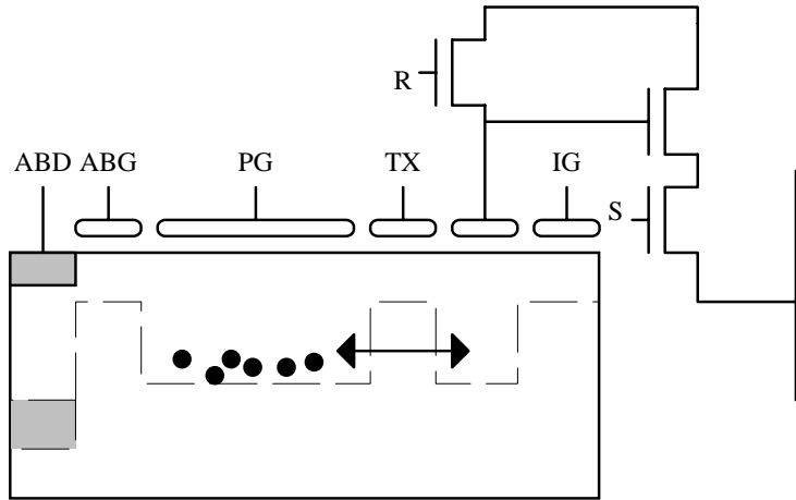
Fig. 10. JPL CMOS-compatible lateral APS.
