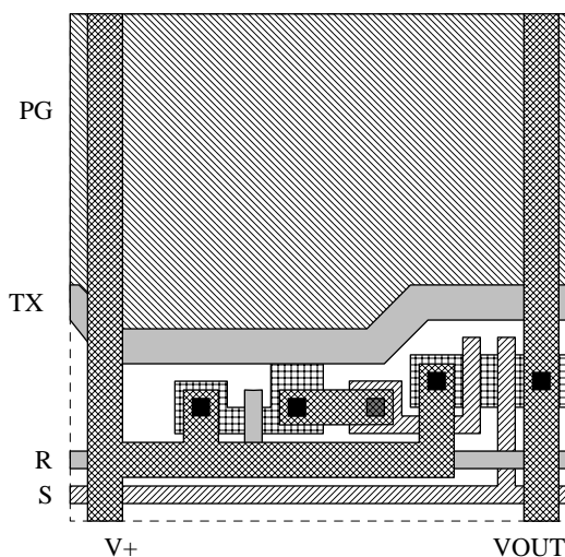
Fig. 3. Layout of a simple CMOS-compatible APS pixel.
