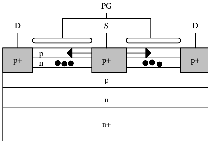
Fig. 7. Schematic illustration Texas Instruments' BCMD pixel. 15 \mu\text{V}/\text{e}^- with a 15 electron r.m.s. input referred noise level likely dominated by dark current shot noise. Readout is row-at-a-time into a bank of storage capacitors later scanned for serial output. The image sensor was configured as a hexagonally-packed array with on-chip color filters.
