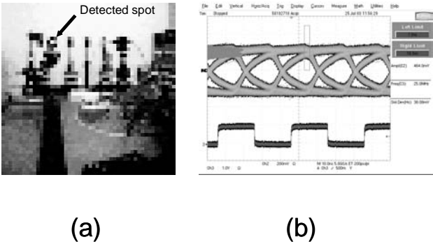
FIGURE 5.15 Experimental results of the smart CMOS image sensor. (a) Captured image, (b) 30-Mbps eye pattern for a wavelength of 830 nm.
