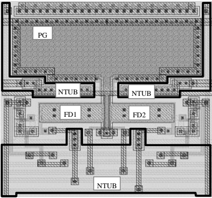
FIGURE 4.18 Pixel layout of the demodulated image sensor. The pixel size is 42 \times 42 \mu m^2 [349].
