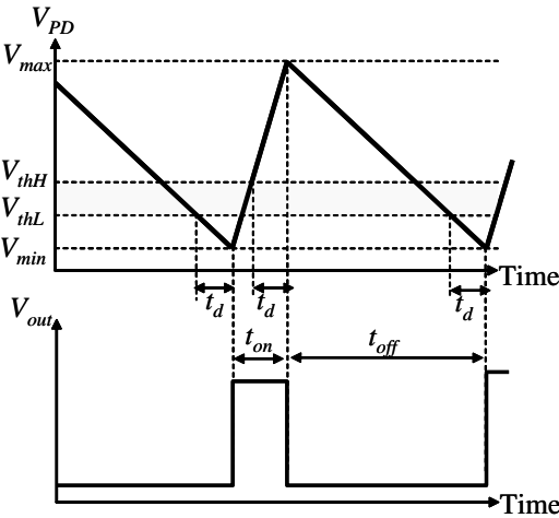
FIGURE 3.12 Time course of V_{PD} , taking the delay t_d into consideration.
