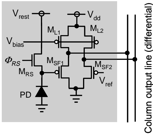
FIGURE 4.5 Differential APS. Illustrated after Ref. [278].
