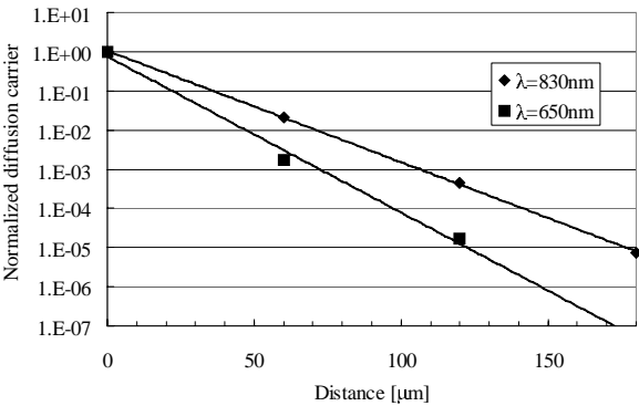
FIGURE 5.16 Measured amount of diffusion carriers on the pixels.
