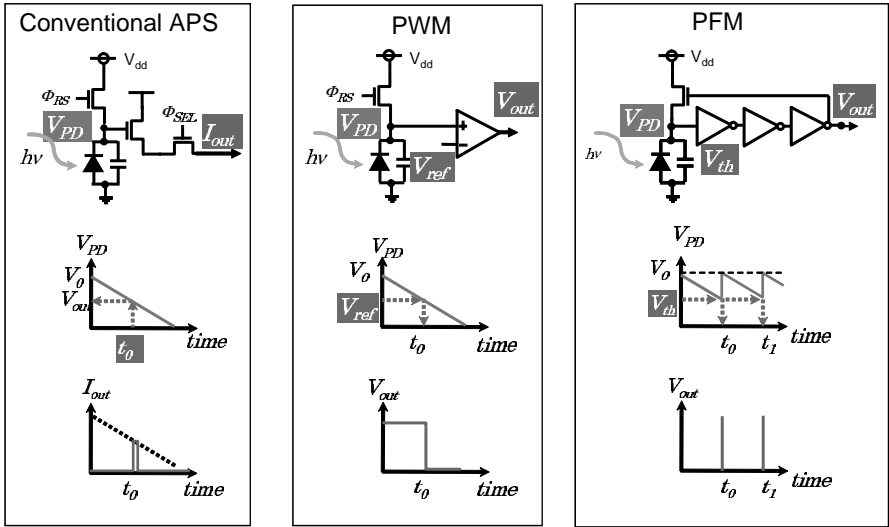
FIGURE 3.8 Basic circuits of pulse modulation. Left: conventional 3T-APS. Middle: pulse width modulation (PWM). Right: pulse frequency modulation (PFM).
