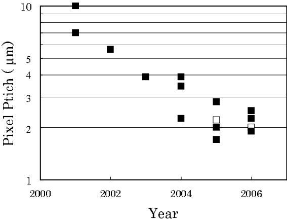
FIGURE 1.2 Trend of pixel pitch in 4T-APS type CMOS imagers. The solid and open squares show the pixel pitch for CMOS imagers and CCDs, respectively.
