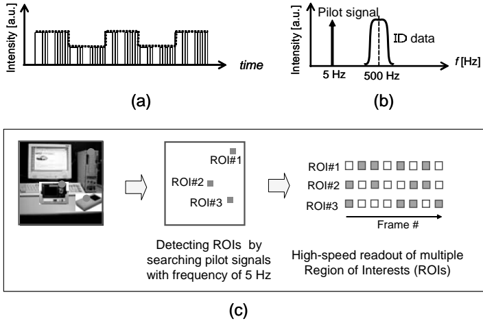
FIGURE 5.3 Method of detecting ID positions using a slow pilot signal. (a) Waveforms of pilot and ID signals, (b) power spectrum of pilot and ID signals, (c) procedure to obtain an ID signal using a pilot signal.
