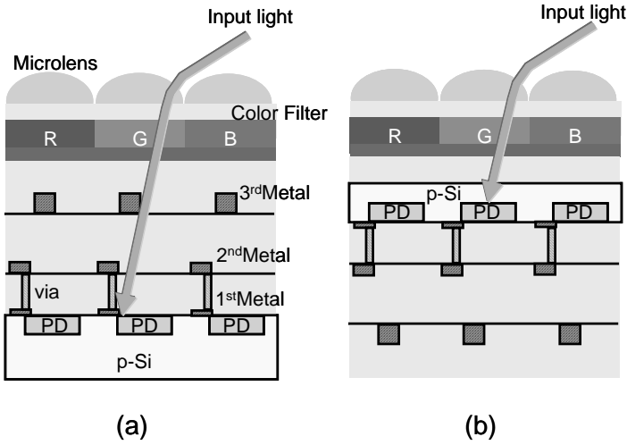
FIGURE 3.20 Cross-section of (a) a conventional CMOS image sensor and (b) a back-illuminated CMOS image sensor.
