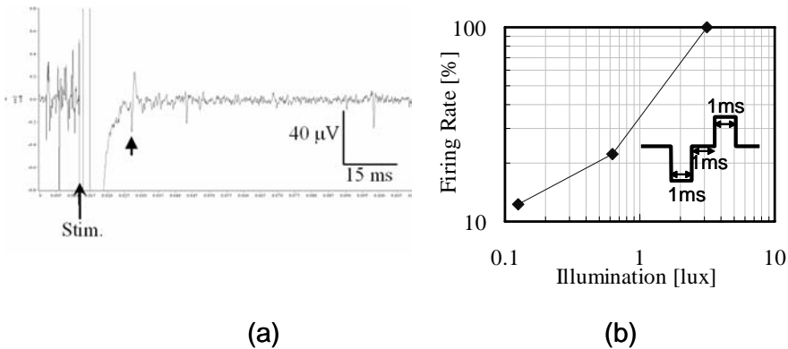
FIGURE 5.46 Experimental results of in vitro stimulation using the PFM photosensor. (a) Example obtained waveform obtained. (b) Firing rate as a function of input light intensity [208].
