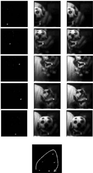
FIGURE 4.21 Demonstration of marker tracking. The images are placed in order of time from top to bottom. Left column: modulated light pattern extracted by the sensor. Middle column: output from the modulated light and background light. Right column: output from only the background light. The bottom figure shows the moving trace of the marker. For convenience, the moving direction and the track of the LED are superimposed [343].
