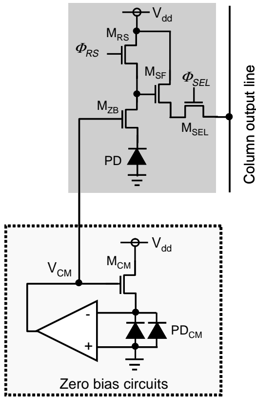
FIGURE 4.2 Near zero bias circuits for reducing dark current in an APS [279].
