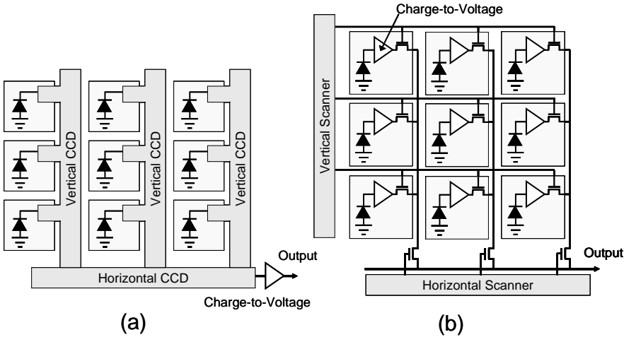
FIGURE 2.38 Conceptual illustration of the chip structure of (a) CCD and (b) CMOS image sensors.
