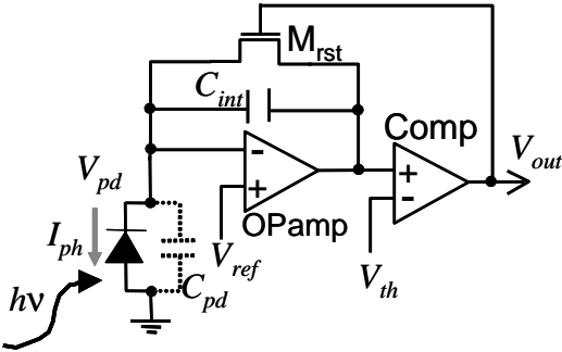
FIGURE 3.17 PFM pixel circuit with constant PD bias [199]. OPamp: operational amplifier, Comp: comparator.
