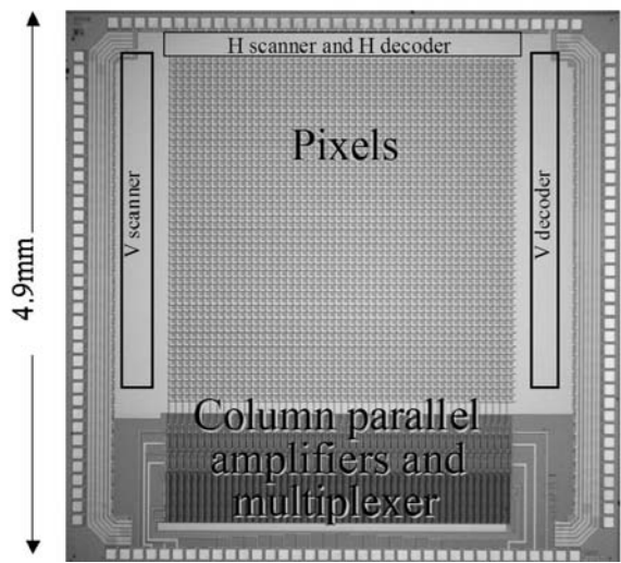
FIGURE 5.14 Microphotograph of a smart CMOS image sensor for an indoor optical wireless LAN.
