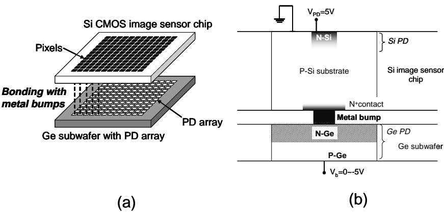
FIGURE 3.22 Smart CMOS image sensor that can detect in both the visible and eye-safe regions. (a) Chip structure, (b) cross-section of the sensor [242].
