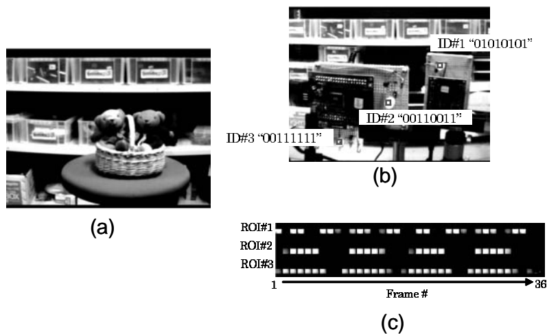
FIGURE 5.8 Images taken by a smart CMOS image sensor for optical ID tags. (a) Normal image, (b) ID detection, (c) 36-frame ROI images/ID (in one frame for a normal image).
