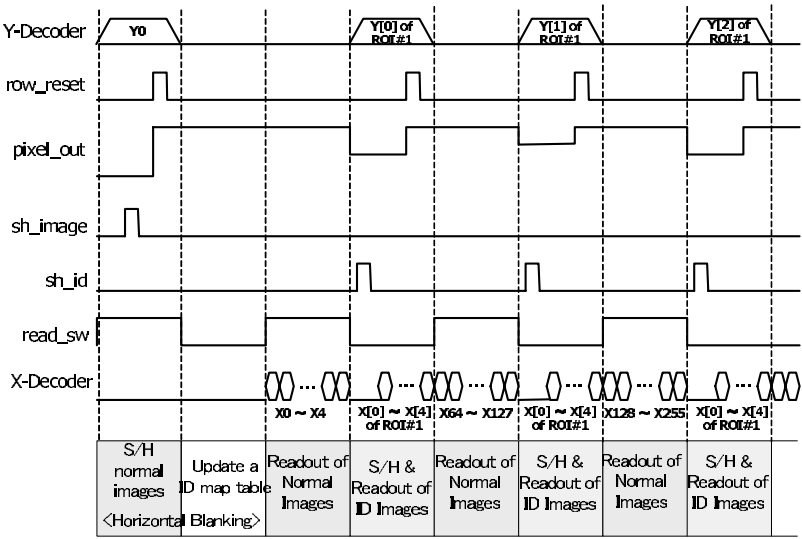
FIGURE 5.6 Timing chart for high-speed readout of multiple ROIs.
