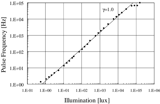
FIGURE 3.11 Experimental output pulse frequency dependence on the input light intensity for the PFM photosensor in Fig. 3.10 .
