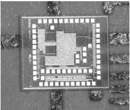
FIGURE 3.21 PFM photosensor fabricated using SOS technology [203].
