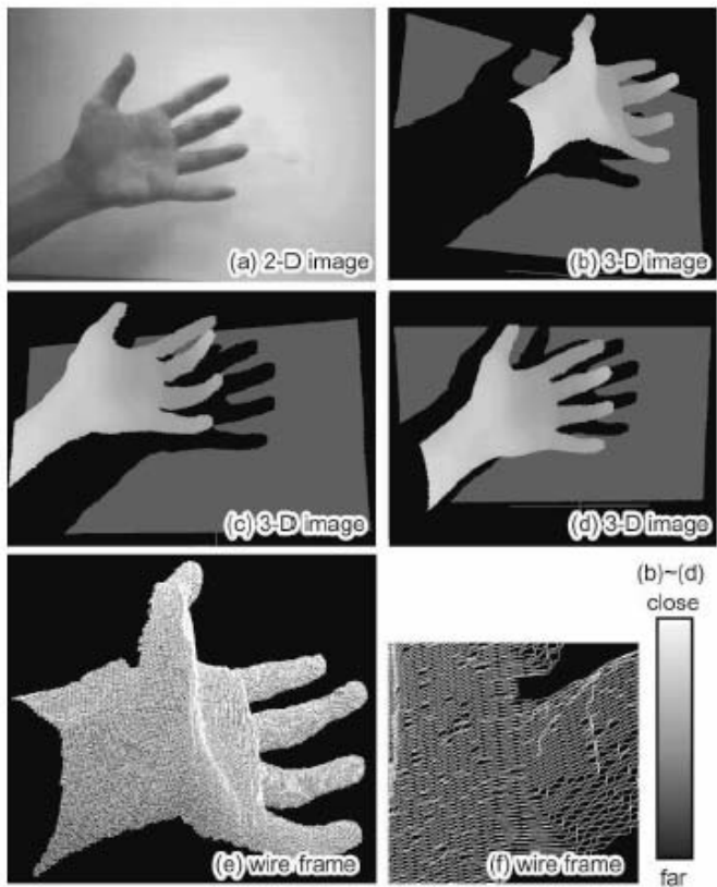
FIGURE 4.23 Examples of images taken by a 3D range finding image sensor developed by Y. Oike et al. [356]. Courtesy of Dr. Y. Oike.
