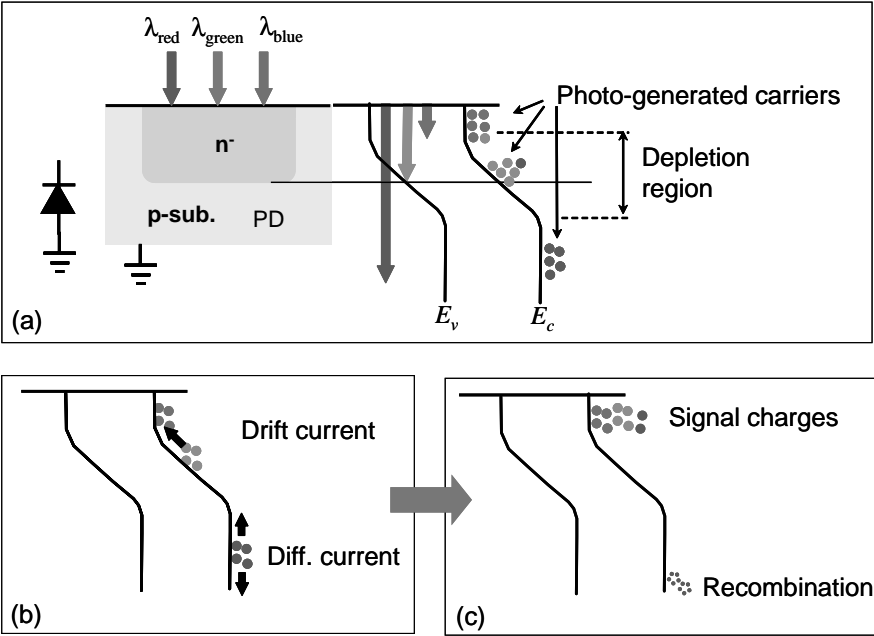
FIGURE 2.17 Behavior of photo-generated carriers in a PD.
