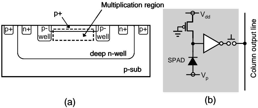
FIGURE 4.6 Basic structure of (a) an APD in standard CMOS technology and (b) a circuit for the Geiger mode APD in a pixel. The PMOS connected to V_{dd} acts as a resistor for quenching process. V_p is a negative voltage value that forces the PD into the avalanche breakdown region. SPAD: single photon avalanche diode. Illustrated after Ref. [98].
