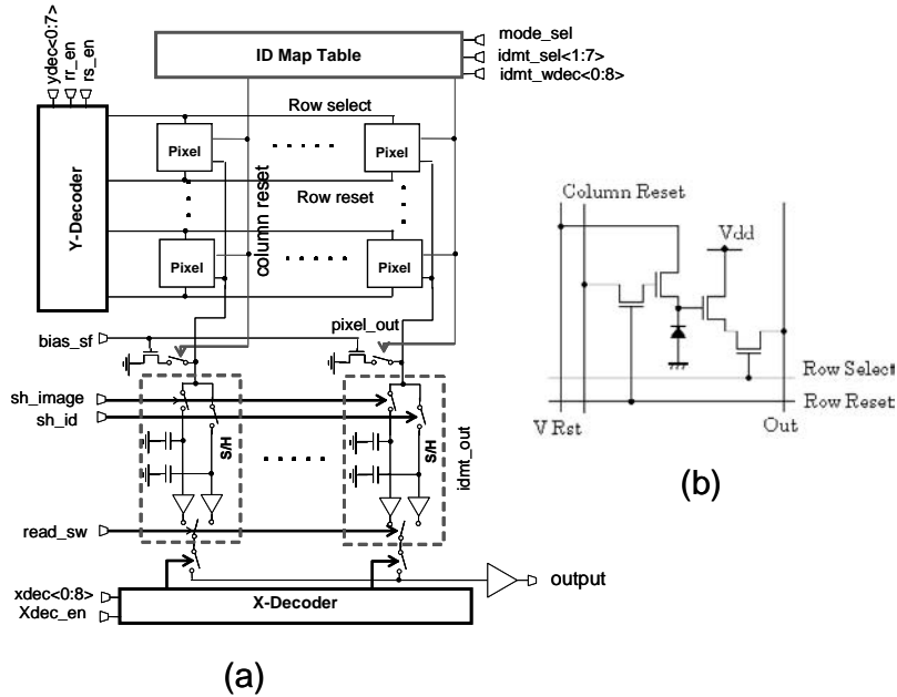
FIGURE 5.5 (a) Block diagram of a smart CMOS image sensor for fast readout of multiple ROIs. (b) Pixel circuits.
