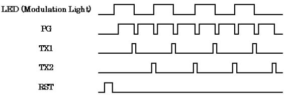
FIGURE 4.19 Timing chart of the demodulation image sensor [348]. PG: photogate, TX: transfer gate, RST: reset.
