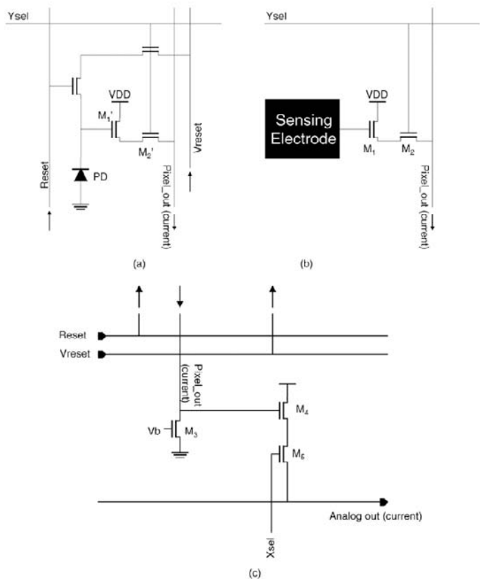
FIGURE 5.19 Circuits of a smart CMOS image sensor for optical and potential dual imaging for (a) a light-sensing pixel, (b) a potential-sensing pixel, and (c) a column unit.
