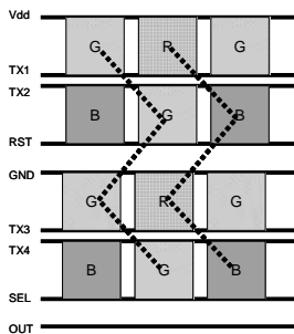
FIGURE 2.37 Pixel sharing with a zigzag placement of RGB pixels [156].
