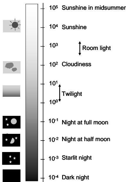
FIGURE B.1 Typical levels of illuminance for a variety of lightning conditions [6, 143].
