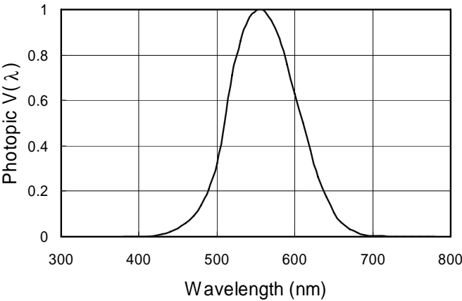
FIGURE B.2 Photopic eye response.
