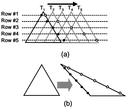
FIGURE 2.39 Illustration of the origin of a rolling shutter. (a) A triangle-shape object moves from left to right. (b) The original image is distorted.
