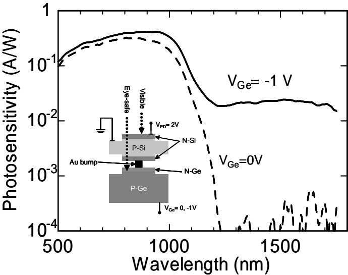
FIGURE 3.23 Photonsensitivity curve as a function of input light wavelength. The bias voltage V_b of the Ge PD is a parameter. The inset shows the test structure for this measurement [242].
