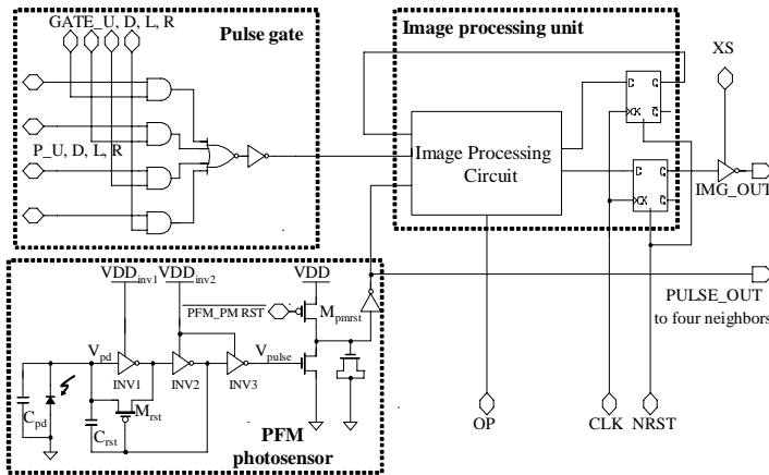
FIGURE 5.43 Pixel schematic of a capacitive feedback PFM with image preprocessing functions [209].
