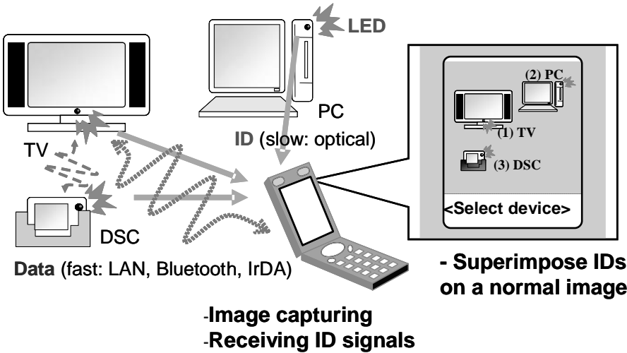
FIGURE 5.2 Concept of OptNavi. A dedicated smart CMOS image sensor can detect and decode optical IDs from home electronic appliances. The decoded results are superimposed on the image taken by the sensor.
