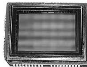
Sony ICX483AQA 10.14-megapixel APS-C (23.4 × 15.6 mm) CCD from digital camera Sony α DSLR-A200 or DSLR-A300, sensor side
