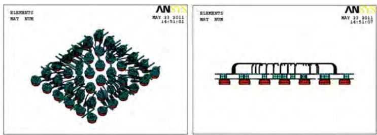
Fig. 8.32 The interconnects of 40 pin MCSP with wire bonding
