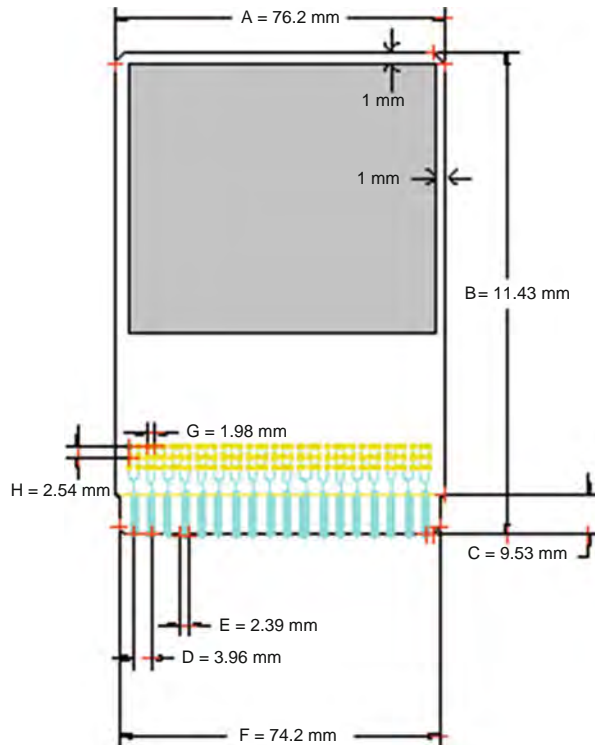
Fig. 7.6 PCB for packages <27.0 mm long 74.20 \times 74.20 (mm 2 ) buried planes
