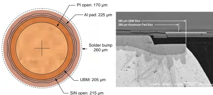
Fig. 2.17 Top view of an example UBM, PI repassivation, passivation and aluminum pad stack up, and enclosure relationship. On the right is a FA image of an early TMCL fail on the 8 \times 8 array with UBM size (260 \mu\text{m} ) larger than the aluminum pad size (250 \mu\text{m} ). The extension of UBM beyond perimeter of aluminum pad is thought as the root cause of the early failure
