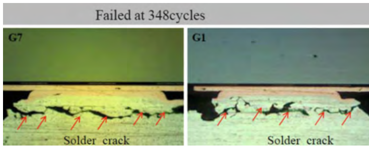
Fig. 10.64 Solder joint thermal cycling failure of 2Cu1Pi design
