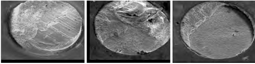
Fig. 10.1 Failure modes observed from shear test [2]
