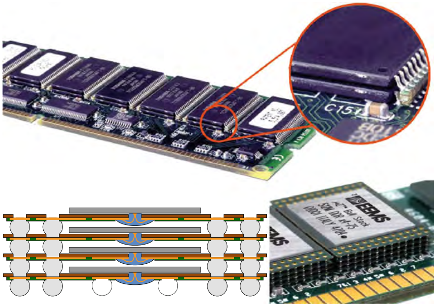
Fig. 4.6 Top: TSOP PoP on a memory module. Bottom: schematic cross section of Tessera \mu Z^{\text{TM}} ball PoP and actual stack up of \mu Z^{\text{TM}} ball PoPs on a single in-line memory module (SIMM)
