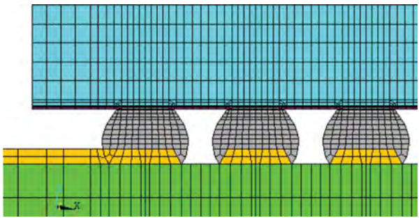
Fig. 10.17 Cross section of 5 \times 5 WLCSP mounted on the PCB board
