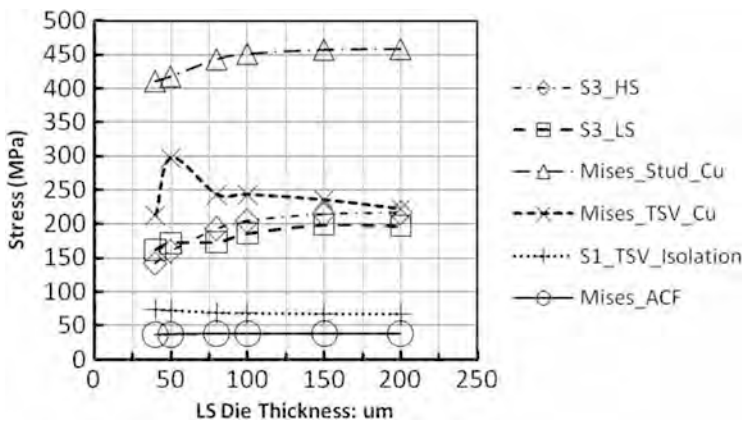
Fig. 6.24 The stresses of HS, LS, Cu stud, TSV Cu, isolation layer, and ACF layer versus LS die thickness
