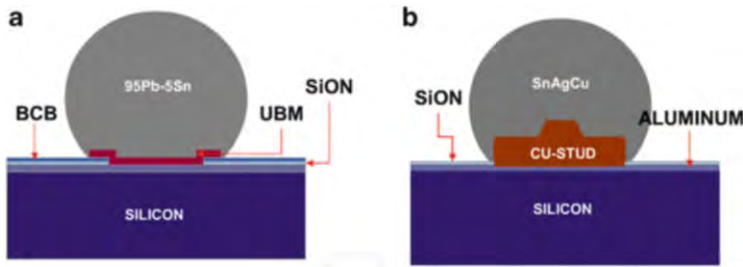
Fig. 5.13 Power WLCSP bumping options: UBM versus Cu stud. (a) Regular power WLCSP, (b) copper stud bumping with solder
