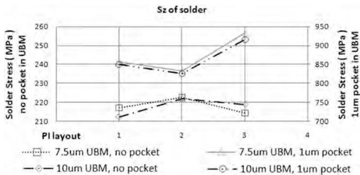
Fig. 10.47 Z component peeling stress comparison with different design parameters in drop test
