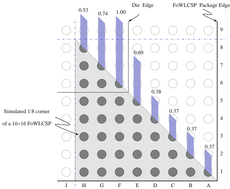
Fig. 3.13 Normalized inelastic strain energy density along the diagonal of a 16 × 16 bump fan-out WLP package with a 3 × 3 mm, 0.5 mm pitch silicon die size embedded in the middle of the package. Higher inelastic strain energy density prompts earlier TMCL fails
