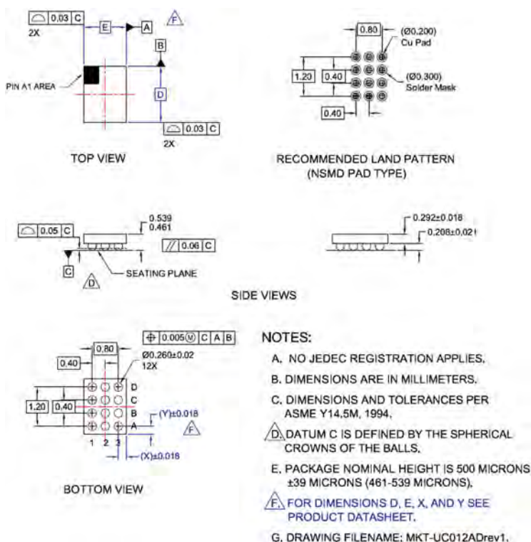
Fig. 8.1 A typical 3 \times 4 WLCSP layout
