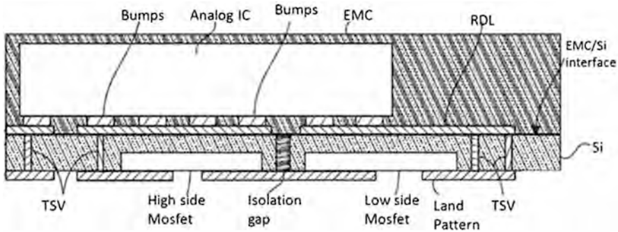
Fig. 6.35 A schematic concept of stack analog IC die with two Mosfet power device wafer
