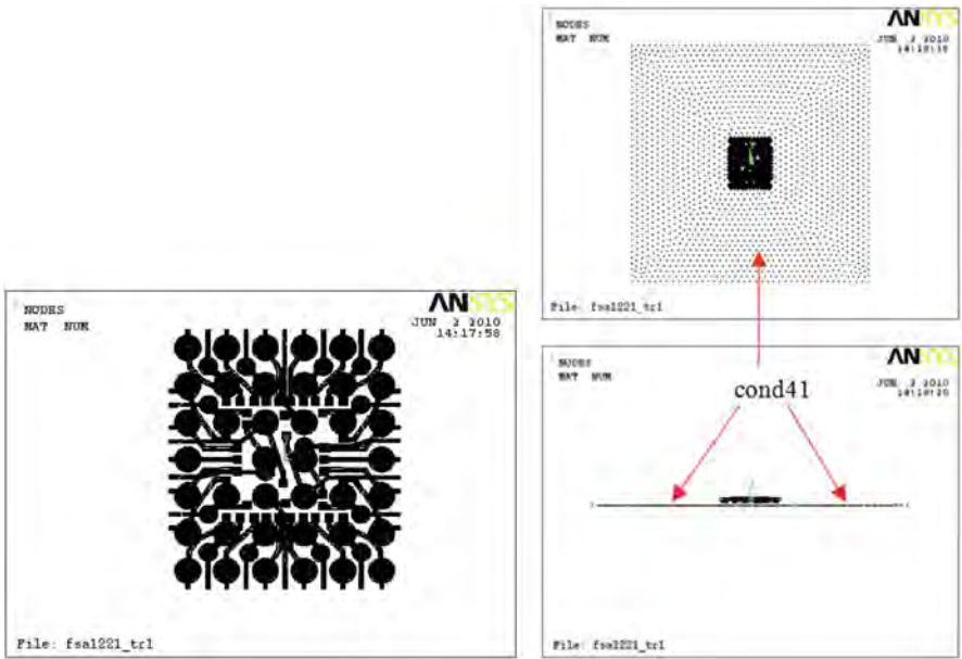
Fig. 8.30 The components cond1-cond40 (pin 1-pin 40) and cond41
