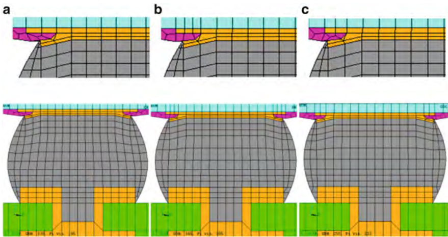
Fig. 10.56 Finite element model 2Cu1Pi WLCSP with different UBM diameters: (a) ØUBM = 230 µm, (b) ØUBM = 245 µm, and (c) ØUBM = 255 µm
