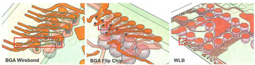
Fig. 3.8 Electrical modeling on wire bond BGA, flip chip BGA, and eWLB fan-out WLCSP. Chip to package interconnections are highlighted in red squares/rectangle
