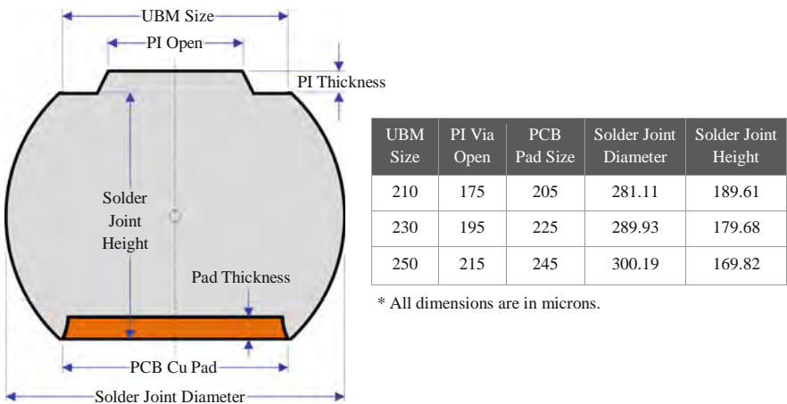
Fig. 9.5 UBM/pad size-dependent solder joint size for typical 0.4 mm pitch WLCSP with 250 \mu\text{m} diameter solder balls reflowed
