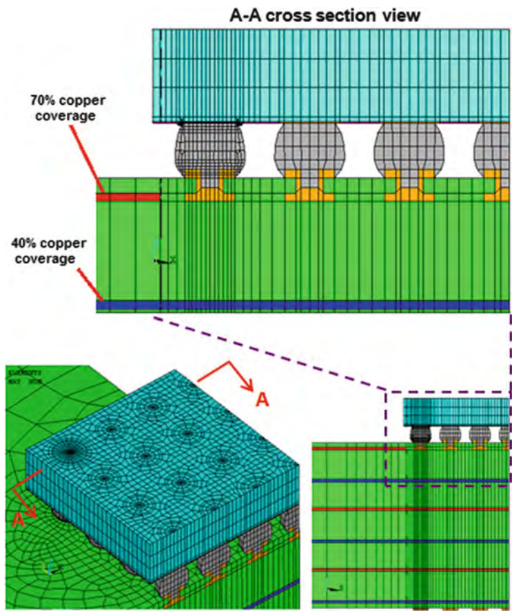
Fig. 10.39 The finite element model for TMCL
