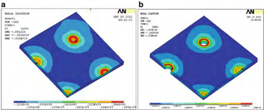
Fig. 6.26 The tensile stress S1 of HS and LS die at reflow: (a) the tensile stress S1 of the HS die at reflow (max 345 MPa) and (b) the tensile stress S1 of the LS die at reflow (max 378 MPa)
