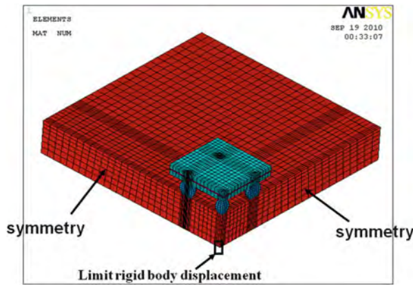
Fig. 6.25 The quarter model of the wafer-level power stack die package mounted on a PCB
