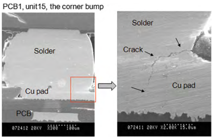
Fig. 10.34 Drop test failure mode
