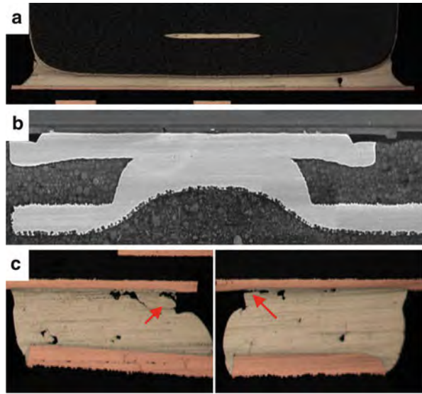
Fig. 5.37 Cross sections of a 7 \times 7 daisy chain module post 1,000 TMCL cycles: (a) cross section through a passive showing no solder crack; (b) cross section show no damage to the buried via connecting the module; (c) two corner module/PCB solder joints show signs of crack initiation after 1,000 cycles
