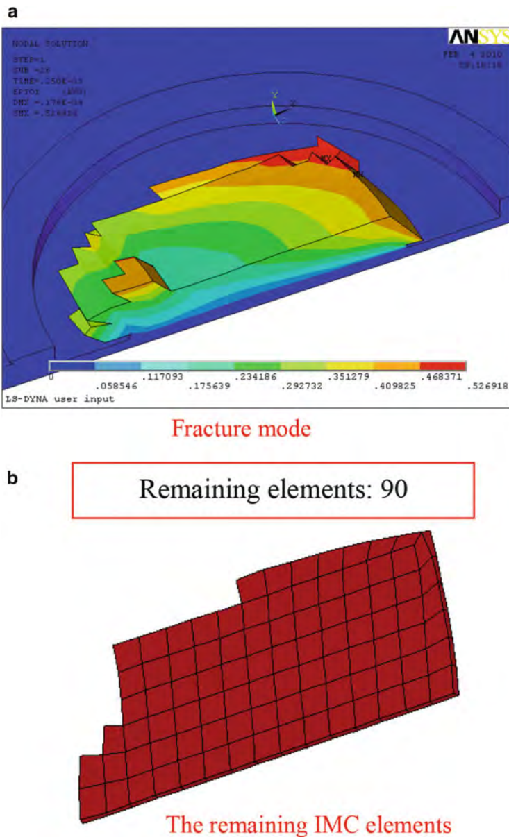
Fig. 10.12 Fracture surface (a) and remaining IMC (b) at 600 mm/s
