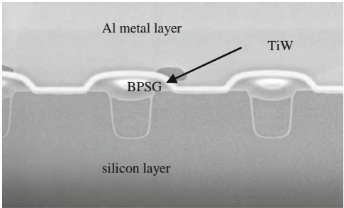
Fig. 5.18 Local structure under Al metal
