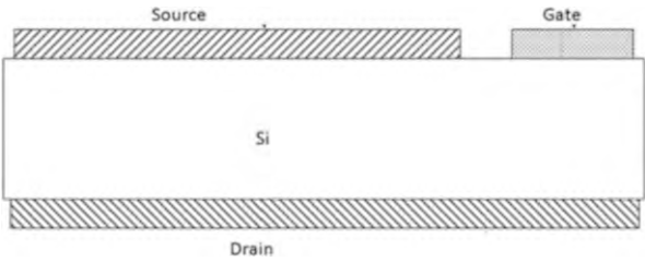
Fig. 5.10 The metal layout of a VDMosfet
