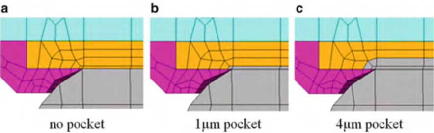
Fig. 10.51 The finite element model cross section of the WLCSP with different pocket depths in UBM: (a) no pocket, (b) 1 μm pocket, and (c) 4 μm pocket
