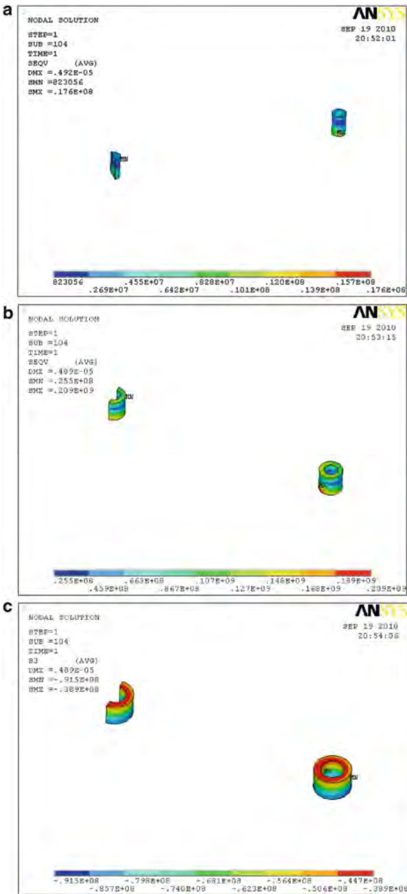
Fig. 6.30 The stress distribution of TSV filled with epoxy at reflow: (a) the von Mises stress of epoxy core in TSV (max 17.6 MPa), (b) the von Mises stress of TSV copper (max 209 MPa), and (c) the compressive stress S3 of isolation layer (max 91.5 MPa)
