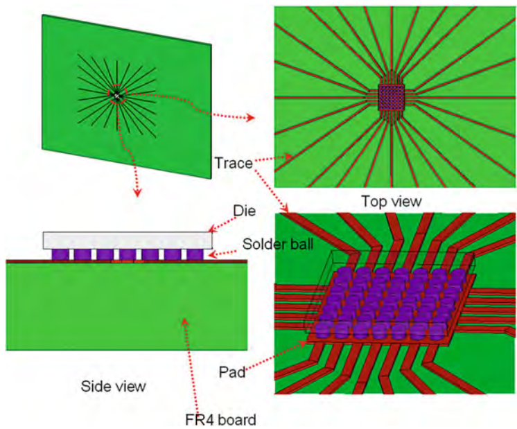
Fig. 7.10 WLCSP (49 balls) mounted on JEDEC 1S0P thermal test board
