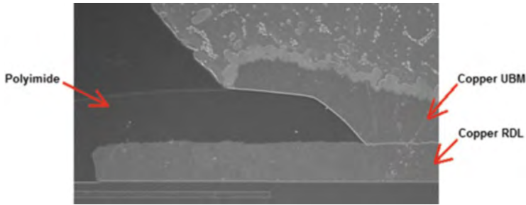
Fig. 10.55 SEM picture of the 2Cu1Pi WLCSP
