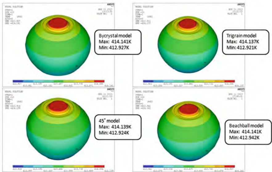
Fig. 8.51 Temperature distribution of four different microstructures
