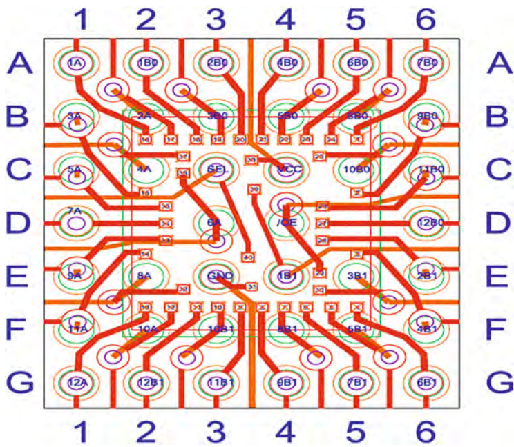
Fig. 8.26 The pin map distribution and RDL of the MCSP with GGI
