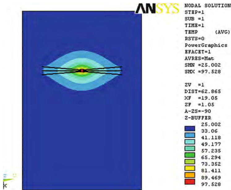
Fig. 7.22 Simulated temperature distribution of 6-ball WLCSP under 0.25 W power input (1SOP, the worst internal trace layout)
