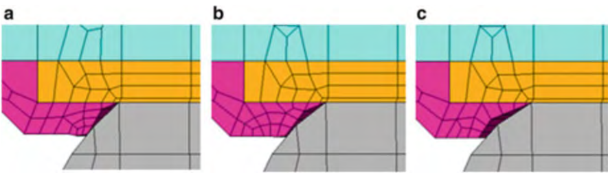
Fig. 10.41 Finite element model of the three different polyimide layouts: (a) PI layout 1, (b) PI layout 2, and (c) PI layout 3
