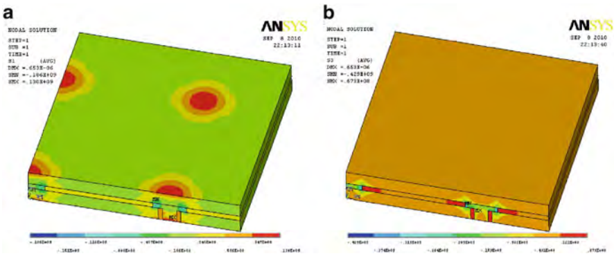
Fig. 6.18 The principal stress of the stack die power package at 25 C after the stacking process: (a) the first principal stress S1 (tensile) (max 130 MPa) and (b) the third principal stress S3 (compressive) (max 429 MPa)
