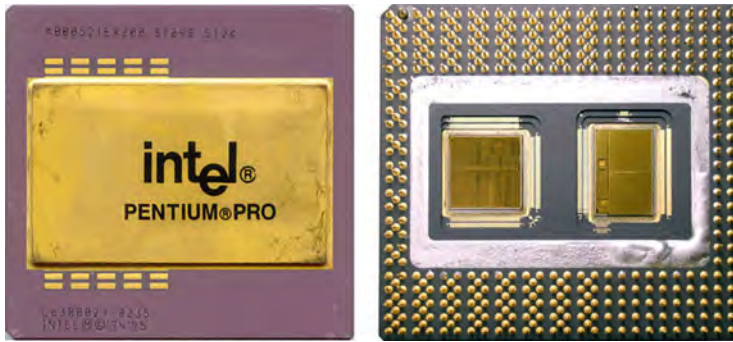
Fig. 4.1 Intel® Pentium® Pro top view of heat sink and bottom view PGA and solder ring (after removal of cap plate) and two dies with gold wire bond
