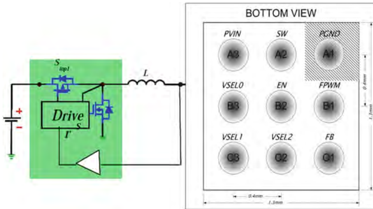
Fig. 1.8 Wafer-level integrated power solution
