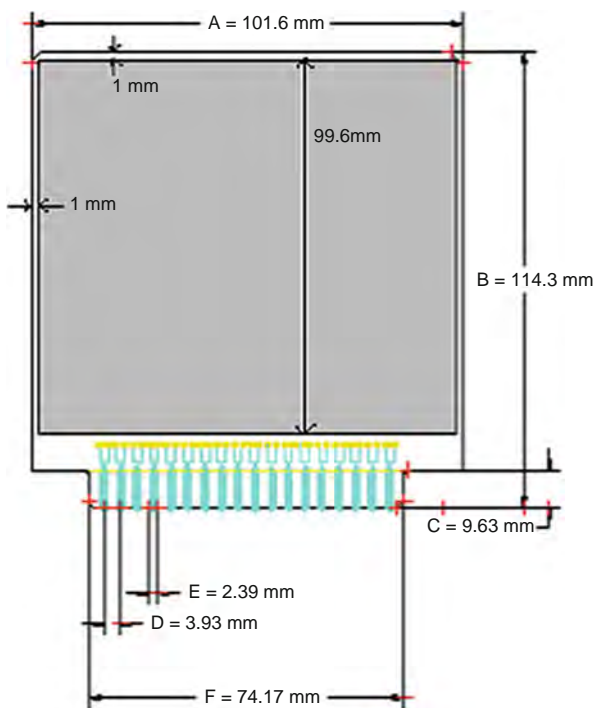
Fig. 7.7 PCB for packages >27.0 mm long 99.60 \times 96.60 (mm 2 ) buried planes
