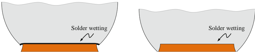
Fig. 9.6 Wetting of solder joints on ENIG finish ( left ) and OSP/immersion Ag finish ( right )
