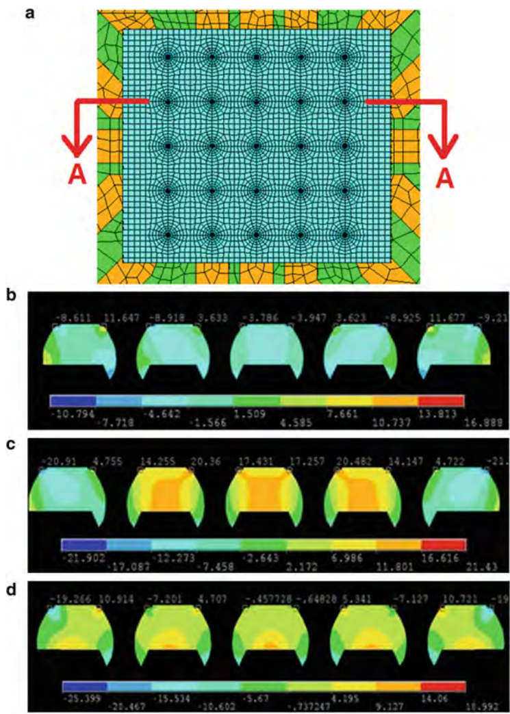
Fig. 10.24 Solder joint Z component stress. (a): solder joint’s cross-section position. (b): A–A cross-section view of Sz stress for Model 1 (no via). Maximum Sz: 16.8 MPa at corner joints. (c): A–A cross-section view of Sz stress for Model 2 (9 vias). Maximum Sz: 21.4 MPa on inner joints. (d): A–A cross-section view of Sz stress for Model 3 (25 vias). Maximum Sz: 18.9 MPa at corner joint
