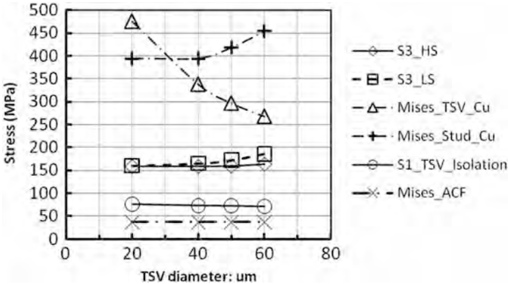
Fig. 6.21 The stresses of HS, LS, Cu stud, TSV Cu, ACF, and isolation layer versus TSV diameter
