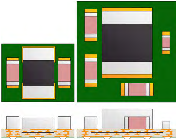
Fig. 5.28 Top view and cross-sectional view of the two studied embedded WLCSP modules
