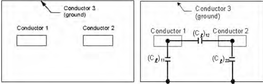
Fig. 8.12 A three conductor system
