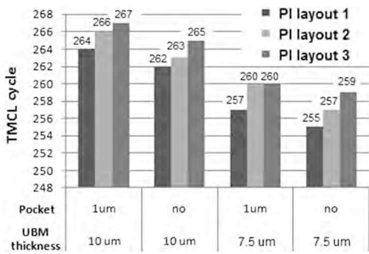
Fig. 10.49 First failure cycle comparison of solder at the interface to UBM (different polyimide layouts, UBM thicknesses, and UBM pocket designs)
