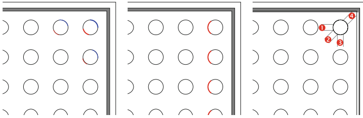
Fig. 2.9 High stress on WLCSP in TMCL ( left ), in drop ( middle , assuming major bending is in X direction), and directions of traces that should be avoided ( right ): direction 1 and 3 correspond to potential high stress in drop and direction 2 and 4 correspond to potential high stress in TMCL
