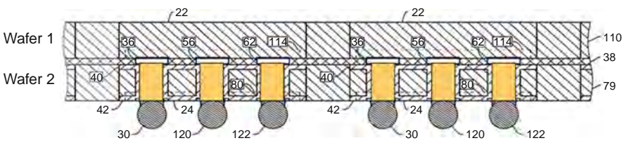
Fig. 6.14 The cross section of the wafer-level buck converter with two stacked wafers before singulation (wafer 1 for high side and wafer 2 for low side)
