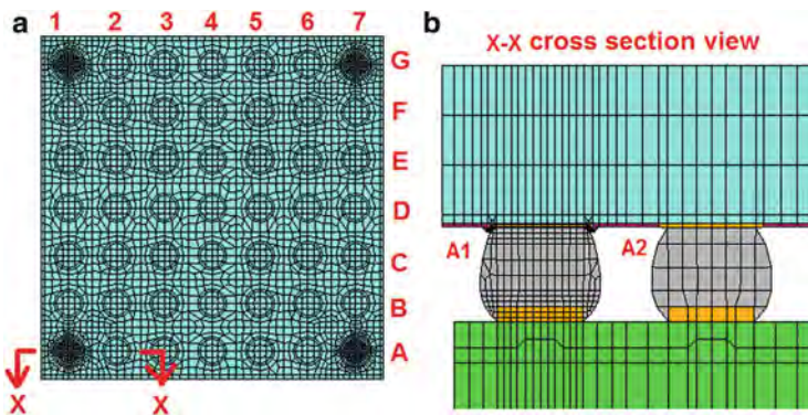
Fig. 10.37 Cross section of WLCSP. (a) WLCSP 7 \times 7 top view. (b) A–A cross-section view
