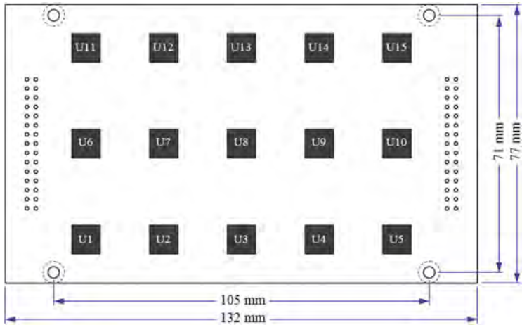
Fig. 2.5 JEDEC drop PCB with 15 components mounted on
