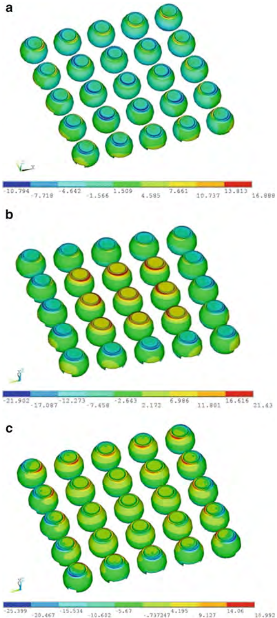
Fig. 10.23 Solder joint's Z component stress comparison. (a) Model 1: no through PCB vias. Maximum Sz at the corner of 5 \times 5 array: 16.9 MPa. (b) Model 2: nine through PCB vias. Maximum Sz at the corner of inner 3 \times 3 array: 21.4 MPa. (c) Model 3: 25 through PCB vias. Maximum Sz at the corner of 5 \times 5 array: 19 MPa
