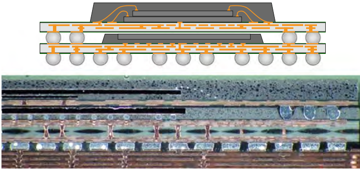
Fig. 4.7 Top : schematic cross section of PoP with memory chip stack MCM on top of flip chip BGA package. Bottom : cross section of Apple® A7 processor. Overall PoP is 14 \times 15.5 \times 1.0 mm with 1330 BGA bumps at 0.4 mm pitch. Top package : 1 GB LPDDR3 with 456 perimeter bumps at 0.35 mm pitch. Bottom package : dual core ARM CPU with integrated GPU and L1, L2, and L3 cache flip chip SoC. Flip chip bump pitch is 150/170 \mu\text{m} (Photo source: Prismark/Binghamton University)
