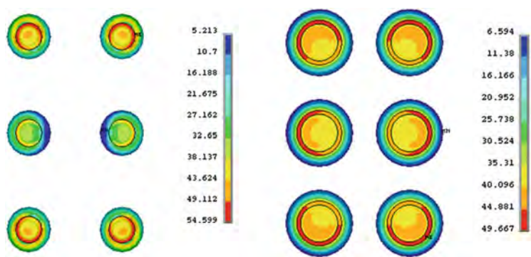
Fig. 6.11 The von Mises stresses of micro bump and standard bump at -40\text{ }^{\circ}\text{C} in TMCL: (a) micro bump (max 54.6 MPa) and (b) standard bump (max 49.7 MPa)
