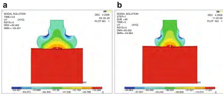
Fig. 5.21 Deformation of the model after bonding process with different FAB sizes: (a) 190 \mu\text{m} , (b) 145 \mu\text{m}
