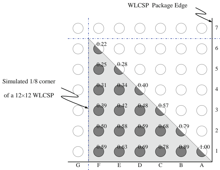
Fig. 3.14 Normalized inelastic strain energy density per cycle for the 1/8 part of a 12 × 12 bump WLCSP. Higher inelastic strain energy density prompts earlier TMCL fails
