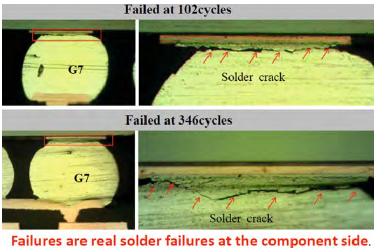
Fig. 10.63 Solder's thermal cycling failure of 1Cu1Pi design
