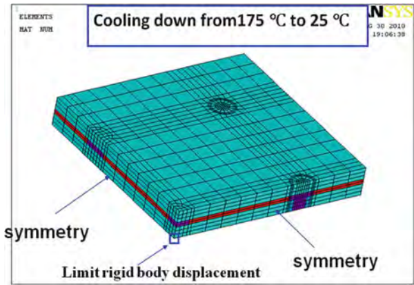
Fig. 6.17 The quarter model of the stack die power package
