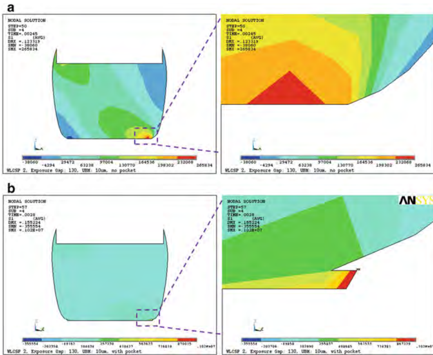
Fig. 10.44 First principal stress S1 of with pocket versus without pocket designs in drop test. (a) Max solder S1: 265.8 MPa (no pocket in UBM). (b) Max solder S1: 1,020 MPa (1 \mu m pocket in UBM)
