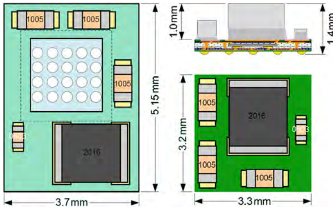
Fig. 4.19 Module size saving is >44 % with changing design from all SMT solutions ( left ) to the embedded WLCSP solution ( right ). Overall package height remains the same due to aggressive thinning of silicon
