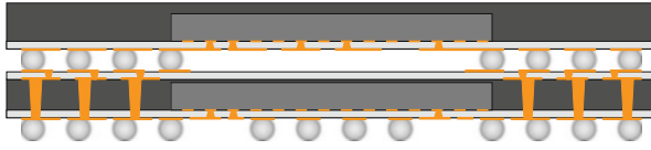
Fig. 4.13 A conceptual PoP based on fan-out WLCSP. Through-mold via (TMV) is drilled through bottom fan-out package to make the front (active side) to back vertical interconnections. Backside rerouting is needed for connecting the top chip. In case of full area array, fan-in routing could be made on the back side of bottom package
