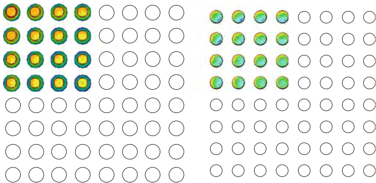
Fig. 2.8 Von Mises stress (Svm) distribution in solder joints on WLCSP chip side ( left ) and first principle stress S1 in BOP aluminum pad. Simulated TMCL PCB has eight layers of copper and aspect ratio of 1.71
