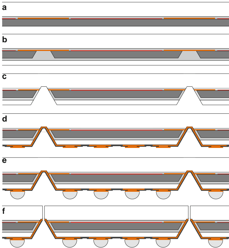
Fig. 4.15 Schematic process flow of ShellOP: (a) bonding silicon to glass carrier and backgrind; (b) forming V trench and attaching bottom glass; (c) V cut through pad metal; (d) backside metallization and redistribution + UBM; (e) print solder or ball drop and reflow; (f) singulation
