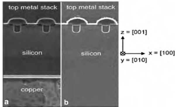
Fig. 1.6 (a) Fairchild UMOSET, (b) regular Mosfet [19]
