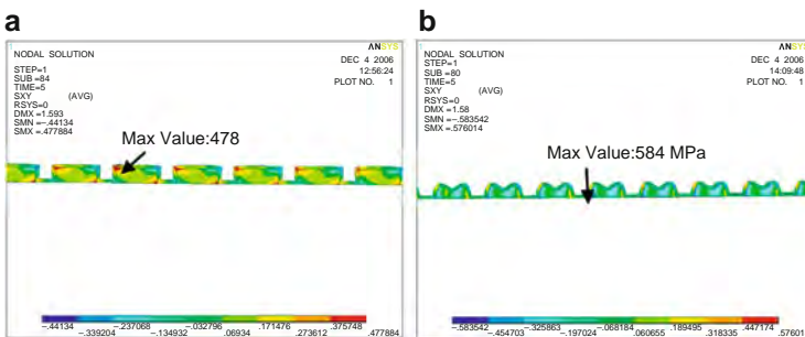
Fig. 5.23 Shear stress distribution of the BPSG/TiW layer for different BPSG profiles: (a) square shape, (b) M shape
