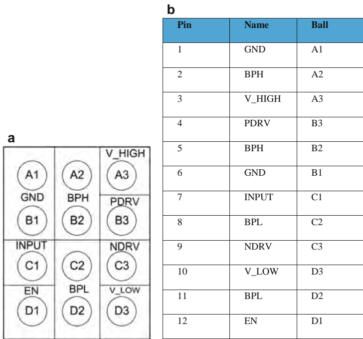
Fig. 8.2 3 × 4 WLCSP pin map. (a) 3 × 4 WLCSP Pin map (b) Pin number
