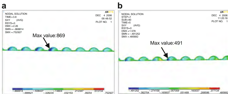
Fig. 5.22 Shear stress distribution in BPSG/TiW layer with different FAB sizes: (a) 190 \mu\text{m} , (b) 145 \mu\text{m}
