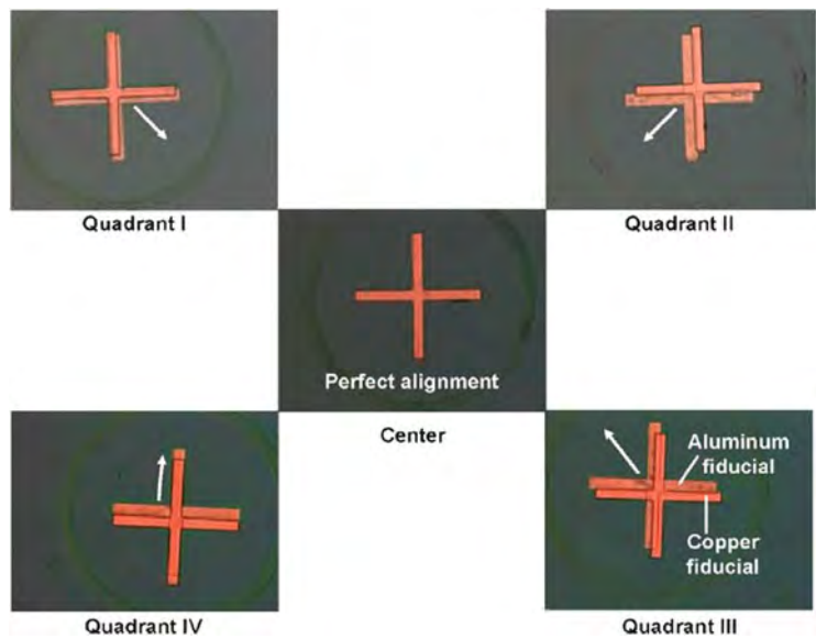
Fig. 3.10 Die shift through fan-out molding process revealed by the cross target method. Here cross targets built on the chip and cross targets build in the bumping layer, at 5 locations across a 200mm fan-out wafer, show the directions of die shift through the molding/curing process
