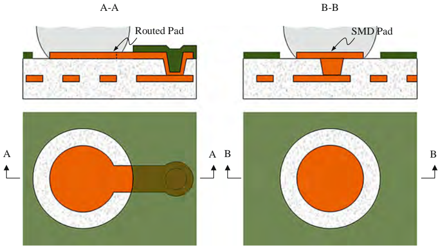
Fig. 9.7 Cross-sectional view and top view of routed PCB copper pad and via-in-pad PCB copper pad. Filled copper via is desired in the via-in-pad design
