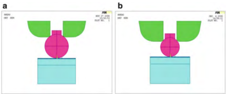
Fig. 5.17 A 2D FEA model including silicon, Cu wire, and capillary with different FAB sizes: (a) 190 \mu\text{m} and (b) 145 \mu\text{m}
