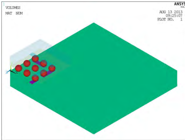
Fig. 8.47 Quarter global model
