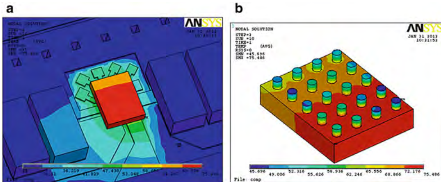
Fig. 7.26 Temperature distribution of the WLCSP on board at 1 s (power on die: 1.5 W) (a) The system temperature (b) The temperature of WLCSP (max: 75.5 °C)
