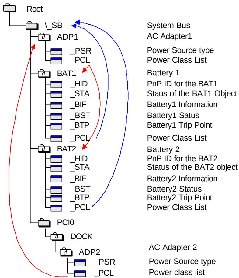
Figure 11-4 Power Source Name Space Example that Includes a Docking Station
