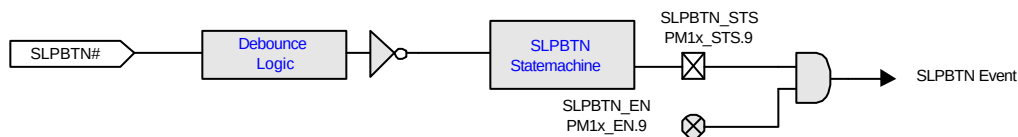
Figure 4-9 Fixed Sleep Button Logic
