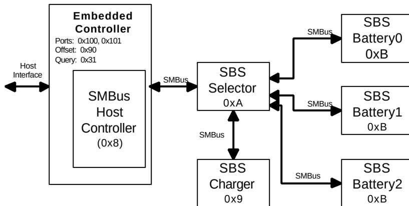
Figure 11-3 Smart Battery Subsystem
