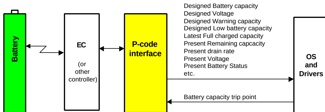
Figure 3-3 Control Method Battery Diagram
