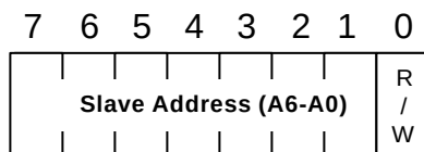
Figure 15-1 SMBus Slave Address Protocol
