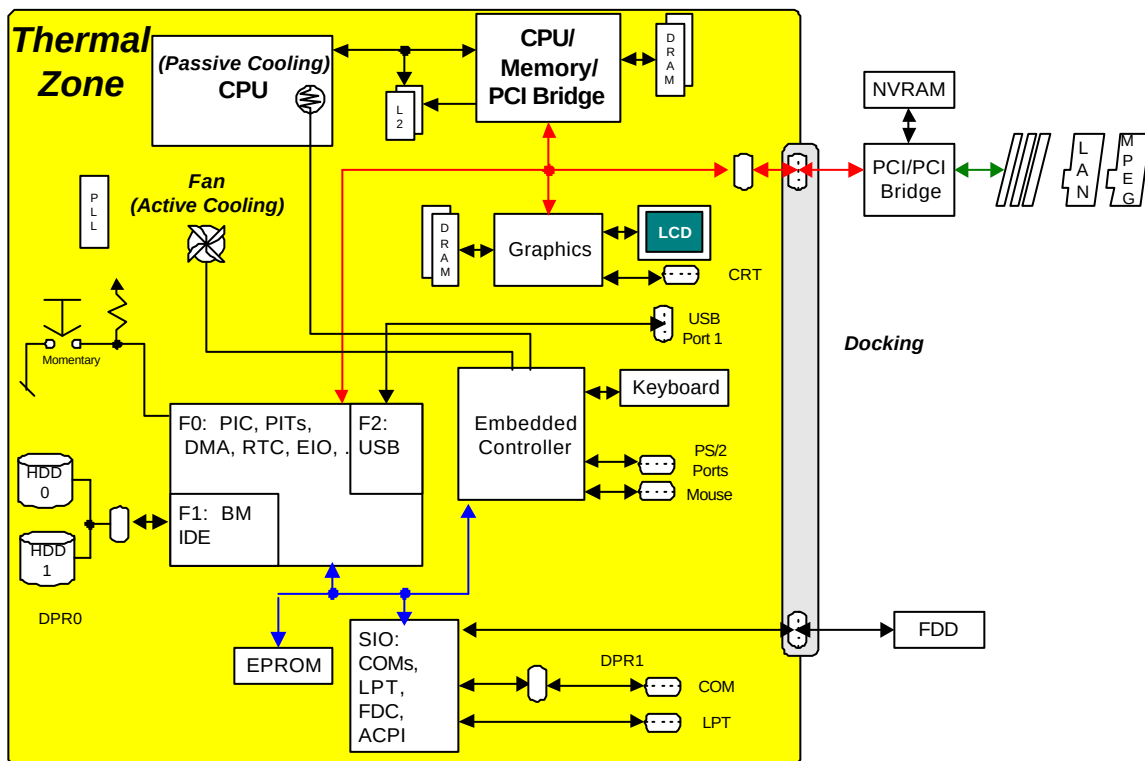
Figure 3-6 Thermal Zone
