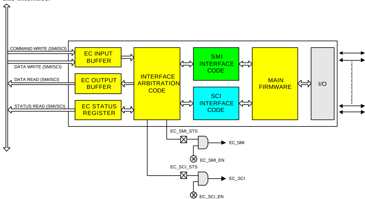
Figure 13-1 Shared Interface
