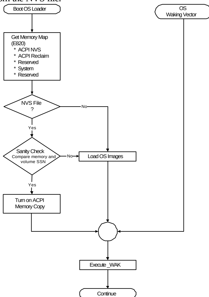
Figure 9-5 OS Initialization
