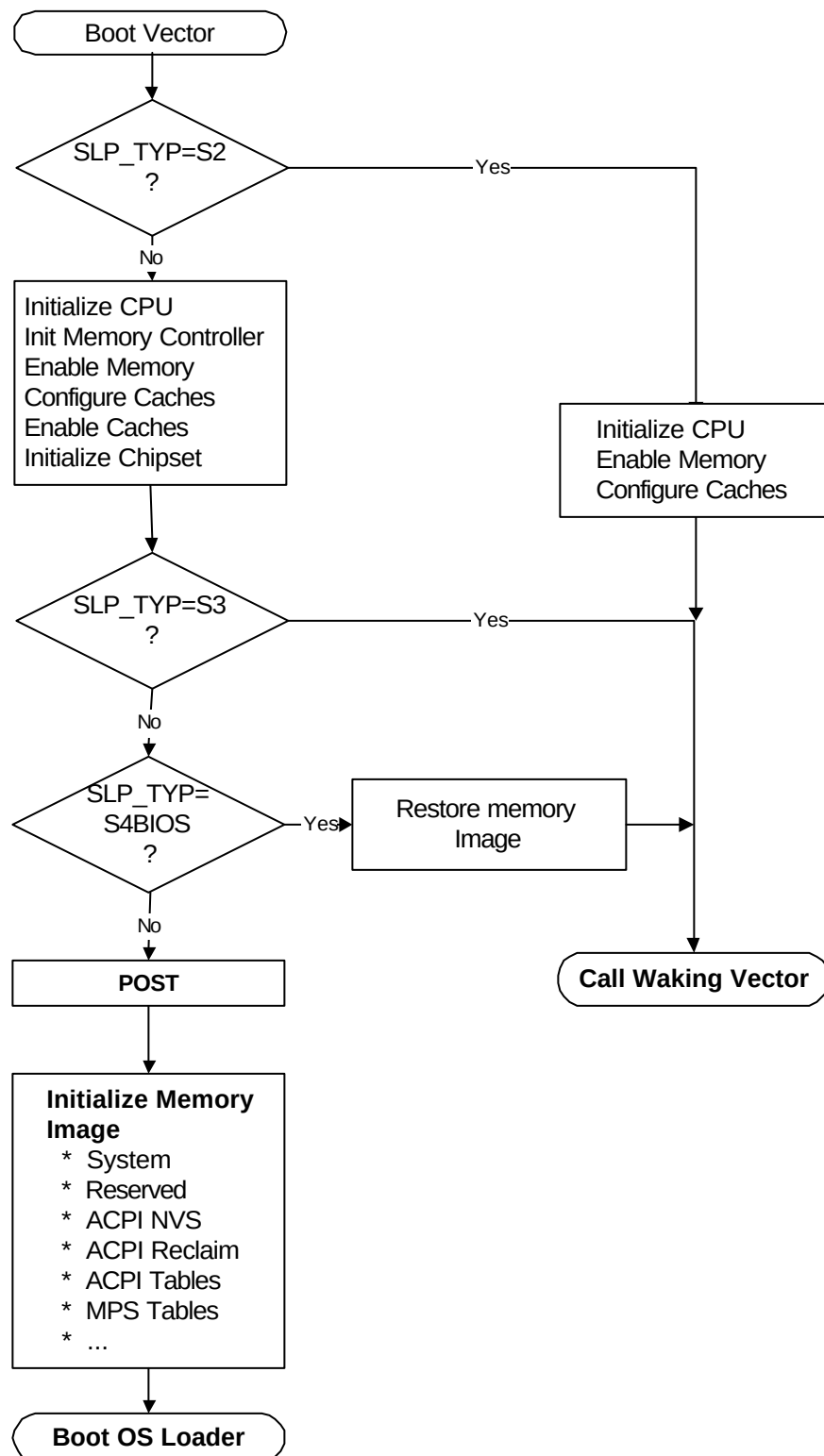
Figure 9-2 BIOS Initialization
