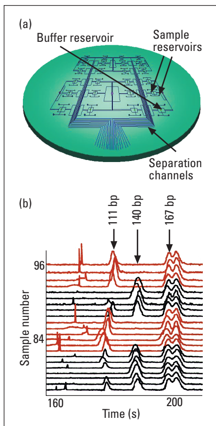
FIGURE 3. Diagram of a 96-sample device for DNA analysis.
