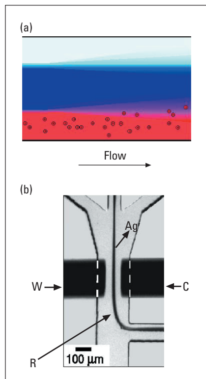
FIGURE 2. Fluorometric sensor based on laminar flow.
