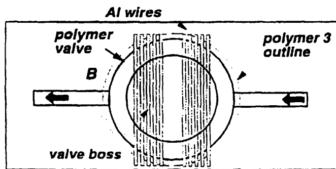
Figure 8: Pass-through valve. The valve is normally closed and opens when the diaphragm is buckled upwards
