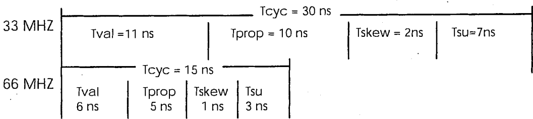
Figure 7-1: 33 MHz PCI vs. 66 MHz PCI Timing
