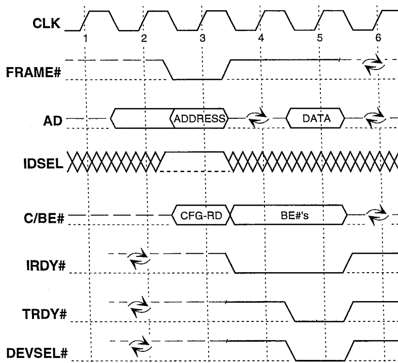
Figure 3-4: Configuration Read
