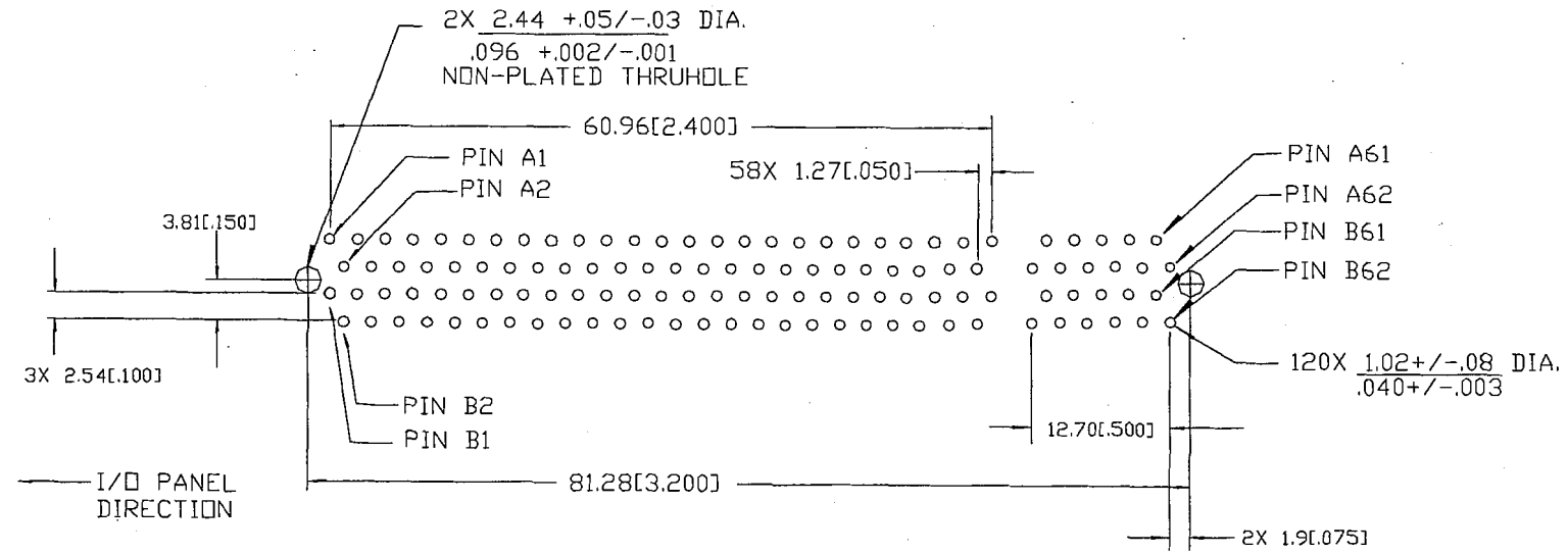
Figure 5-37: 32-bit/5V PCI Riser Connector Footprint
