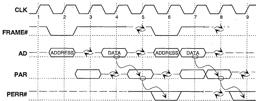
Figure 3-20: Parity Operation
