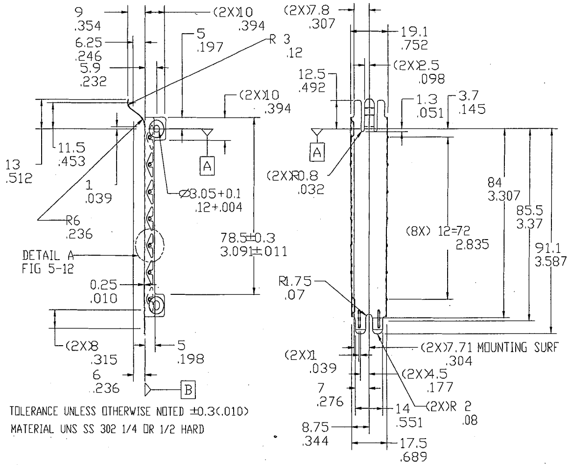
Figure 5-17: MC Bracket
