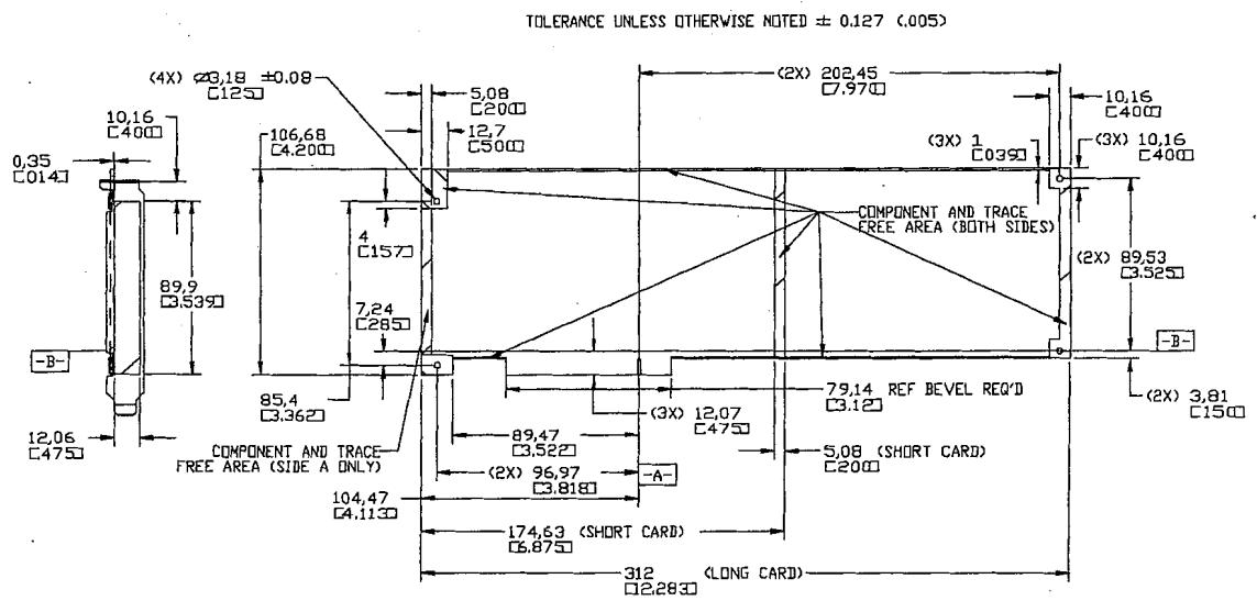
Figure 5-1: PCI Raw Card (5V)
