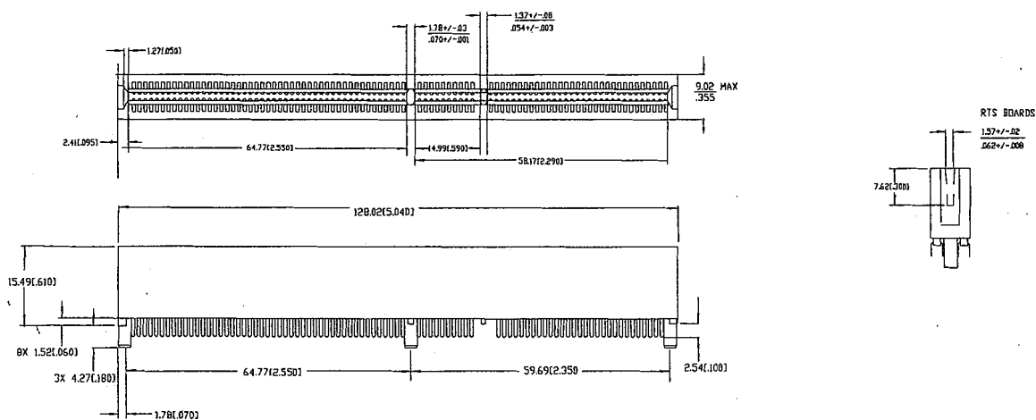
Figure 5-22: 5V/64-bit Connector
