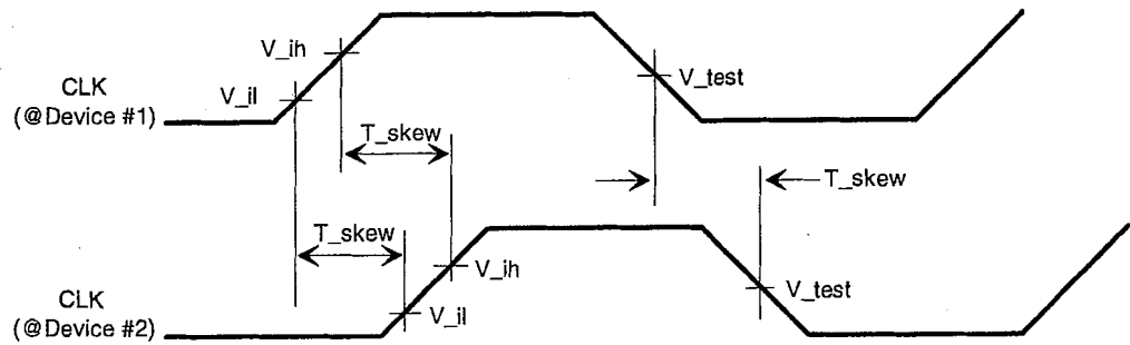
Figure 4-10: Clock Skew Diagram
