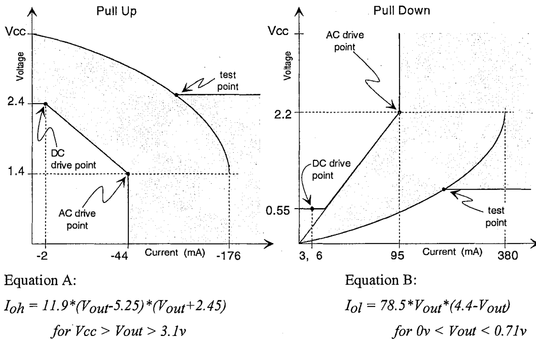
Figure 4-2: V/I Curves for 5V Signaling
