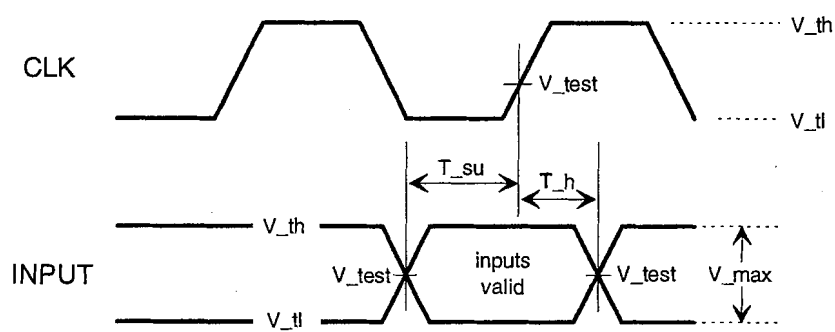
Figure 4-8: Input Timing Measurement Conditions
