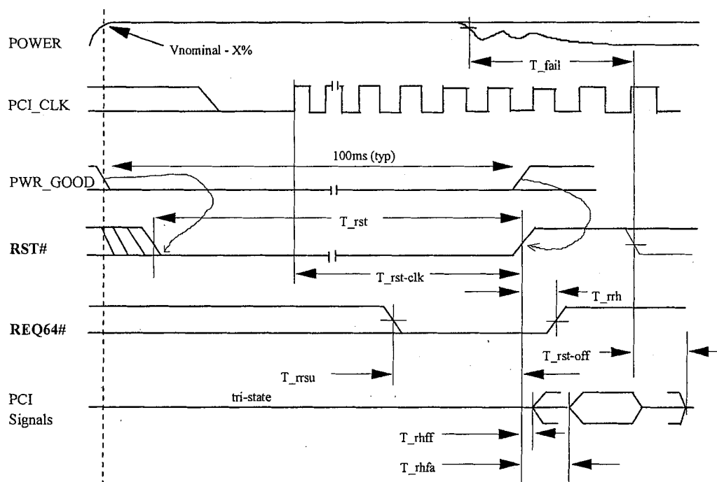
Figure 4-11: Reset Timing 34
