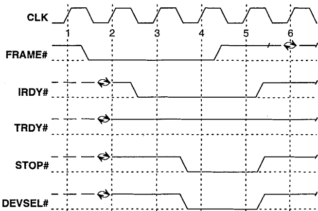
Figure 3-9: Retry
