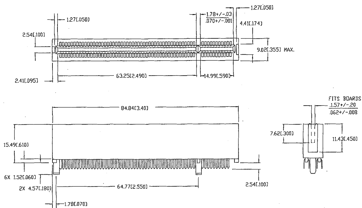
Figure 5-19: 32-bit Connector
