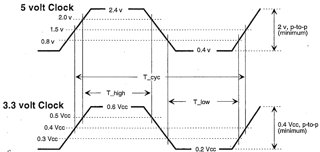
Figure 4-6: Clock Waveforms
