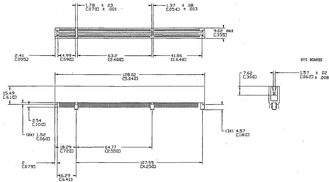
Figure 5-24: 3.3V/64-bit Connector
