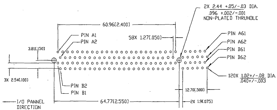
Figure 5-20: 5V/32-bit Connector Layout Recommendation
