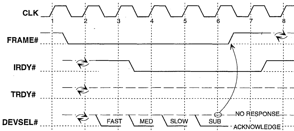
Figure 3-8: Master-Abort Termination
