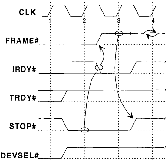
Figure 3-14: Target-Abort
