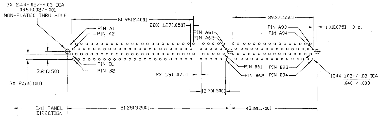
Fig 5-?? Riser 64 bit/5V Connector footprint
