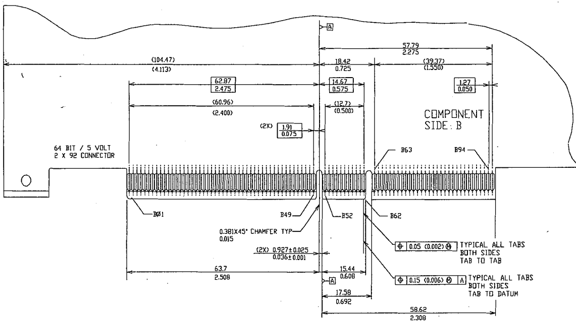
Figure 5-27: 5V/64-bit Card Edge Connector Dimensions and Tolerances
