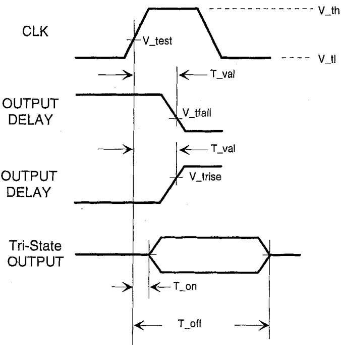
Figure 7-3: Output Timing Measurement Conditions
