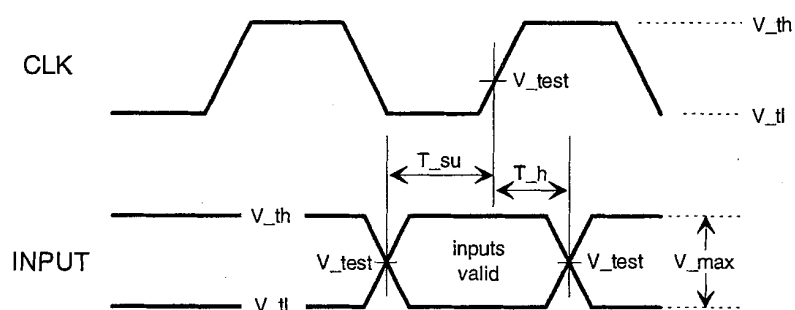
Figure 4-8: Input Timing Measurement Conditions
