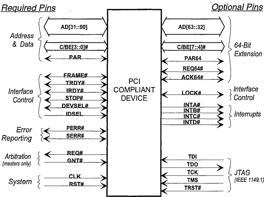
Figure 2-1: PCI Pin List
