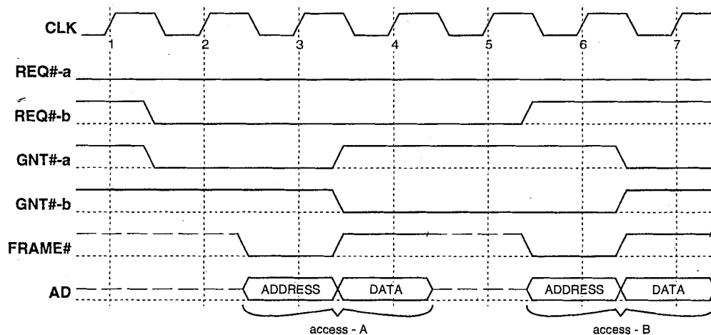
Figure 3-15: Basic Arbitration
