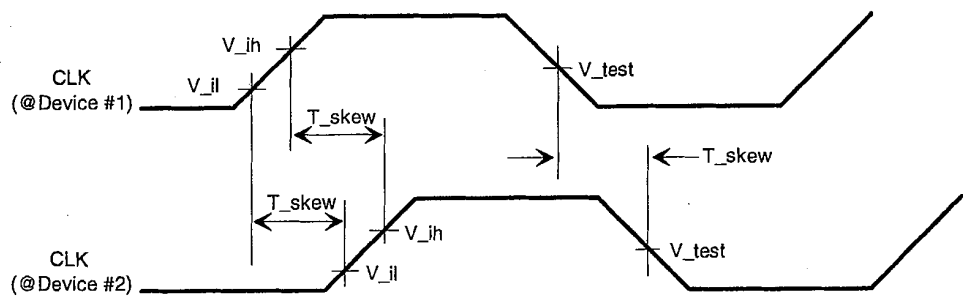
Figure 4-10: Clock Skew Diagram
