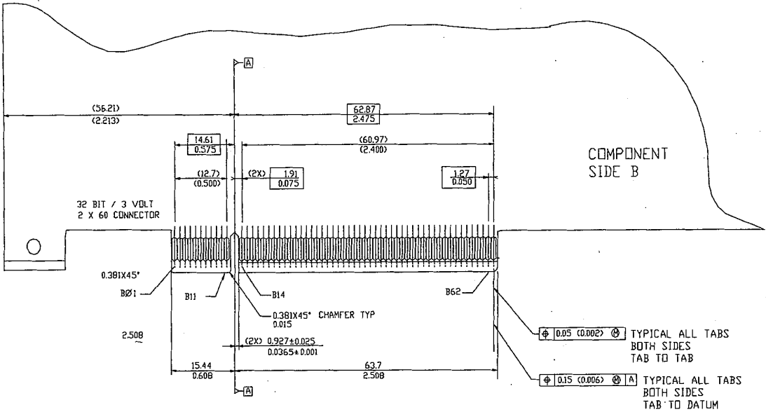
Figure 5-28: 3.3V/32-bit Card Edge Connector Dimensions and Tolerances
