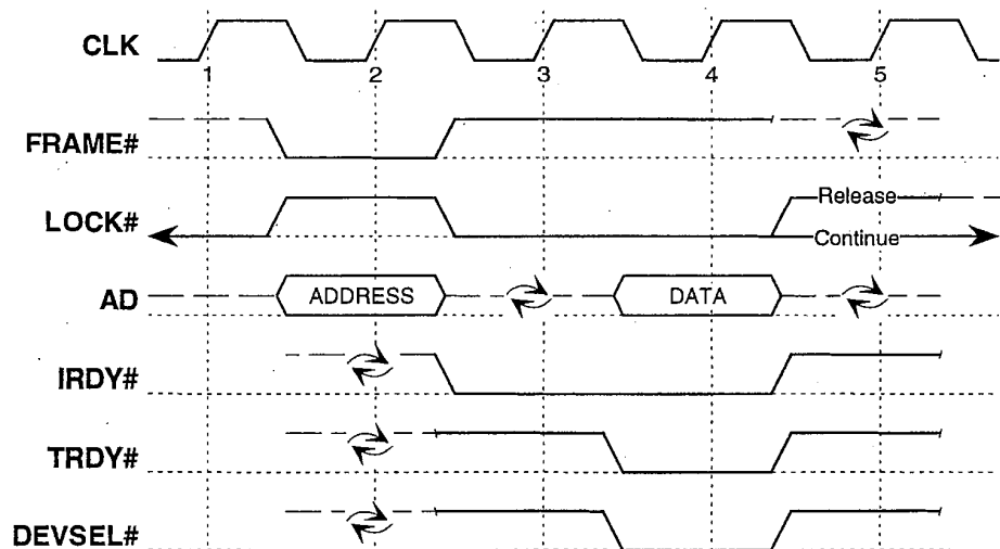
Figure F-2: Continuing an Exclusive Access
