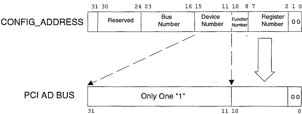
Figure 3-3: Host Bridge Translation for Type 0 Configuration Transactions Address Phase
