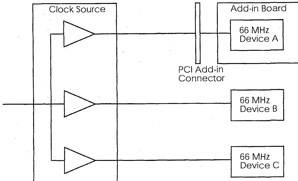
Figure 7-8: Recommended Clock Routing
