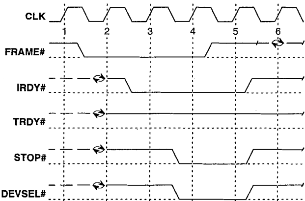
Figure 3-9: Retry
