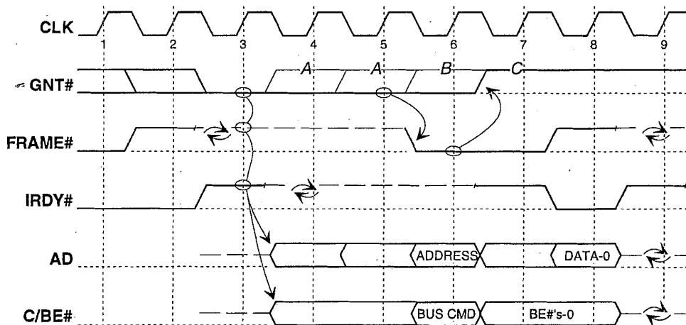
Figure 3-18: Address Stepping
