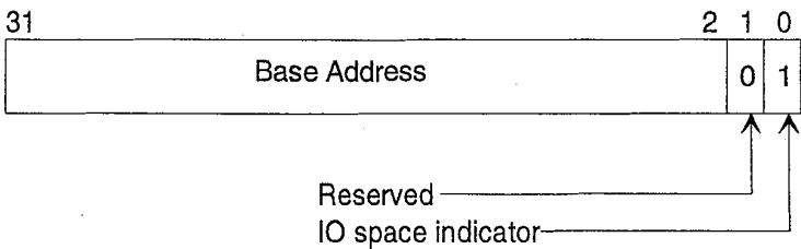
Figure 6-6: Base Address Register for I/O
