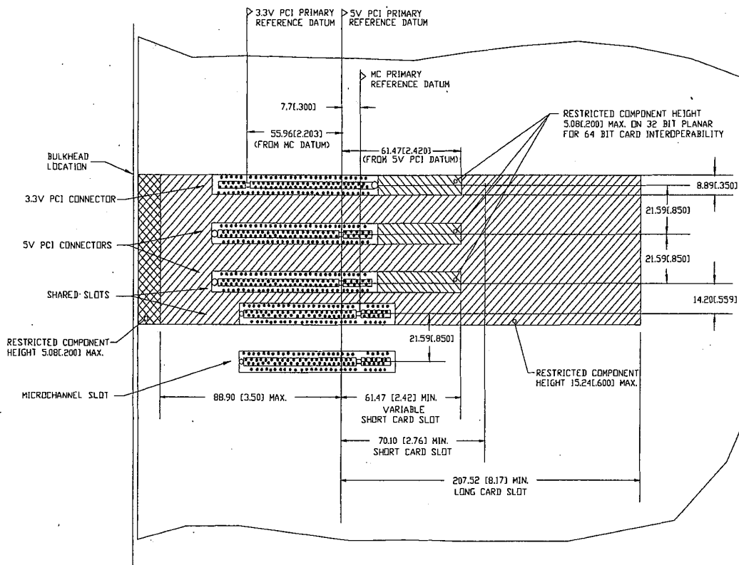
Figure 5-35: PCI Connector Location on Planar Relative to Datum on the MC Connector
