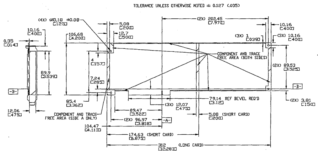
Figure 5-1: PCI Raw Card (5V)
