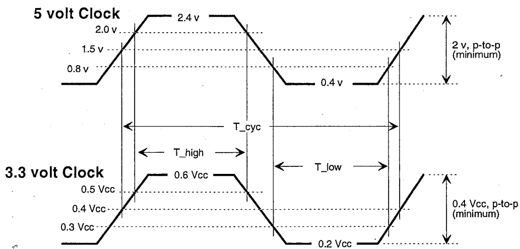
Figure 4-6: Clock Waveforms
