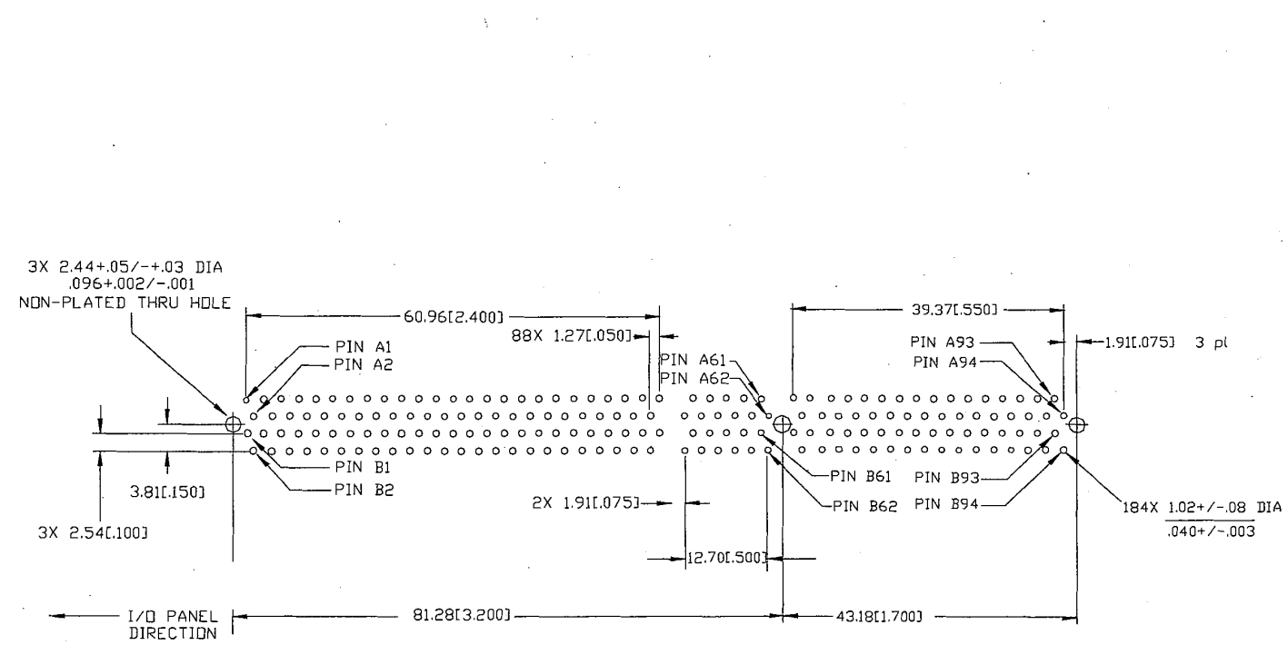
Figure 5-40: 64-bit/5V PCI Riser Connector Footprint
