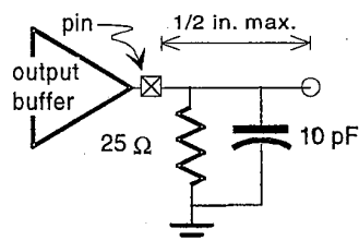
Figure 7-5: T_{val(max)} Rising Edge
