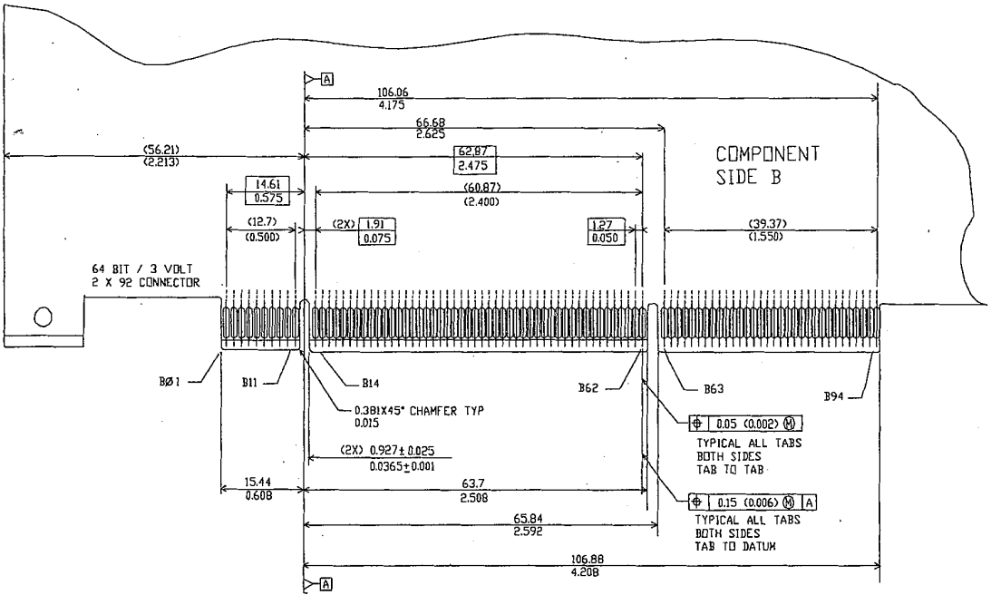
Figure 5-29: 3.3V/64-bit Card Edge Connector Dimensions and Tolerances
