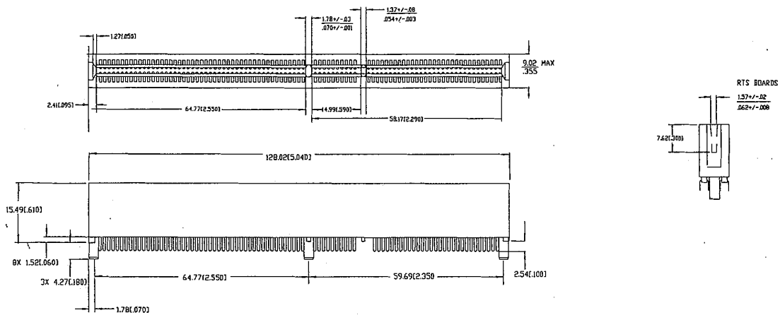
Figure 5-22: 5V/64-bit Connector
