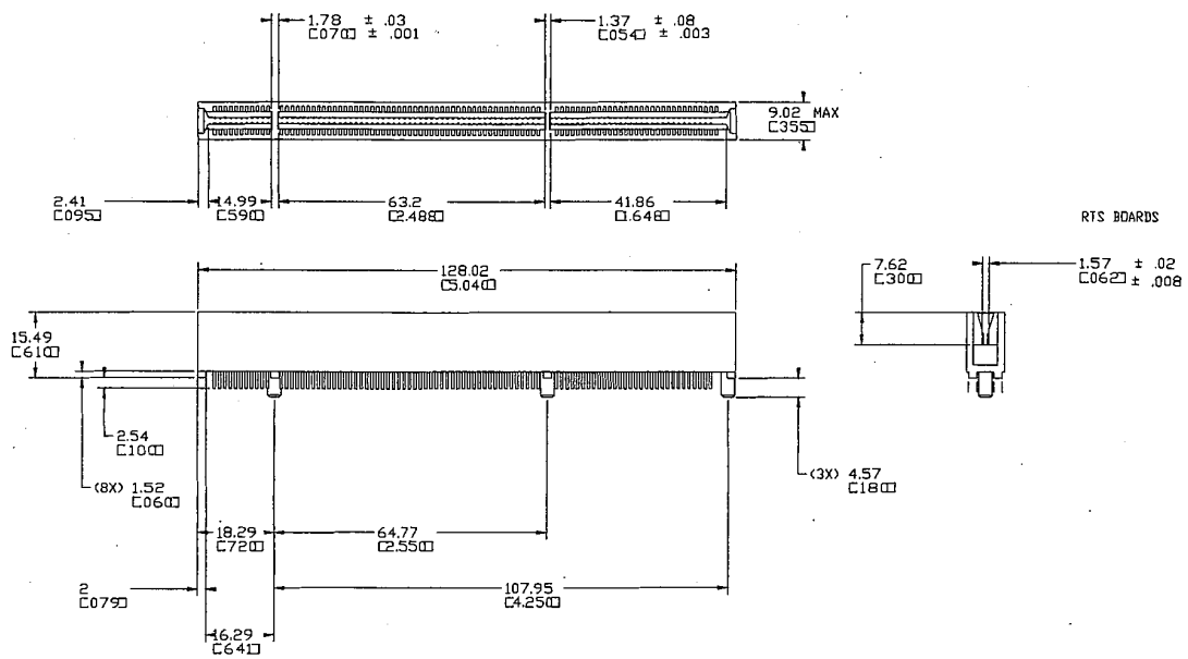
Figure 5-24: 3.3V/64-bit Connector
