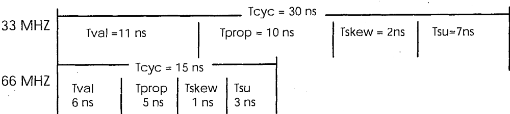
Figure 7-1: 33 MHz PCI vs. 66 MHz PCI Timing
