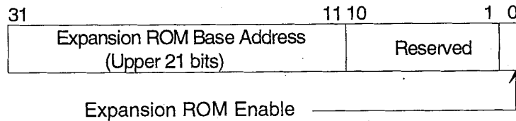
Figure 6-7: Expansion ROM Base Address Register Layout
