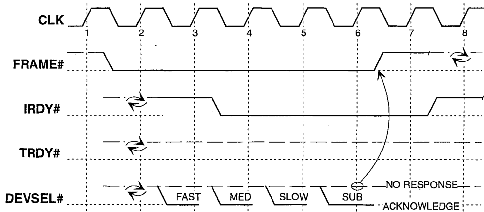
Figure 3-8: Master-Abort Termination
