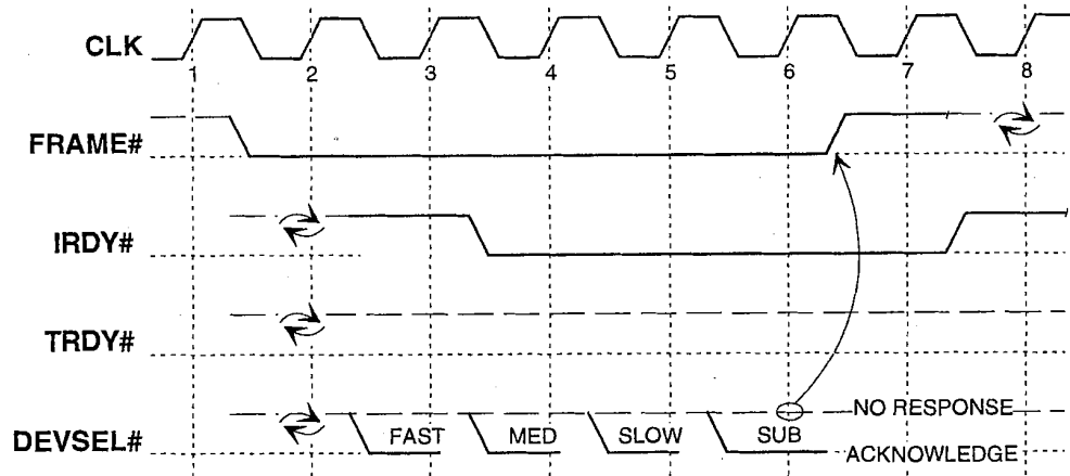
Figure 3-17: DEVSEL# Assertion
