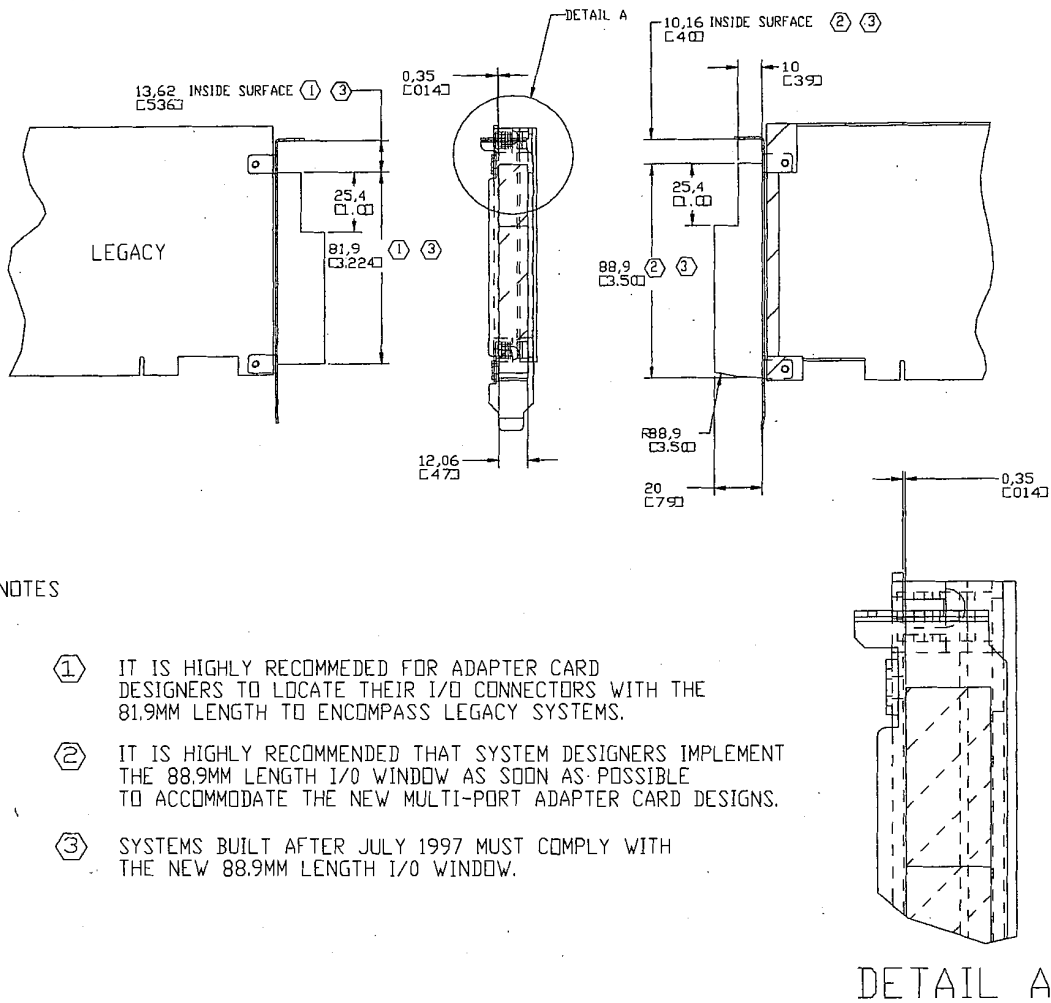
Figure 5-14: I/O Window Height
