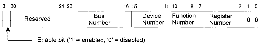
Figure 3-2: Layout of CONFIG_ADDRESS Register
