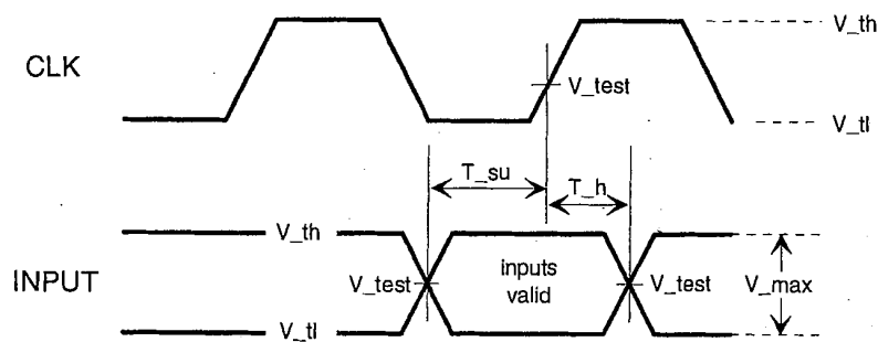
Figure 7-4: Input Timing Measurement Conditions
