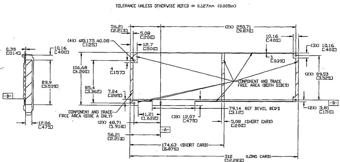
Figure 5-2: PCI Raw Card (3.3V and Universal)
