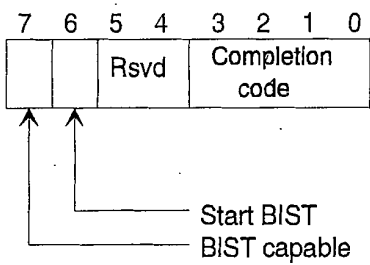
Figure 6-4: BIST Register Layout
