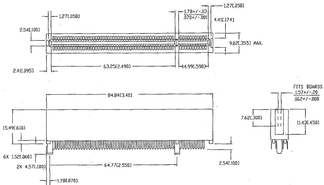
Figure 5-19: 32-bit Connector
