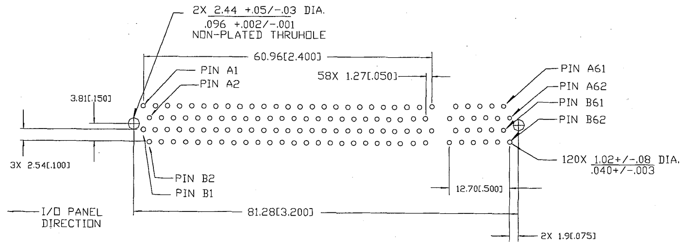
Figure 5-37: 32-bit/5V PCI Riser Connector Footprint
