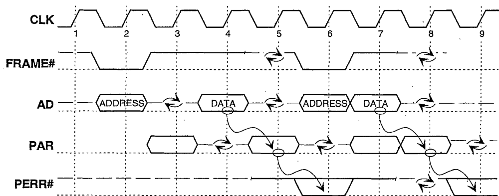
Figure 3-20: Parity Operation
