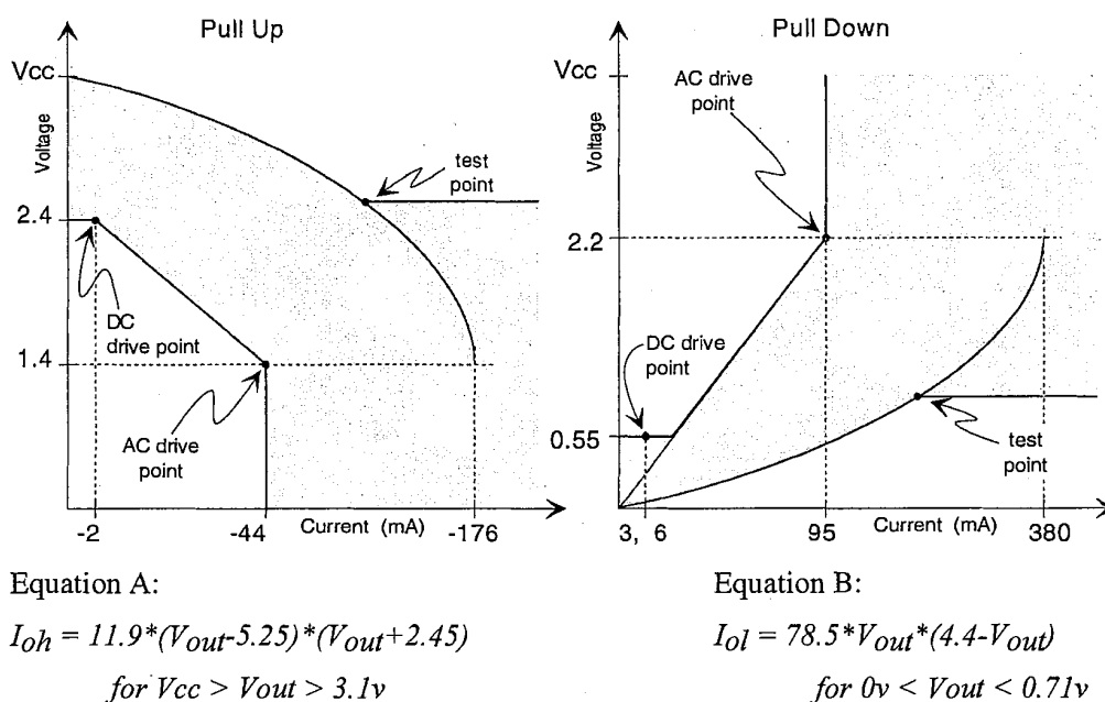
Figure 4-2: V/I Curves for 5V Signaling
