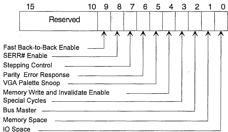
Figure 6-2: Command Register Layout
