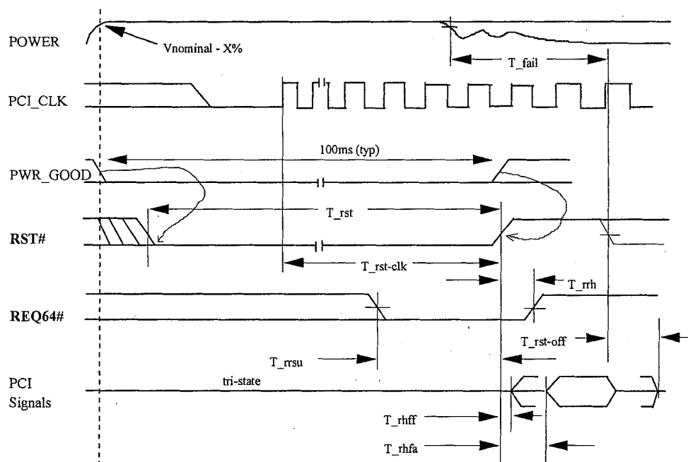
Figure 4-11: Reset Timing 34
