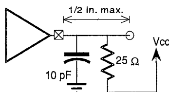
Figure 7-6: T_{val(max)} Falling Edge
