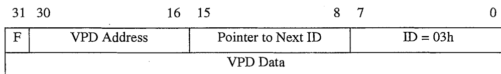
Figure I-1: VPD Capability Structure
