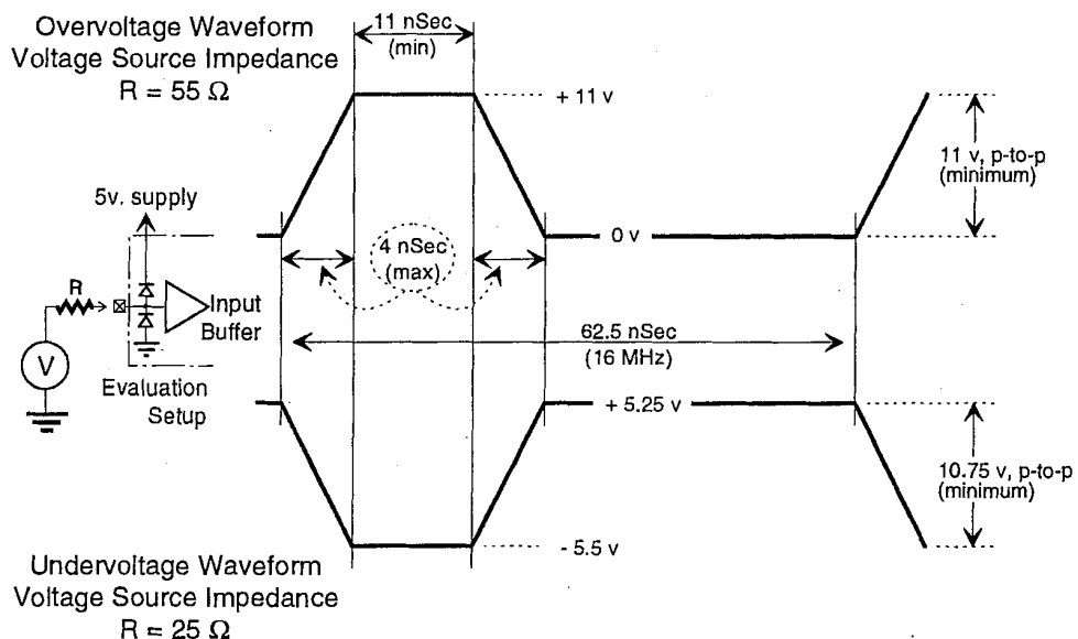
Figure 4-3: Maximum AC Waveforms for 5V Signaling
