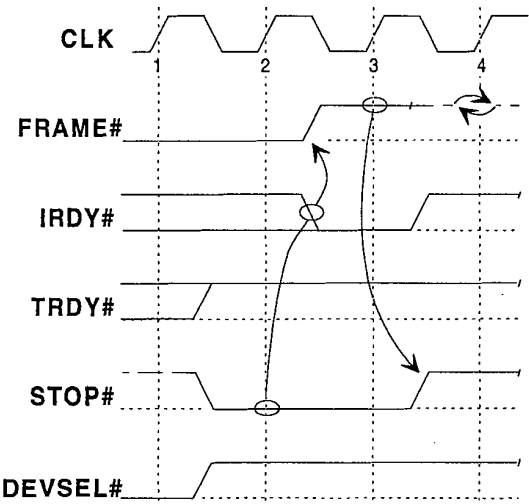
Figure 3-14: Target-Abort
