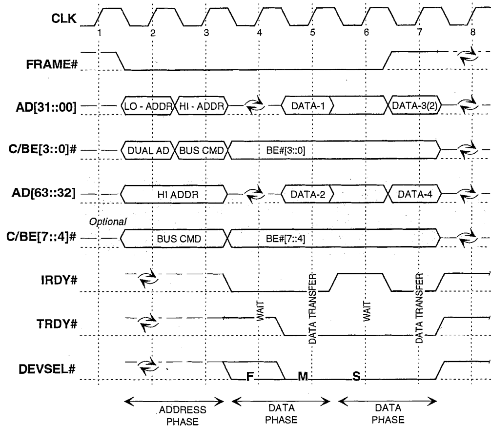
Figure 3-23. 64-Bit Dual Address Read Cycle
