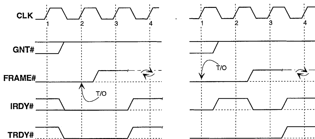
Figure 3-7: Master Initiated Termination
