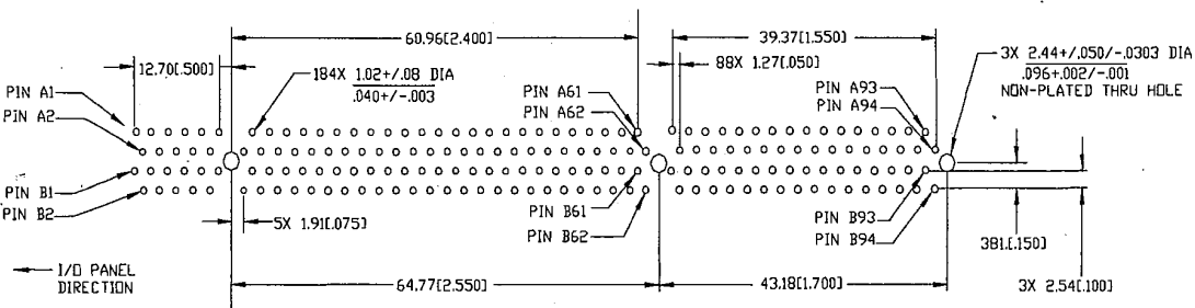
Figure 5-25: 3.3V/64-bit Connector Layout Recommendation
