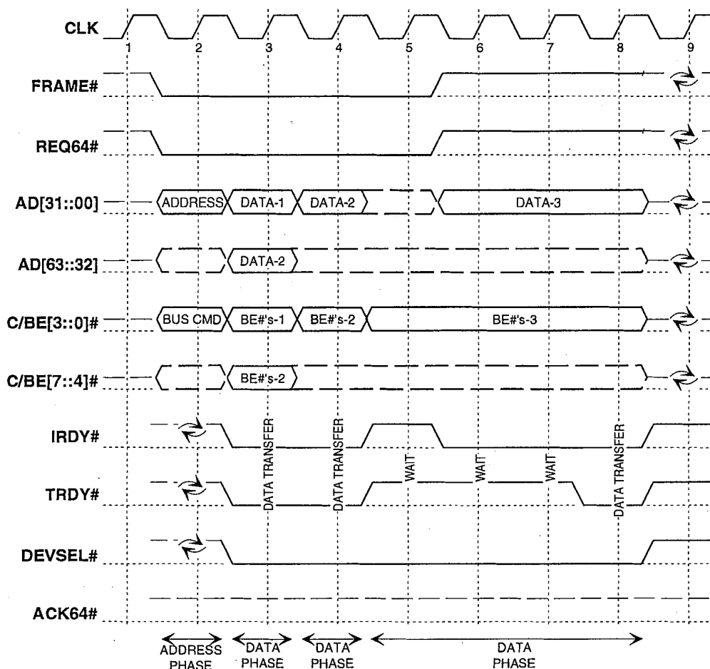
Figure 3-22: 64-bit Write Request With 32-bit Transfer
