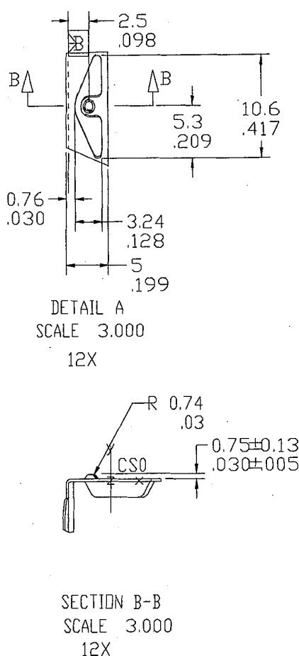
Figure 5-18: MC Bracket Details
