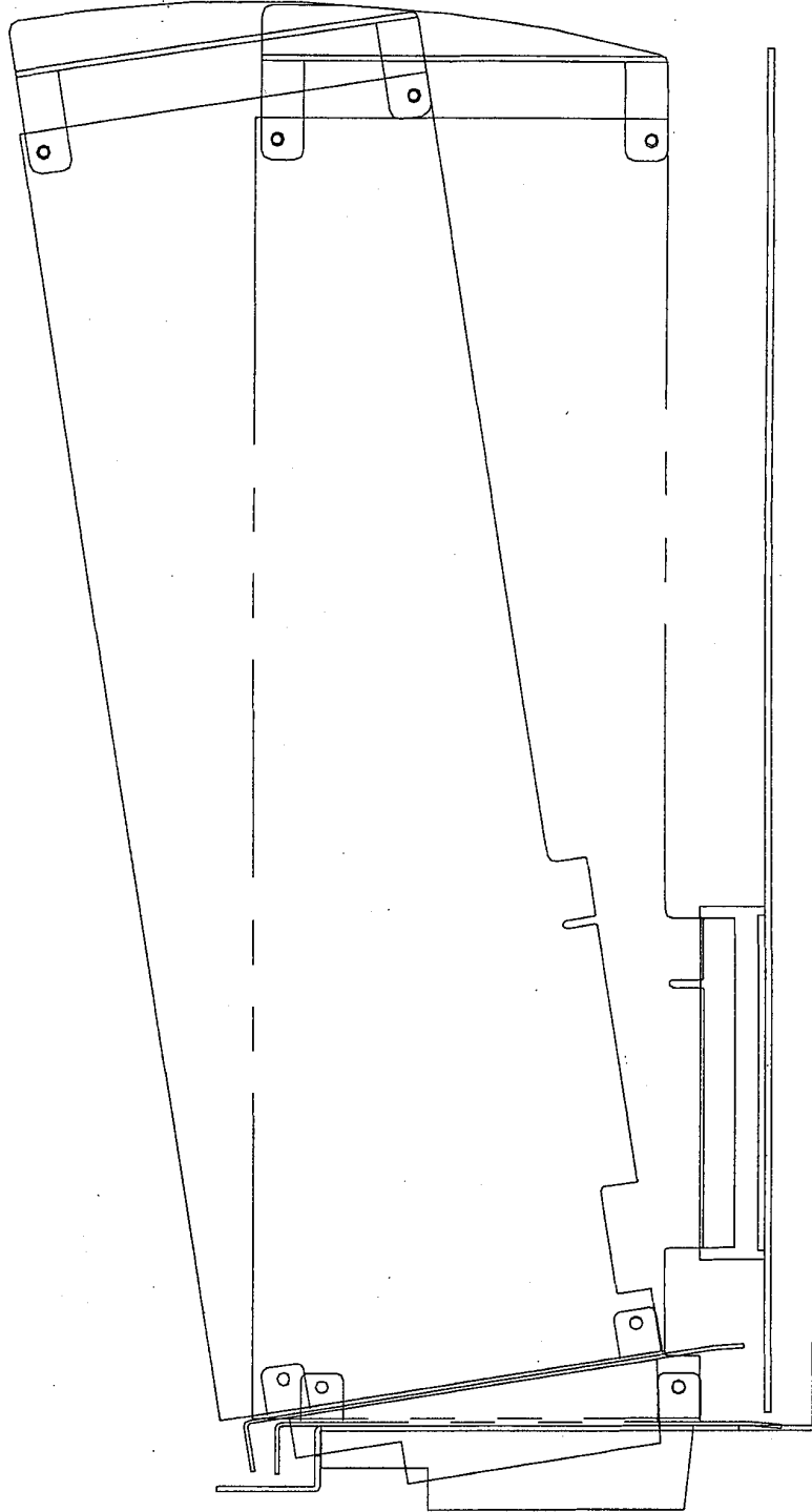
Figure 5-15: Adapter Installation With Large I/O Connector
