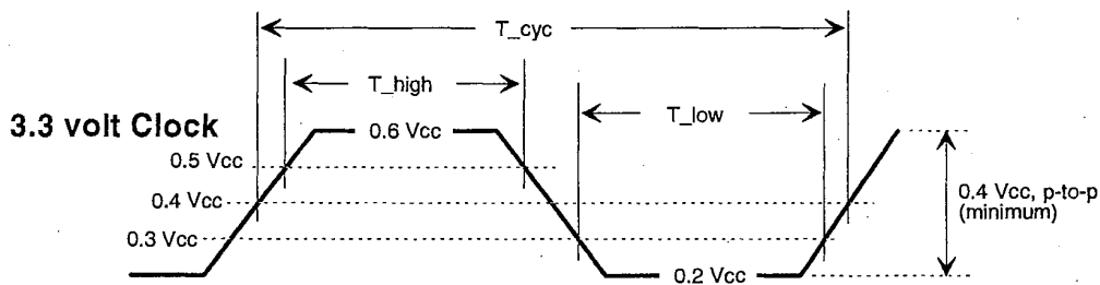
Figure 7-2: 3.3V Clock Waveform
