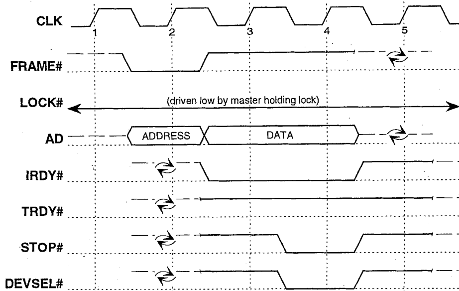
Figure F-3: Accessing a Locked Agent
