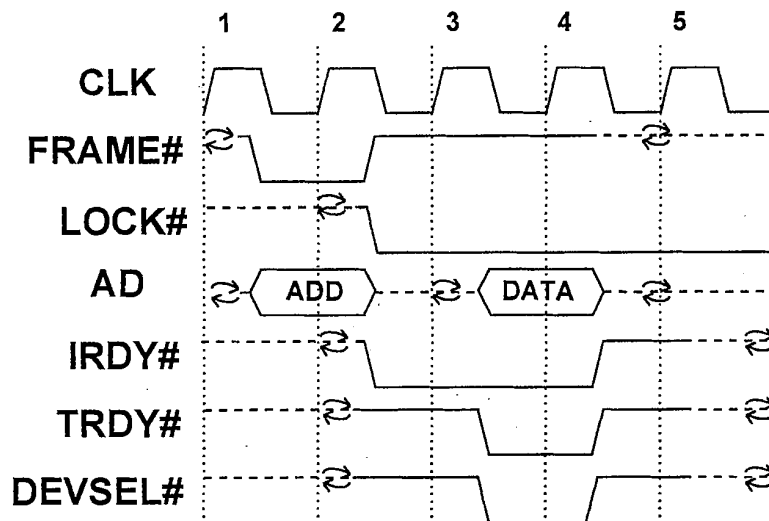
Figure F-1: Starting an Exclusive Access
