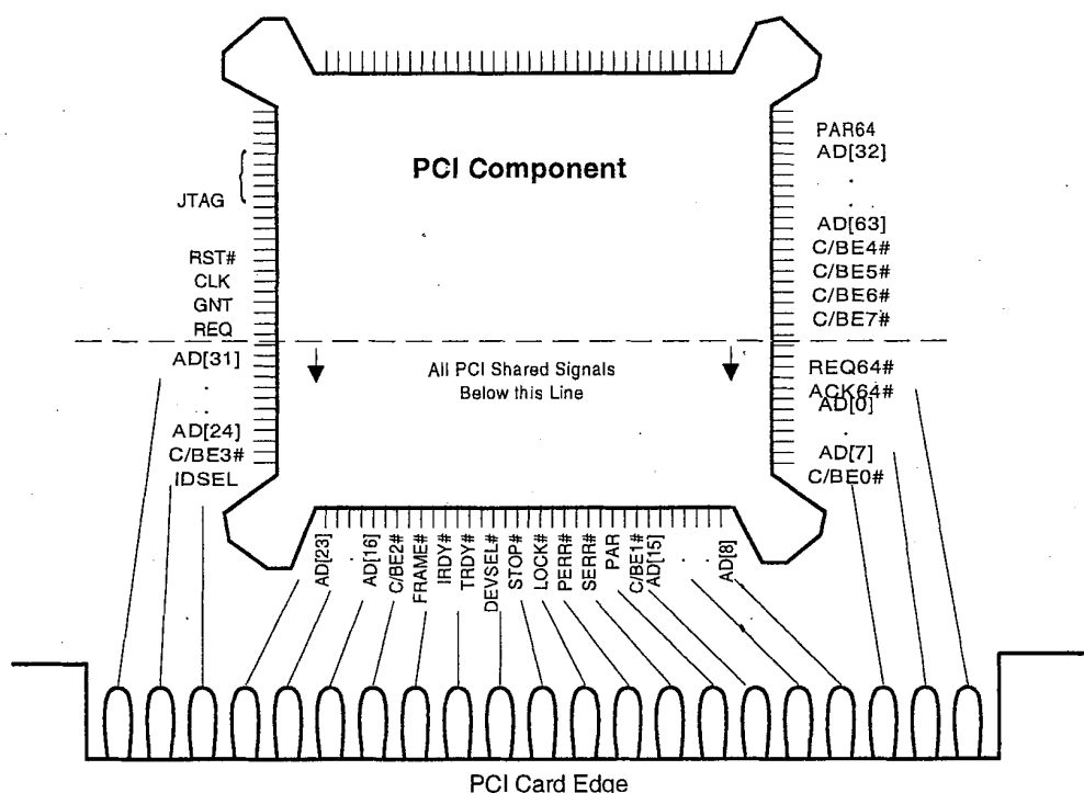
Figure 4-9: Suggested Pinout for PQFP PCI Component
