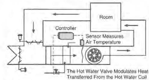
Application 1.2 Heating Control System Schematic
