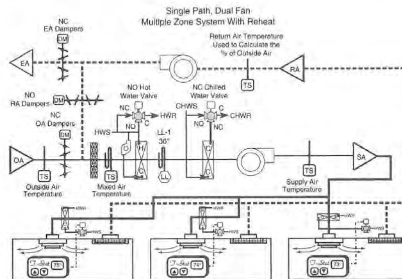
Figure 22.1 Single Path, Multiple Zone AHU with Zone Reheat Coils
