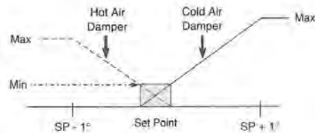
Figure 20.14 Dual Duct VAV Damper Response
