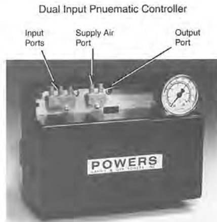
Figure 3.4 Pneumatic Controller
