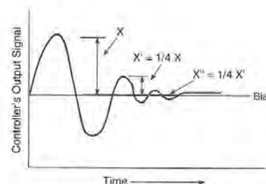
Figure 12.12 Quarter Amplitude Decay Criterion
