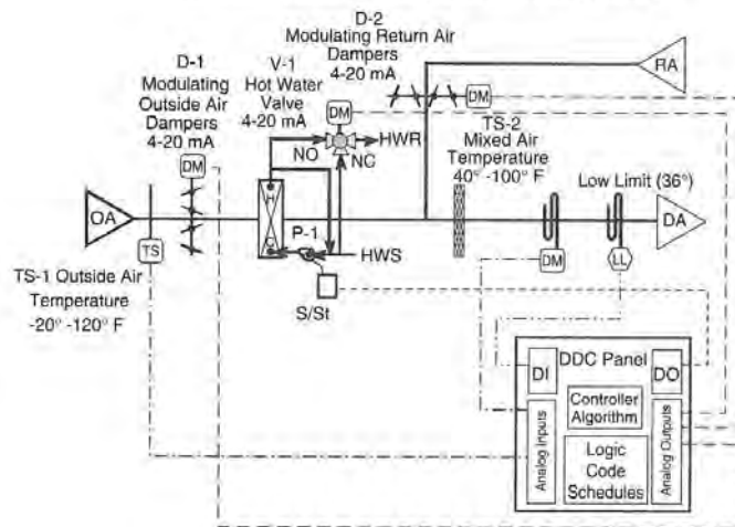
Figure 16.4 Hot Water Coil Preheat Control Strategy
