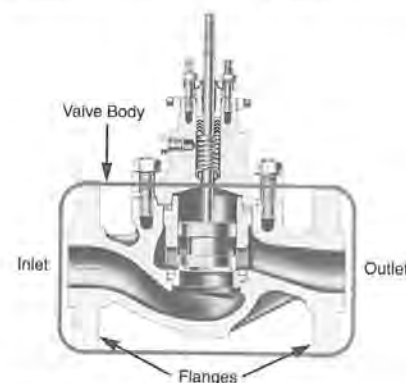
Figure 9.1 Two-Way Valve Body
