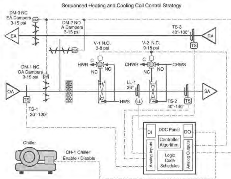
Figure 17.4 Sequenced Hot and Chilled Water Valve Control Strategy
