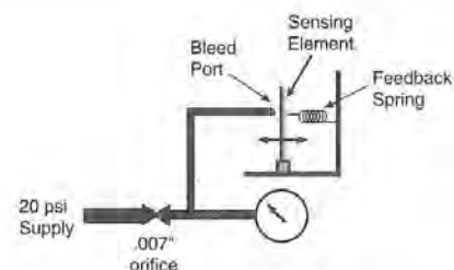
Figure 7.4 Pneumatic Restrictor/Sensor
