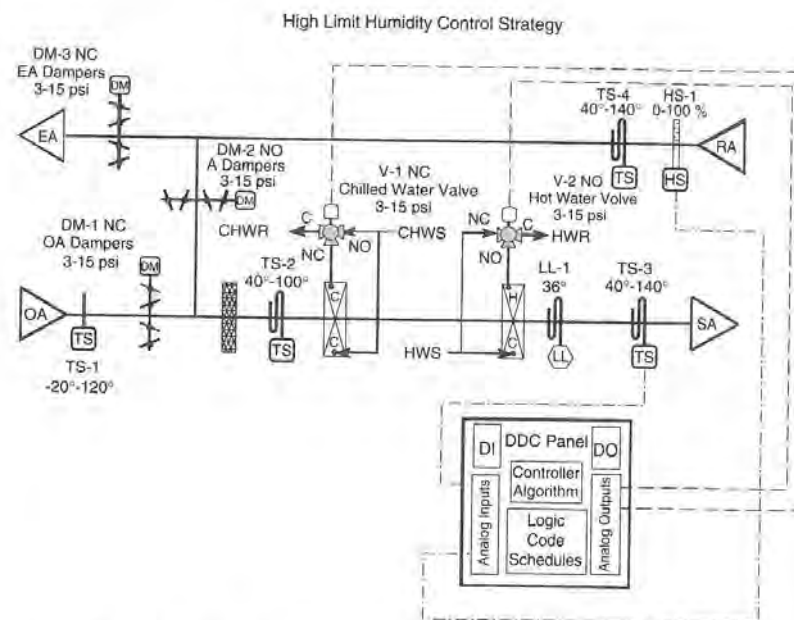
Figure 18.4 Chilled Water Coil Dehumidification With Reheat
