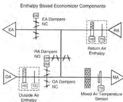
Figure 15.2 Enthalpy Economizer Sensors
