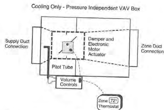
Figure 20.3 Cooling Only VAV Box
