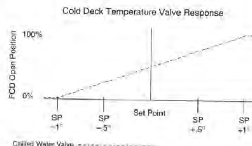
Figure 24.5 Dual Path AHU Cold Deck Valve Response
