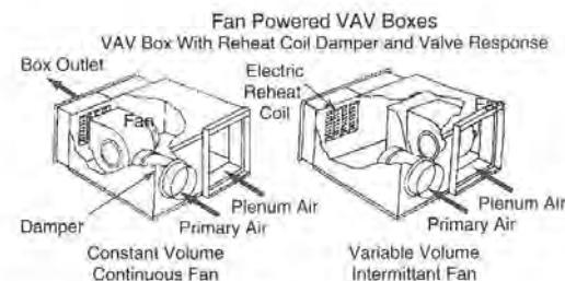
Figure 20.8 Fan Powered VAV Boxes
