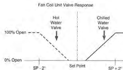
Figure 20.18 Valve Sequence for a Fan Coil Unit
