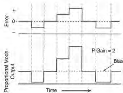
Figure 8.14 Proportional Mode Response to a Step Change in the Error
