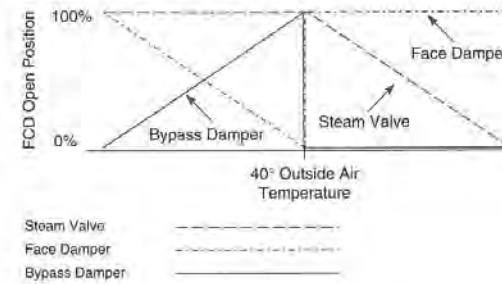
Figure 25.3 Make-Up AHU Valve and Damper Response
