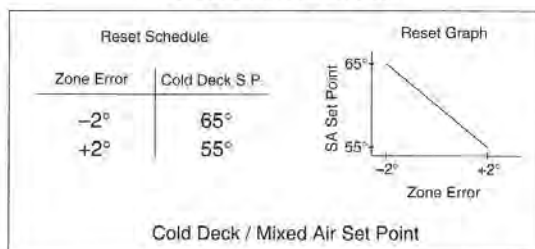
Figure 24.6 Deck Reset Schedules
