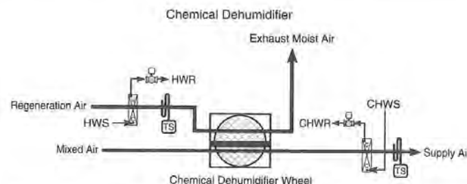
Figure 18.7 Desiccant Dehumidification Configuration
