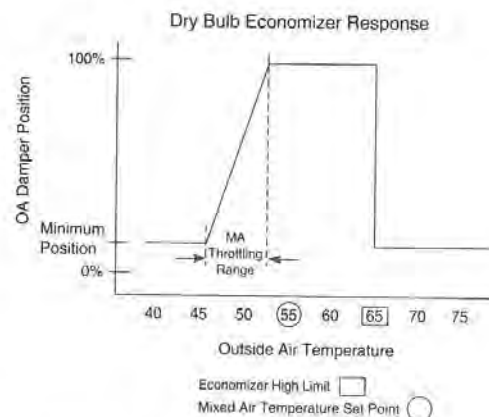
Figure 15.3 Dry Bulb Economizer Response
