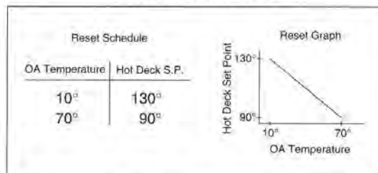
Hot Deck Reset Schedule
