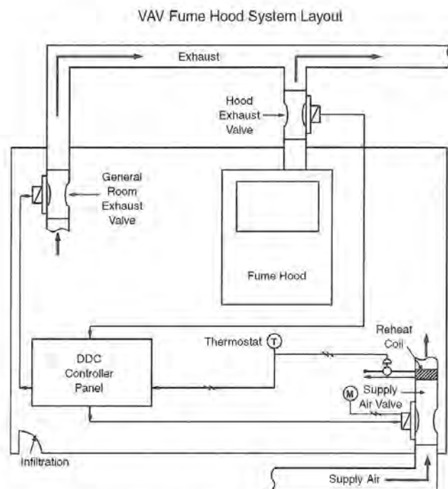
Figure 27.3 Laboratory Fume Hood Layout
