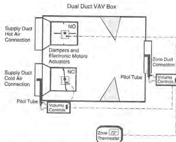
Figure 20.13 Dual Duct VAV Box
