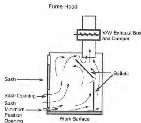
Figure 27.1 Components of a Laboratory Fume Hood
