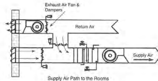
Figure 2.6 Supply Air Path
