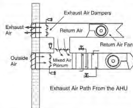
Figure 2.5 Exhaust Airstream
