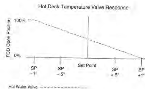
Figure 24.4 Heating Valve Response
