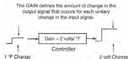
Figure 5.1 The Response of the Proportional Gain Element of a Transfer Function
