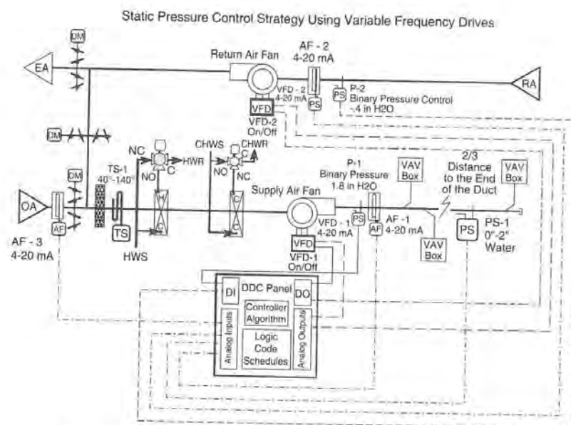
Figure 19.7 Supply and Return Air Static Pressure Control
