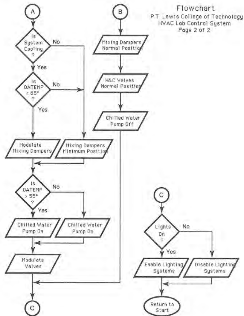
Figure 14.8 Flow Chart
