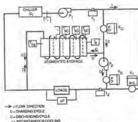
Figure 12.17 Segmented chilled water storage. (Courtesy of McGraw-Hill, Handbook of HVAC Design Fig. 62.57.)
