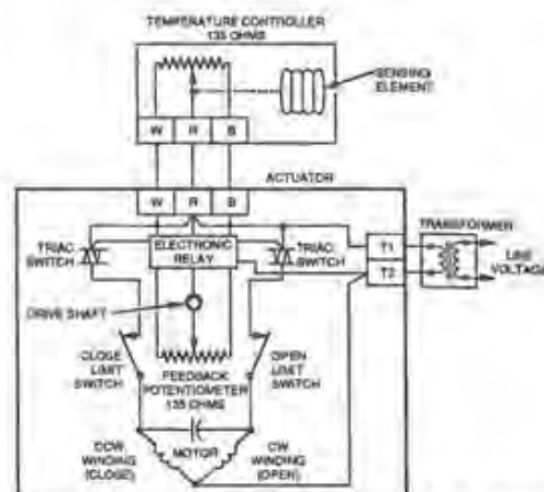
Figure 8.2 Series "90" systems. (Courtesy of Honeywell Inc.)
