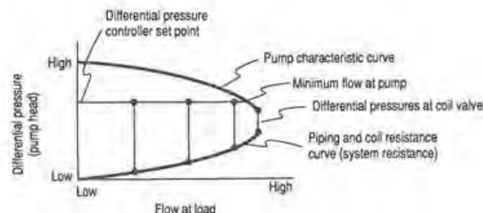
Figure 14.12 Bypass pressure differential control at pump.
