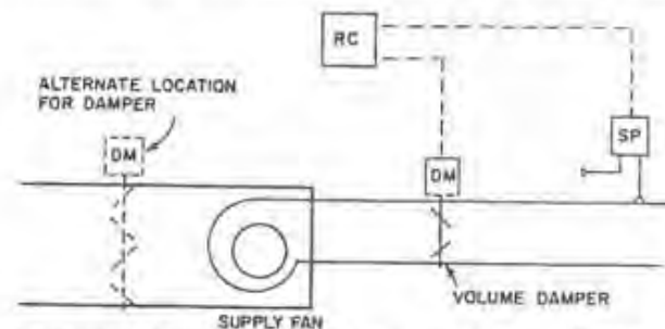
Figure 10.21 Fan volume control—volume damper. (Courtesy of ASHRAE.)
