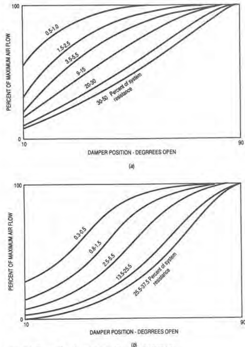
Figure 3.4 Damper flow characteristics. (Courtesy of ASHRAE.)
