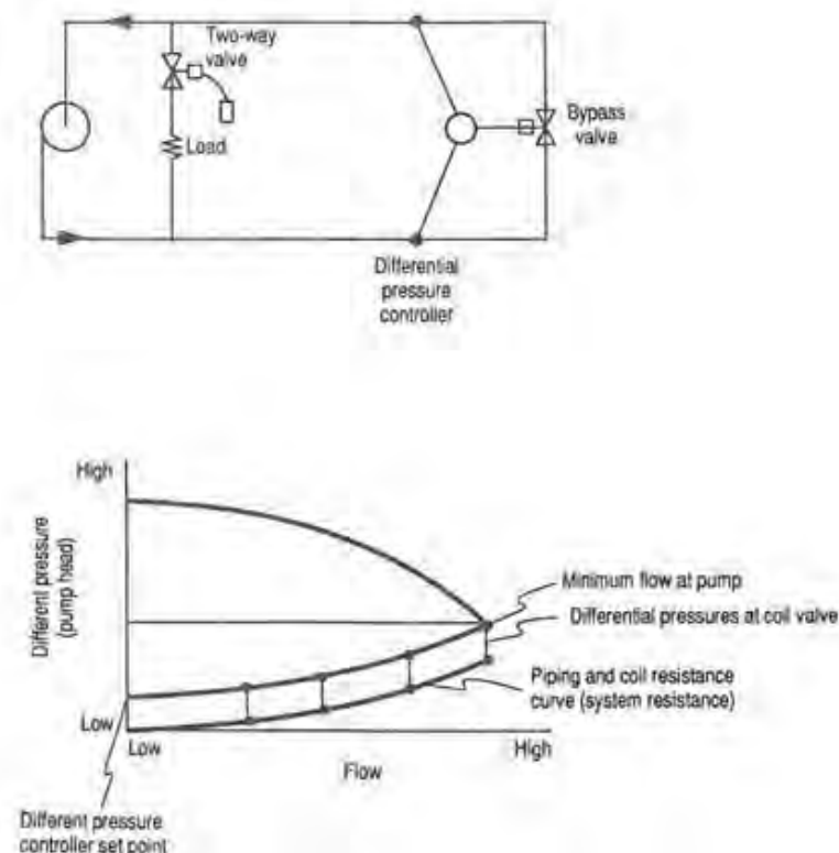
Figure 14.13 Bypass valve and control at the far end of the system.
