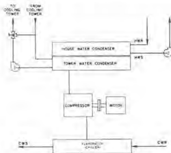
Figure 13.11 Double-bundle condenser in a heat recovery system. (Courtesy of ASHRAE.)
