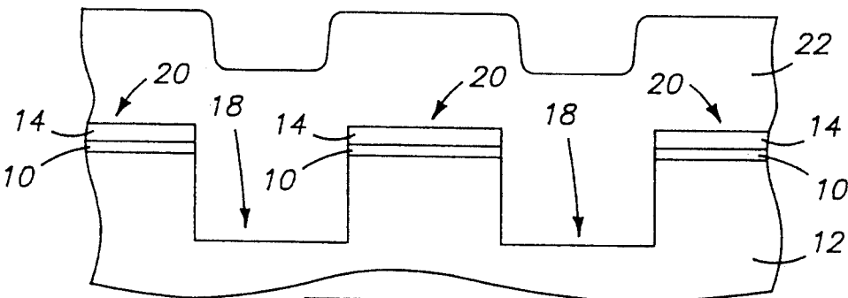
Fig. 3 PRIOR ART
