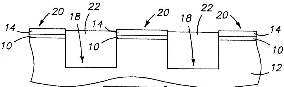
Fig. 4 PRIOR ART
