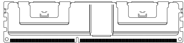
Figure 1: 240-Pin LRDIMM (MO-269 RC/C)
