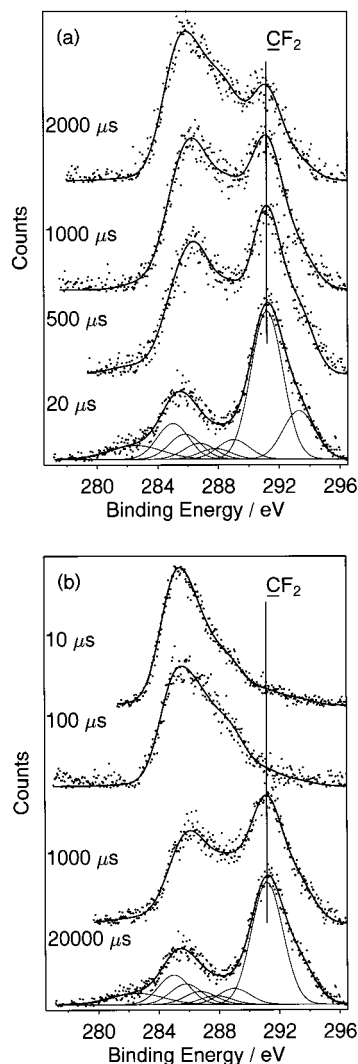
Figure 2. C(1s) XPS spectra of plasma polymerization of 1 H ,1 H ,2 H ,2 H -heptadecafluorodecyl acrylate deposited onto glass with varying (a) t_{\text{on}} ( t_{\text{off}} = 20\,000\ \mu\text{s} , P_p = 40\ \text{W} ) and (b) t_{\text{off}} ( t_{\text{on}} = 20\ \mu\text{s} , P_p = 40\ \text{W} ).
