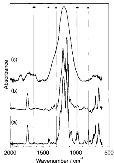
Figure 4. Comparison of infrared spectra: (a) 1 H ,1 H ,2 H ,2 H -heptadecafluorodecyl acrylate monomer; (b) pulsed plasma polymerization conditions ( t_{\text{on}} = 20\ \mu\text{s} , t_{\text{off}} = 20\,000\ \mu\text{s} , P_p = 40\ \text{W} ); and (c) 5 W continuous wave plasma polymerization. NB: * denotes acrylate carbon–carbon double bond absorption bands.
