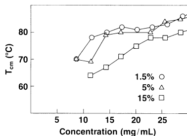
Fig. 7. Effect of PG (%) as added cosolvent on the critical melting temperature ( T_{cm} ) of nafarelin liquid crystals.
