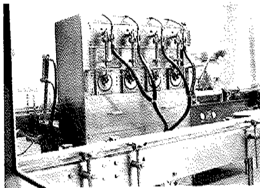
Fig 84-19. Four-pump liquid filler, with a conveyor line for vials protected by a vertical laminar airflow and plastic curtain; note the automatic stoppering machine on the right within the curtain (courtesy, Abbott).
