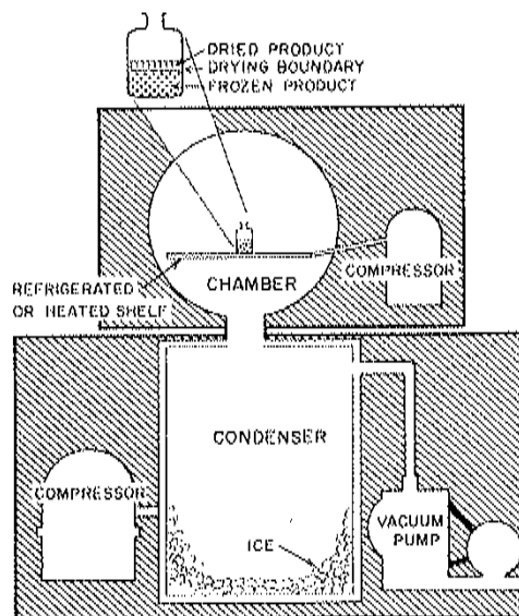
Fig 84-26. Essential components of a freeze-drying system.
