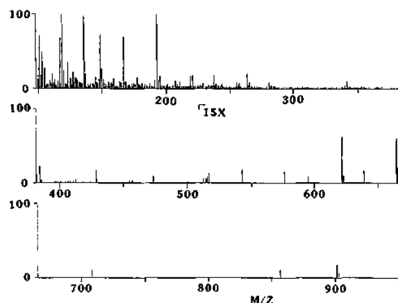
Figure 17—This is the mass spectrum of the particulate matter.
