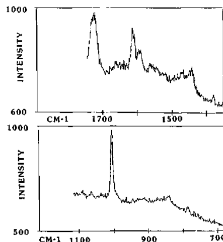
Figure 16—This is the Raman spectrum of a single particle.
