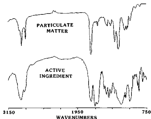
Figure 15—These are the infrared spectra of particulate matter and the active ingredient.
