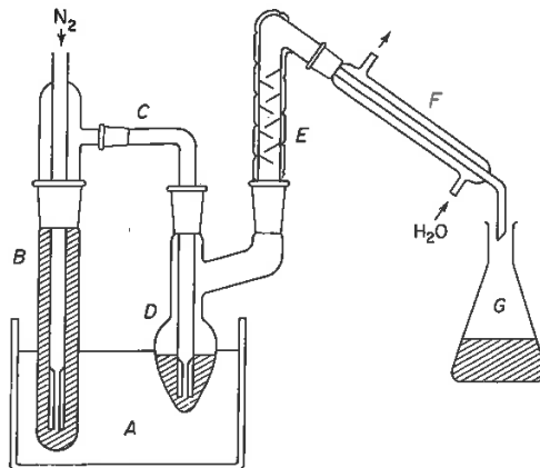
Fig. 1. Apparatus for Hydroxypropoxy Determination.
