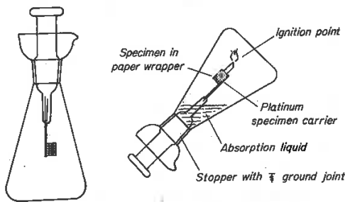
Apparatus for Oxygen Flask Combustion
