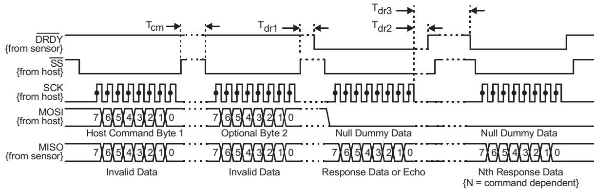
Figure 4-3 SPI Slave-Only Mode Timing
