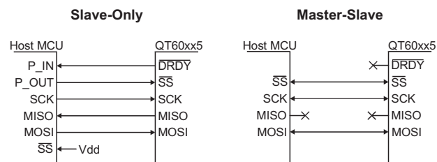
Figure 4-2 SPI Connections
