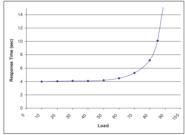
Figure 2: Response time VS Applied Load on a system dimension
