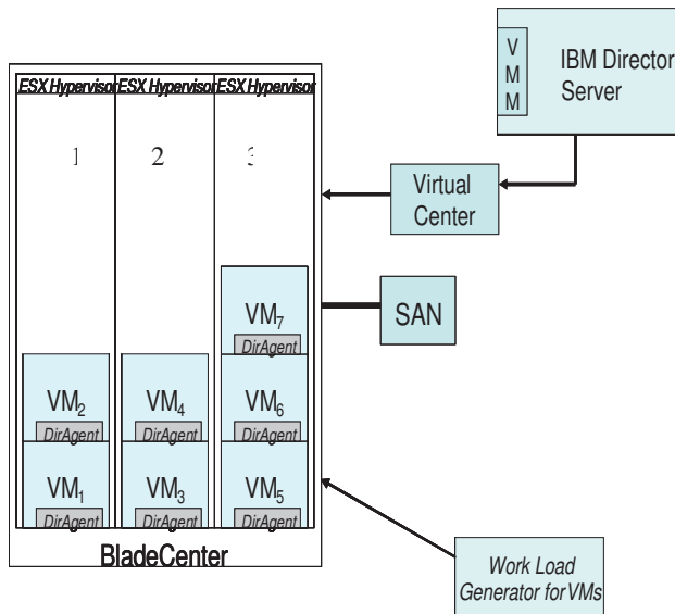
Figure 4: Test-Bed Logical Topology
