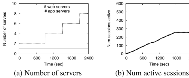
Figure 6. Rubbos: Provision only the Tomcat tier
